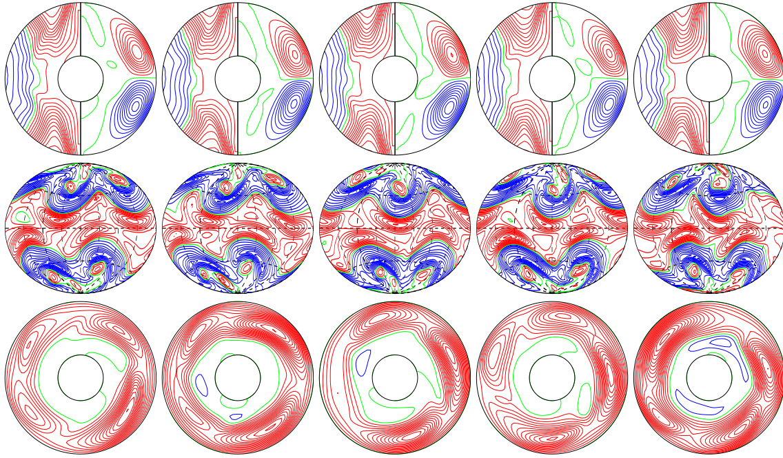
a.e03p1t03r-50000m1n2Nz2.0e5a E_{\text{kin}}
