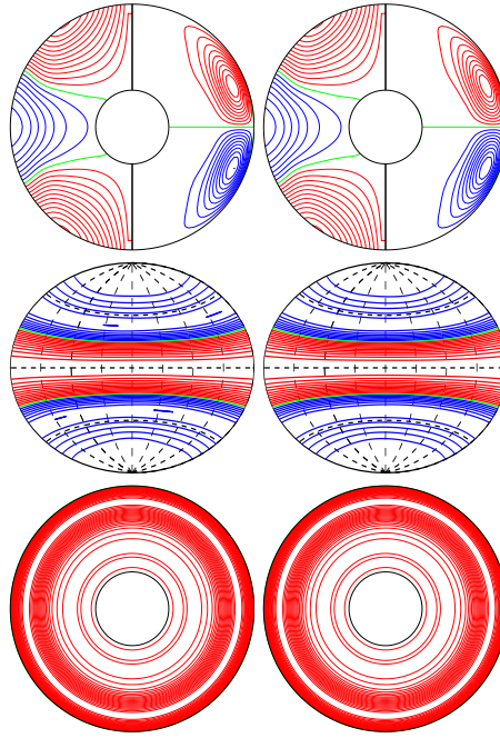
a.e03p1t03r-50000m1n2N2z1.05e5a E_{\text{kin}}
