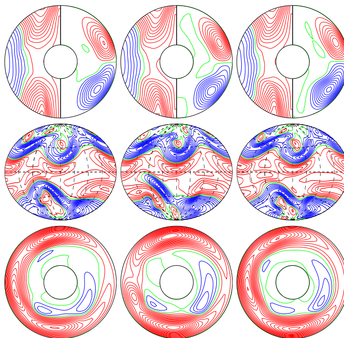
a.e03p1t03r-50000m1n2N2z1.4e5a E_{\text{kin}}
