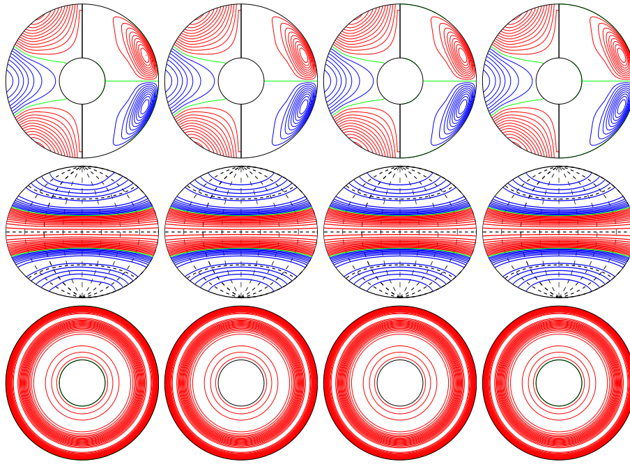
a.e03p1t03r-50000m1n2N2z1.0e5a E_{\text{kin}}
