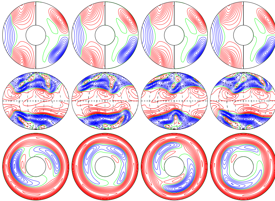
a.e03p1t03r-50000m1n2N2z1.2e5a E_{\text{kin}}
