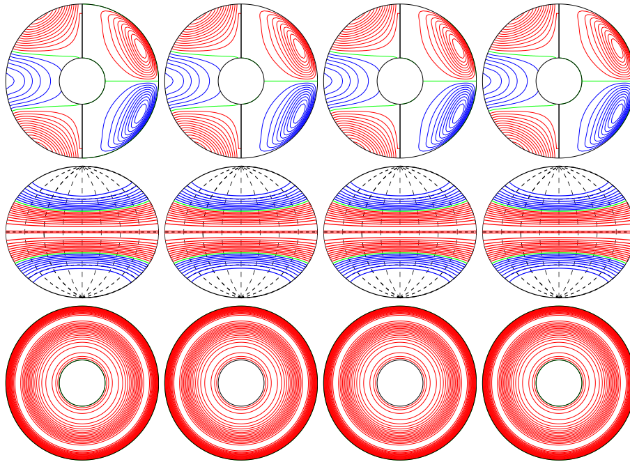
a.e03p1t03r-50000m1n2N2z0.4e5a E_{\text{kin}}
