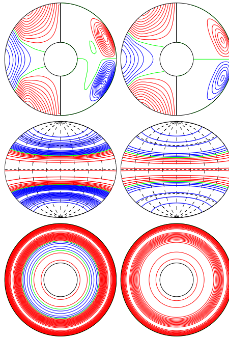
a.e03p1t03r-50000m1n2N2z1.1e5a E_{\text{kin}}
