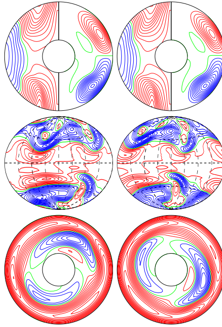
a.e03p1t03r-50000m1n2N2z1.3e5a E_{\text{kin}}
