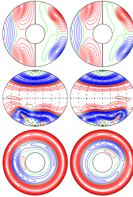
a.e03p1t03r-50000m1n2N2z1.15e5a E_{\text{kin}}
