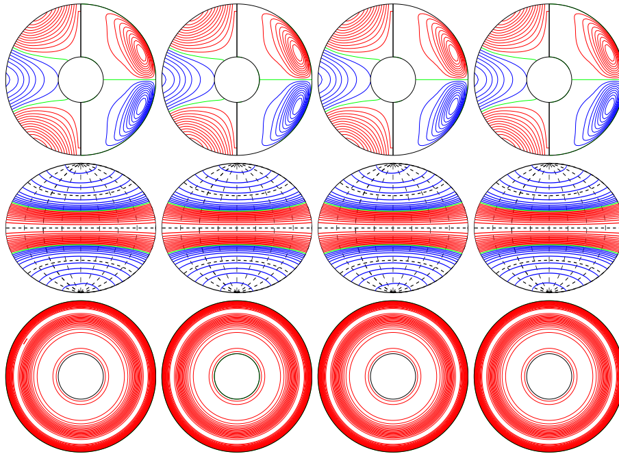
a.e03p1t03r-50000m1n2N2z0.8e5a E_{\text{kin}}
