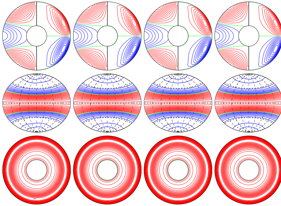
a.e03p1t03r-50000m1n2N2z0.6e5a E_{\text{kin}}
