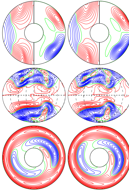
a.e03p1t03r-50000m1n2N2z1.25e5a E_{\text{kin}}
