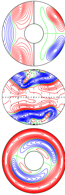
a.e03p1t03r-50000m1n2N2z1.18e5a E_{\text{kin}}
