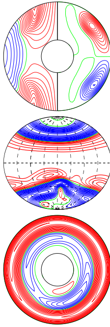
a.e03p1t03r-50000m1n2N2z1.14e5a E_{\text{kin}}
