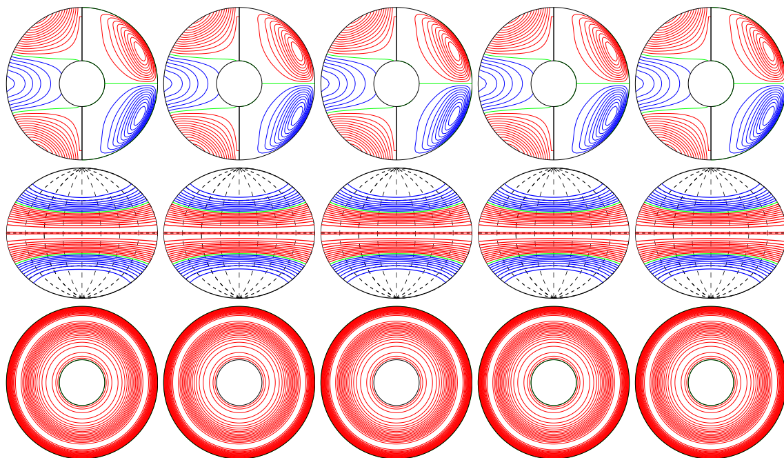
a.e03p1t03r-50000m1n2N2z0.4e5a E_{\text{kin}}
