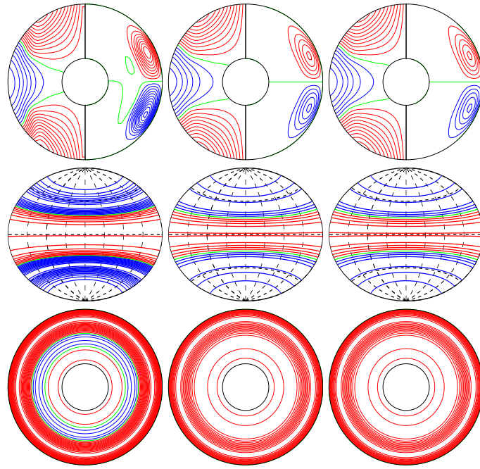
a.e03p1t03r-50000m1n2N2z1.1e5a E_{\text{kin}}
