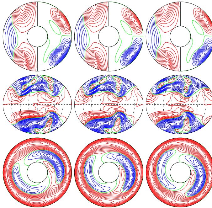
a.e03p1t03r-50000m1n2N2z1.25e5a E_{\text{kin}}
