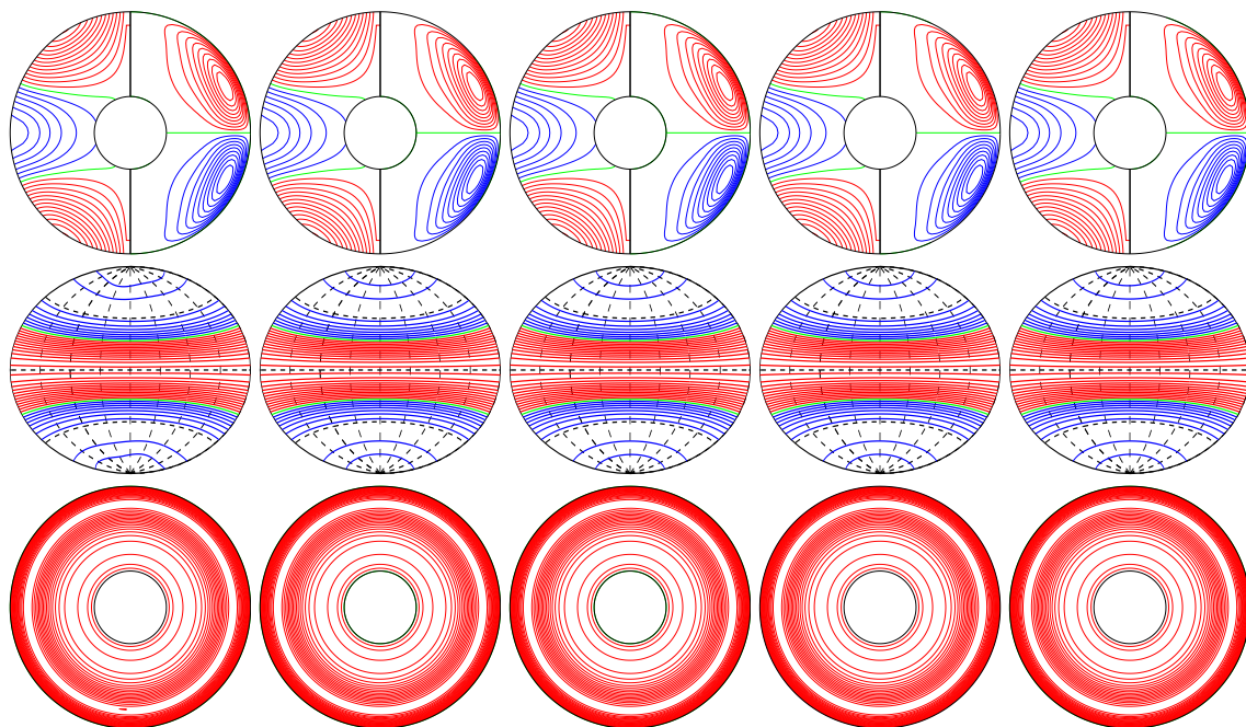
a.e03p1t03r-50000m1n2N2z0.6e5a E_{\text{kin}}
