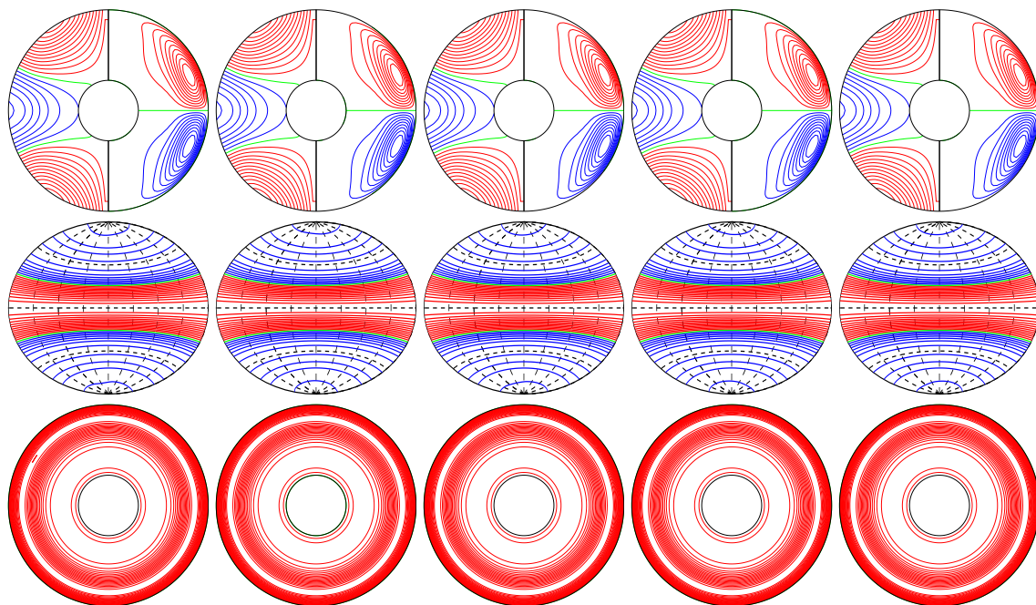
a.e03p1t03r-50000m1n2N2z0.8e5a E_{\text{kin}}
