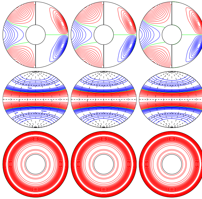
a.e03p1t03r-50000m1n2N2z1.05e5a E_{\text{kin}}
