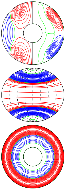
a.e03p1t03r-50000m1n2N2z1.13e5a E_{\text{kin}}
