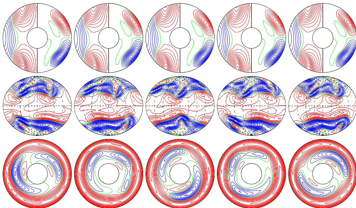
a.e03p1t03r-50000m1n2N2z1.2e5a E_{\text{kin}}
