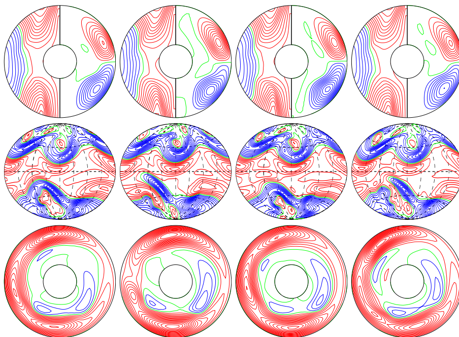
a.e03p1t03r-50000m1n2N2z1.4e5a E_{\text{kin}}
