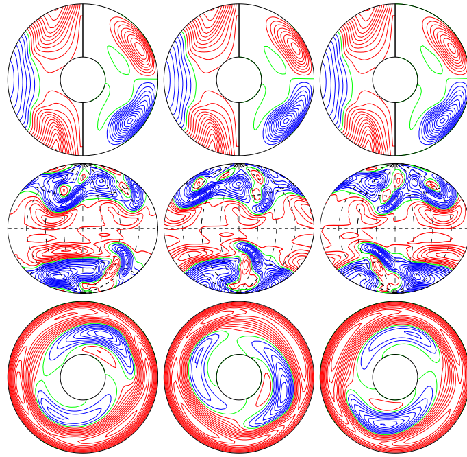
a.e03p1t03r-50000m1n2N2z1.3e5a E_{\text{kin}}
