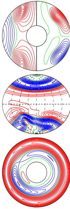
a.e03p1t03r-50000m1n2N2z1.16e5a E_{\text{kin}}
