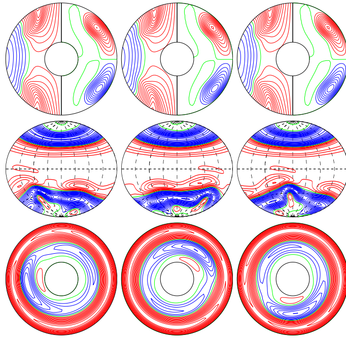
a.e03p1t03r-50000m1n2N2z1.15e5a E_{\text{kin}}
