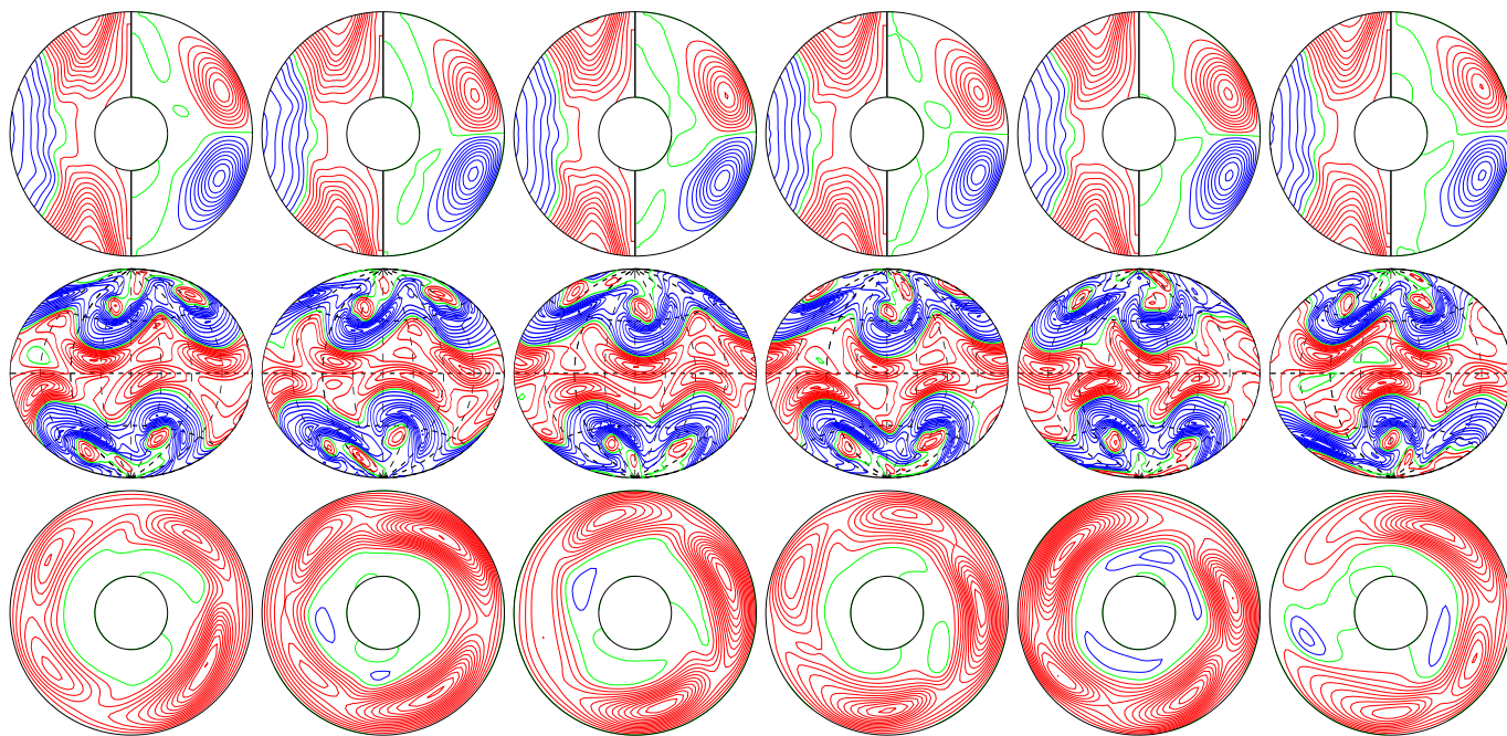
a.e03p1t03r-50000m1n2Nz2.0e5a E_{\text{kin}}
