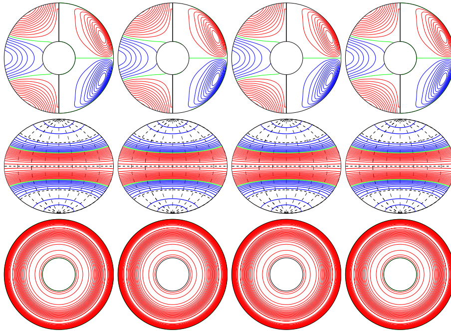
a.e03p1t03r-50000m1n2N2z0.6e5ac E_{\text{kin}}
