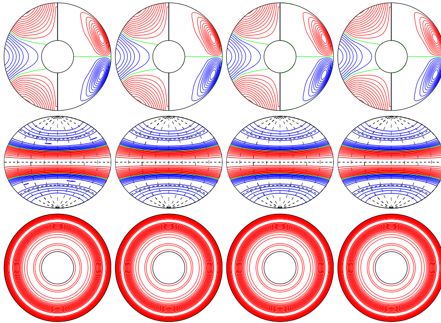
a.e03p1t03r-50000m1n2N2z1.05e5a E_{\text{kin}}
