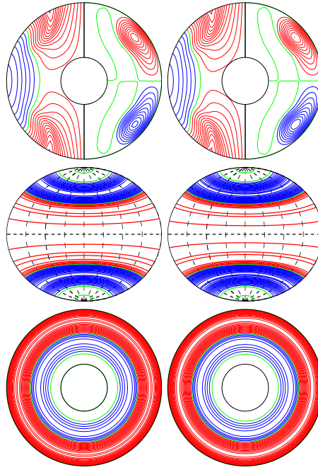
a.e03p1t03r-50000m1n2N2z1.13e5a E_{\text{kin}}
