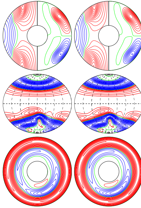
a.e03p1t03r-50000m1n2N2z1.14e5a E_{\text{kin}}
