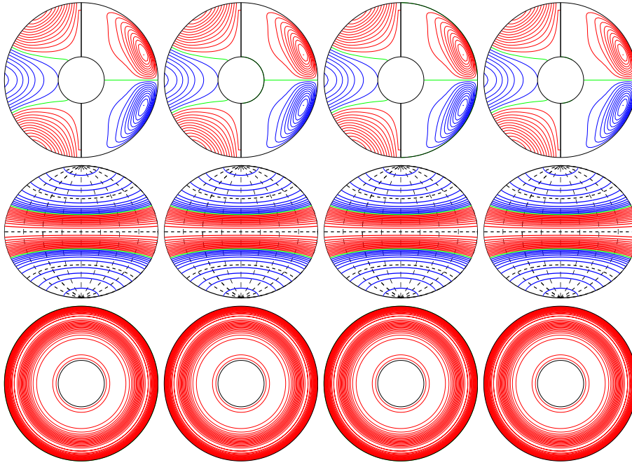
a.e03p1t03r-50000m1n2N2z0.8e5ac E_{\text{kin}}
