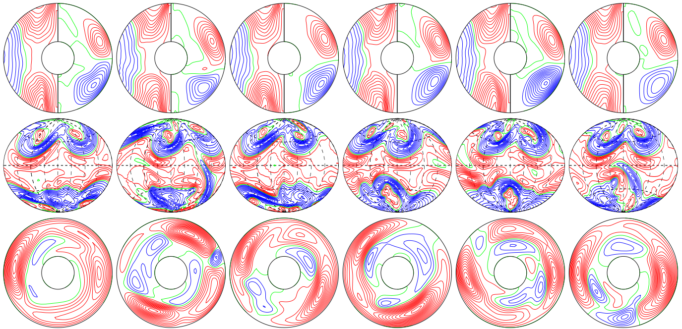
a.e03p1t03r-50000m1n2N2z1.8e5a E_{\text{kin}}
