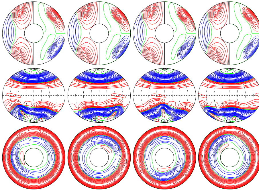
a.e03p1t03r-50000m1n2N2z1.15e5a E_{\text{kin}}
