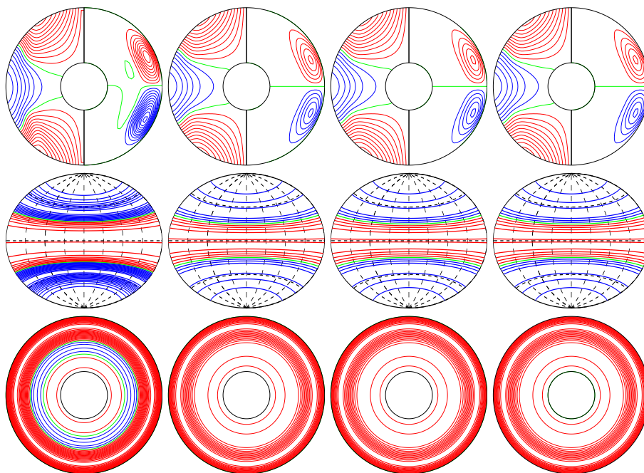
a.e03p1t03r-50000m1n2N2z1.1e5a E_{\text{kin}}
