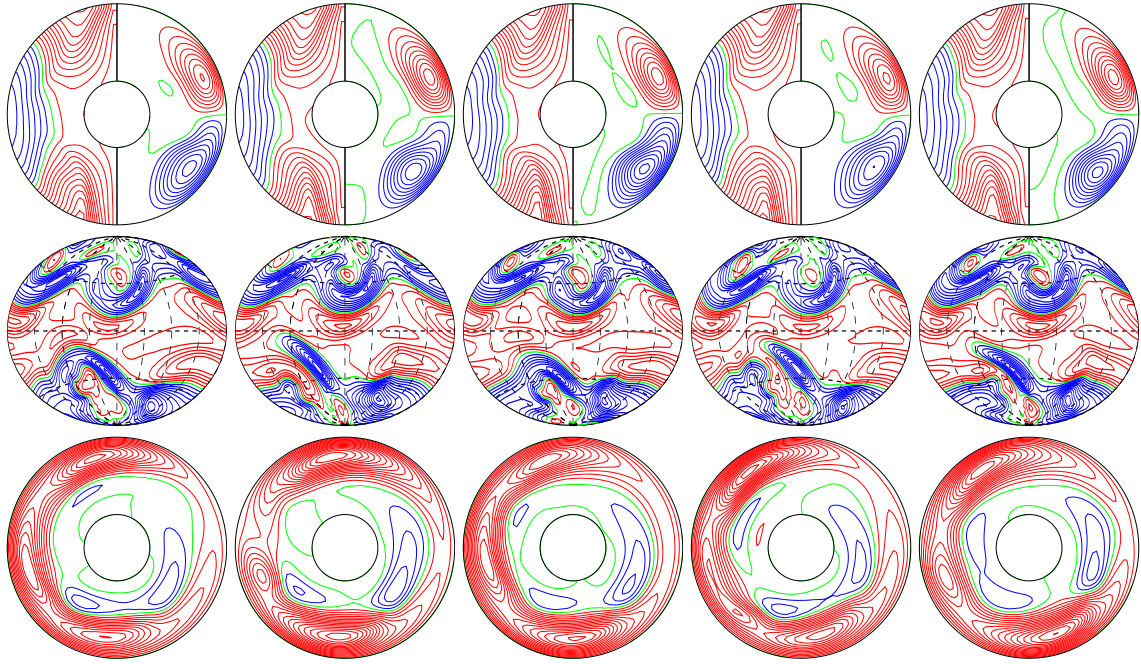
a.e03p1t03r-50000m1n2N2z1.4e5a E_{\text{kin}}
