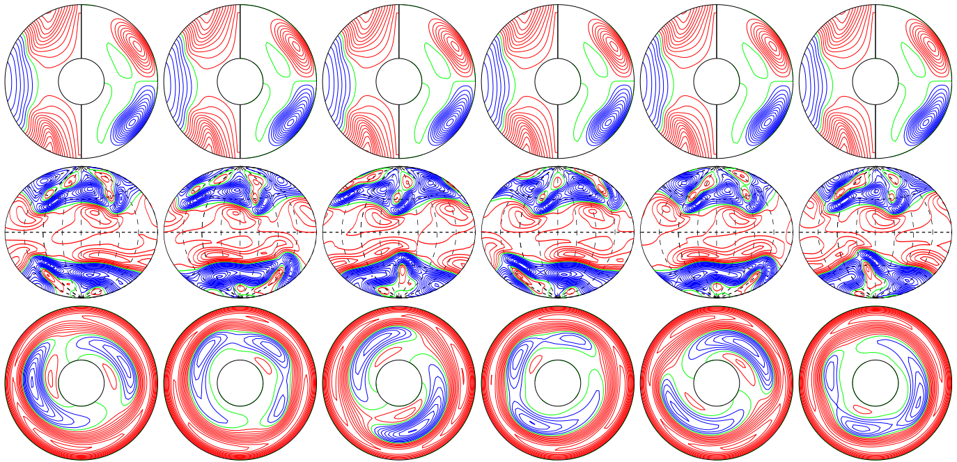
a.e03p1t03r-50000m1n2N2z1.2e5a E_{\text{kin}}
