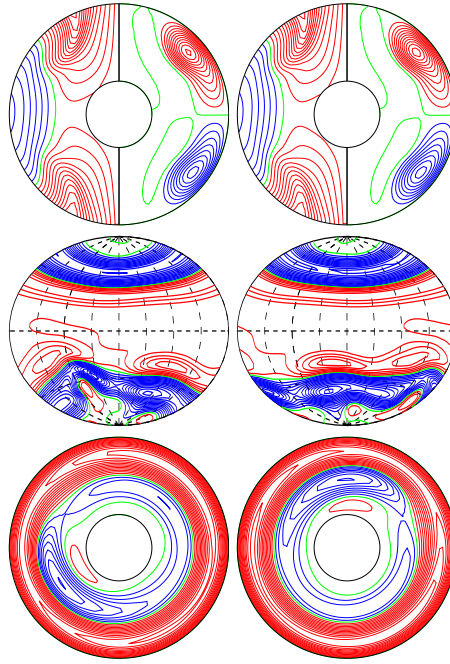
a.e03p1t03r-50000m1n2N2z1.16e5a E_{\text{kin}}
