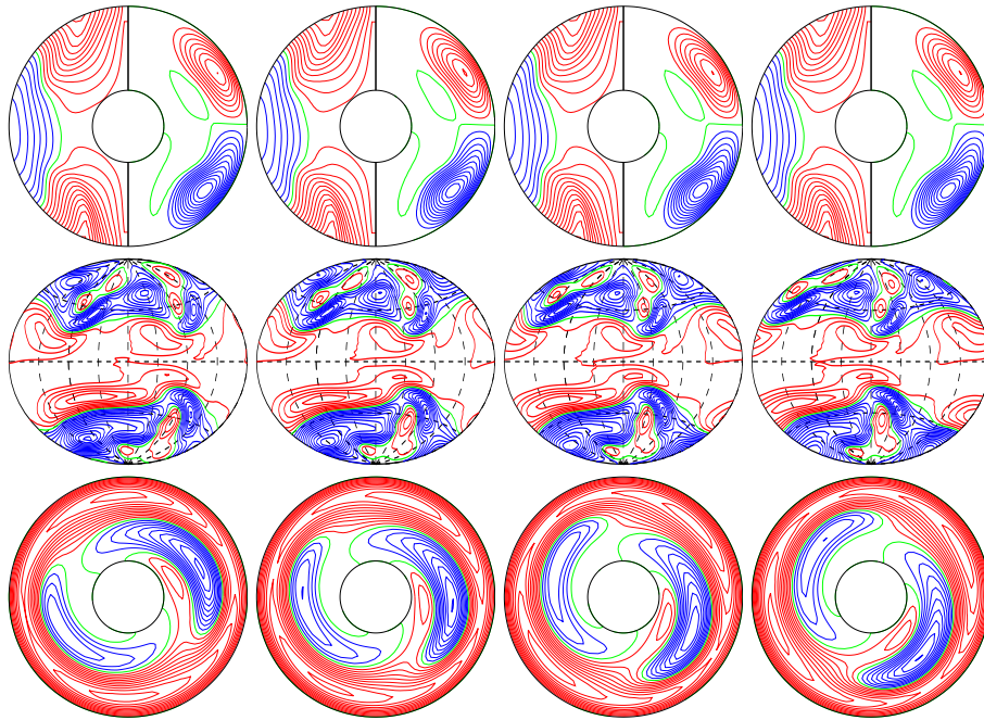
a.e03p1t03r-50000m1n2N2z1.25e5a E_{\text{kin}}
