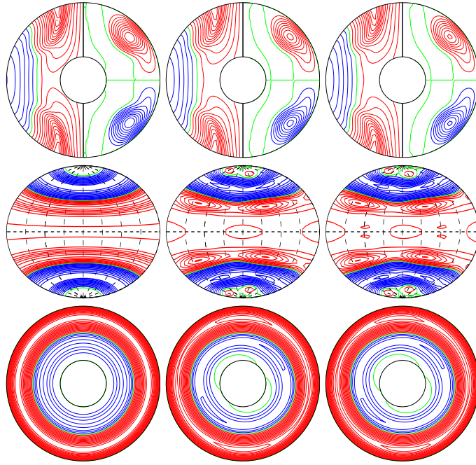
a.e03p1t03r-50000m1n2N2z1.2e5ac E_{\text{kin}}
