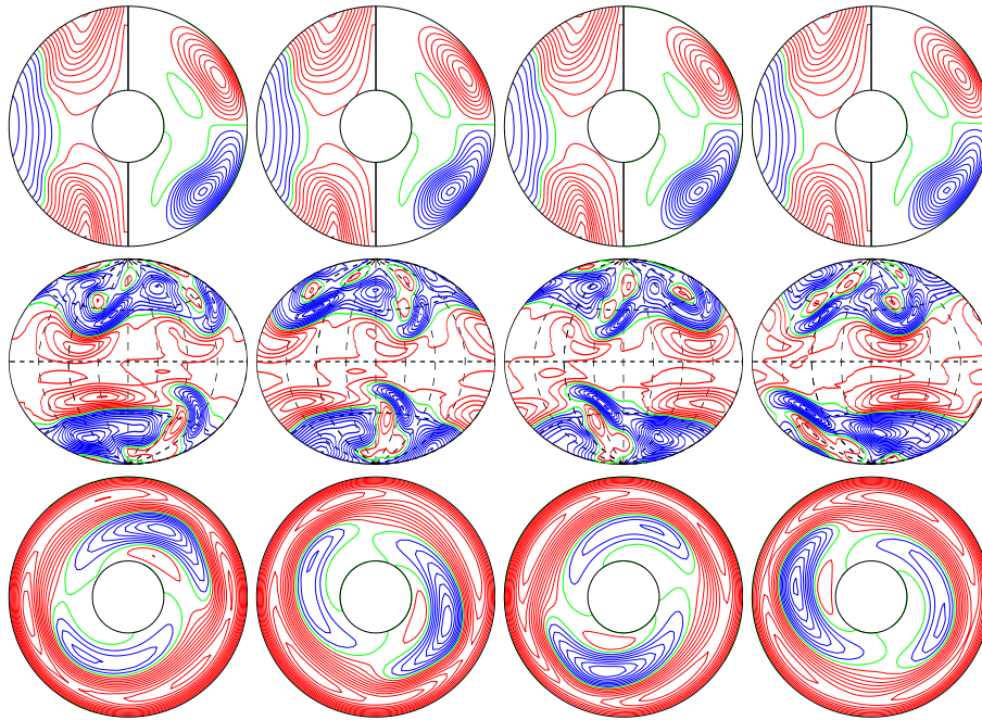
a.e03p1t03r-50000m1n2N2z1.3e5a E_{\text{kin}}
