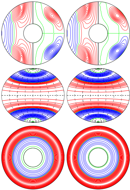
a.e03p1t03r-50000m1n2N2z1.18e5ac E_{\text{kin}}
