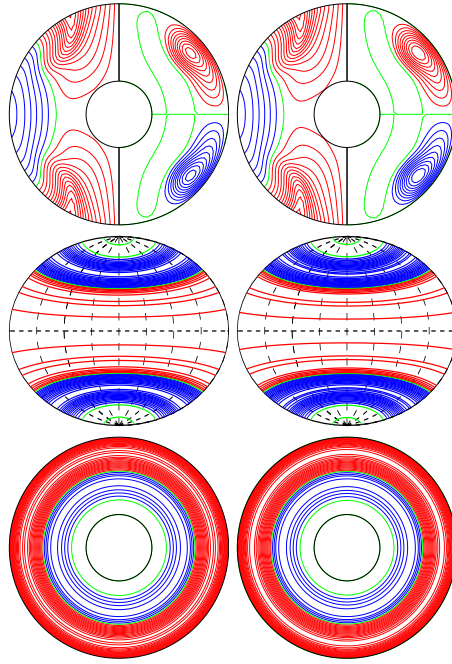
a.e03p1t03r-50000m1n2N2z1.13e5ac E_{\text{kin}}
