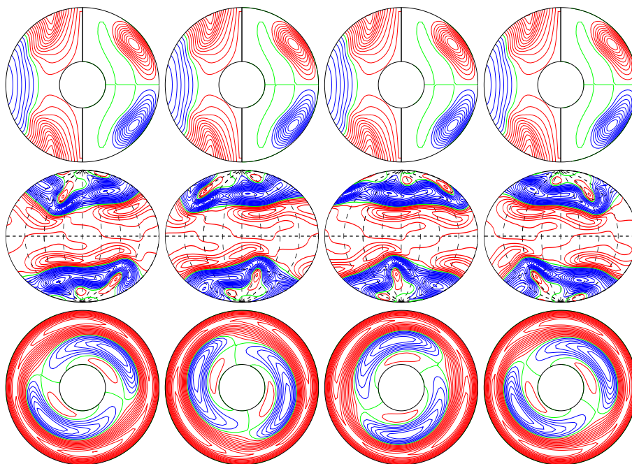
a.e03p1t03r-50000m1n2N2z1.18e5a E_{\text{kin}}
