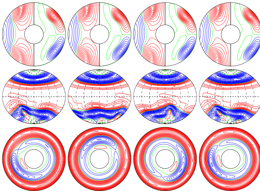
a.e03p1t03r-50000m1n2N2z1.16e5a E_{\text{kin}}
