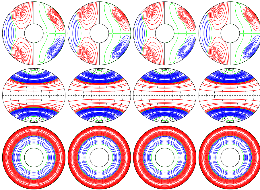
a.e03p1t03r-50000m1n2N2z1.13e5a E_{\text{kin}}
