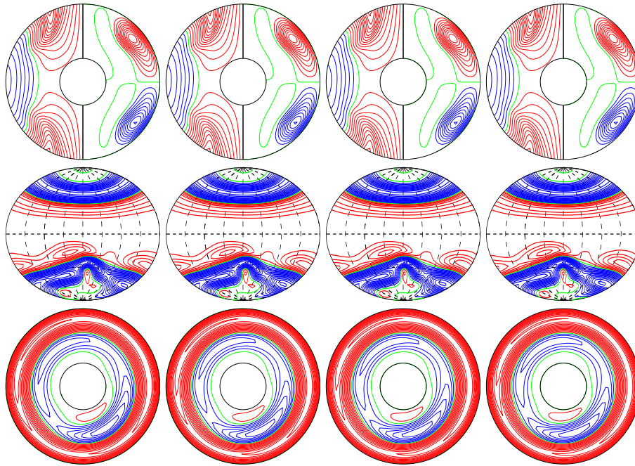
a.e03p1t03r-50000m1n2N2z1.14e5a E_{\text{kin}}
