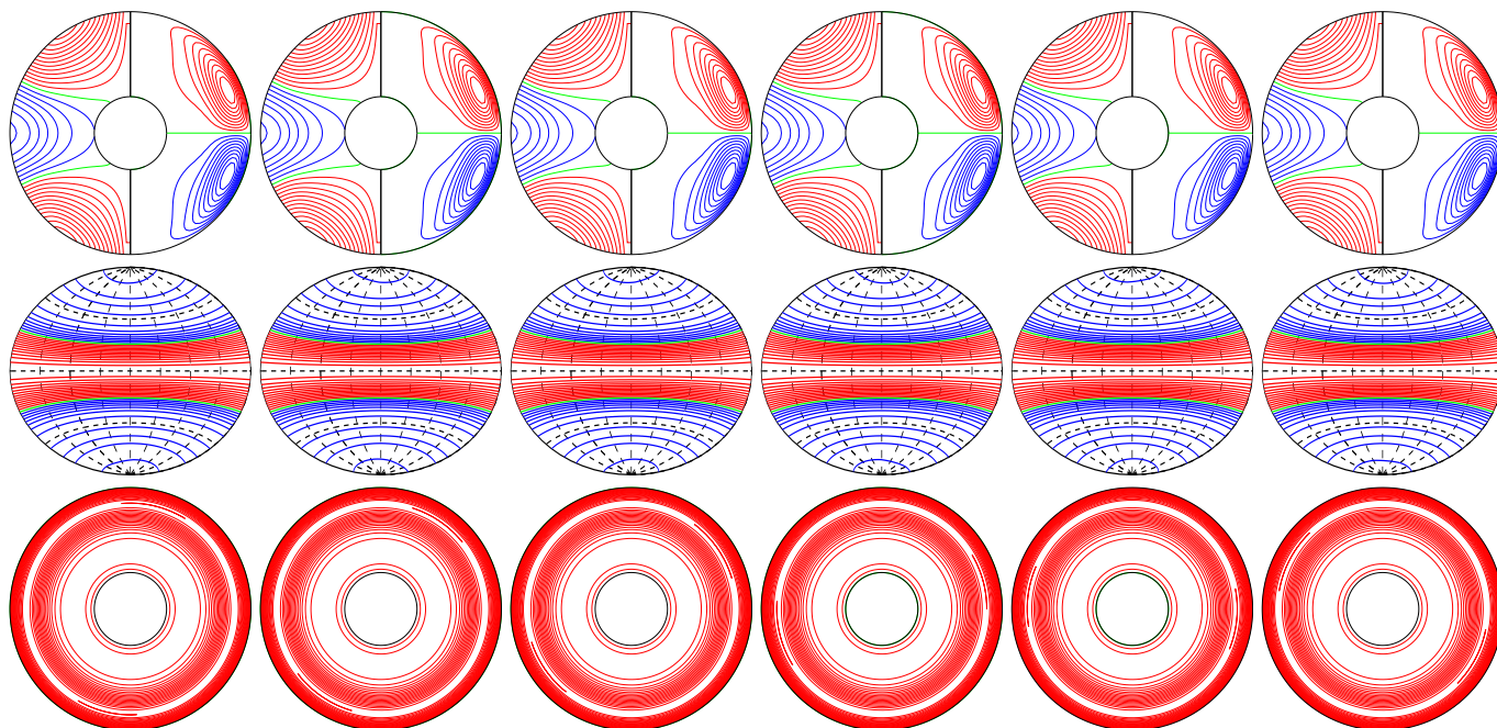
a.e03p1t03r-50000m1n2N2z0.8e5a E_{\text{kin}}
