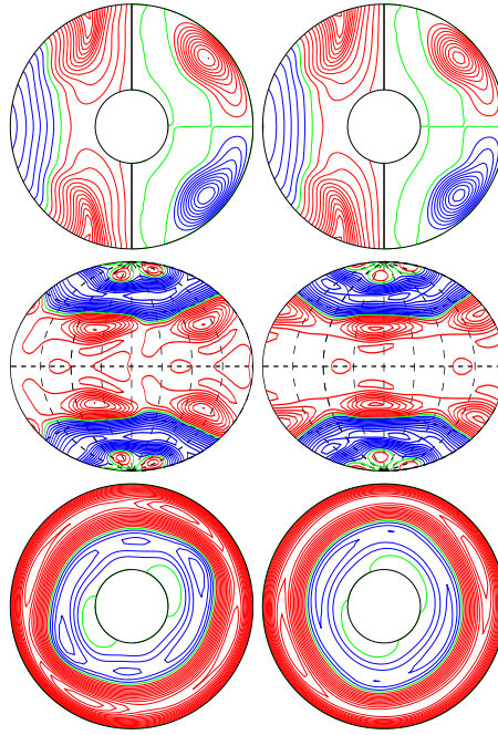
a.e03p1t03r-50000m1n2N2z1.25e5ac E_{\text{kin}}
