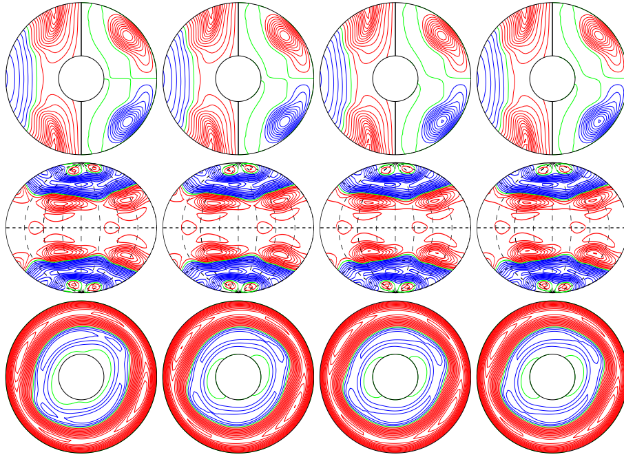
a.e03p1t03r-50000m1n2N2z1.3e5ac E_{\text{kin}}
