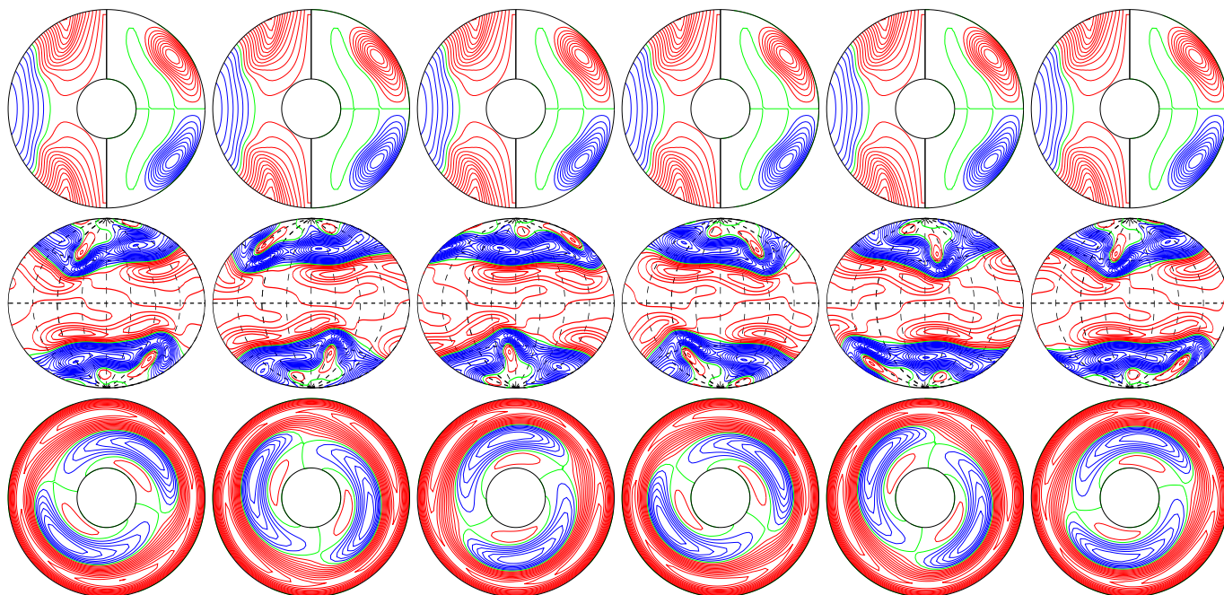
a.e03p1t03r-50000m1n2N2z1.18e5a E_{\text{kin}}
