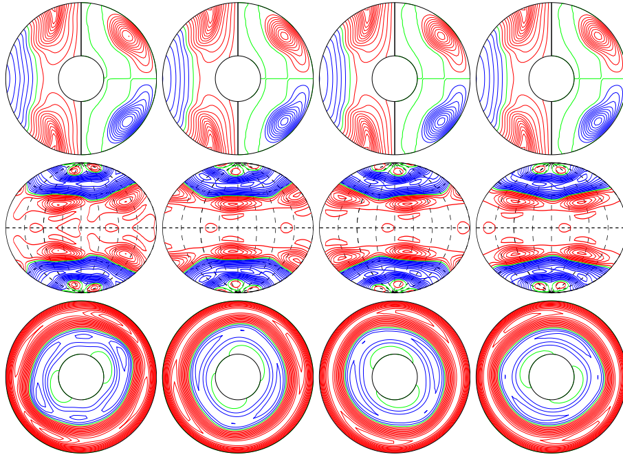
a.e03p1t03r-50000m1n2N2z1.25e5ac E_{\text{kin}}
