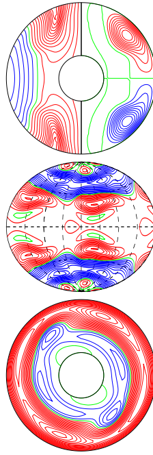
a.e03p1t03r-50000m1n2N2z1.4e5aca E_{\text{kin}}
