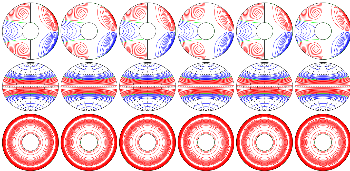
a.e03p1t03r-50000m1n2N2z0.6e5a E_{\text{kin}}
