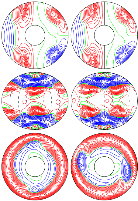
a.e03p1t03r-50000m1n2N2z1.5e5aca E_{\text{kin}}
