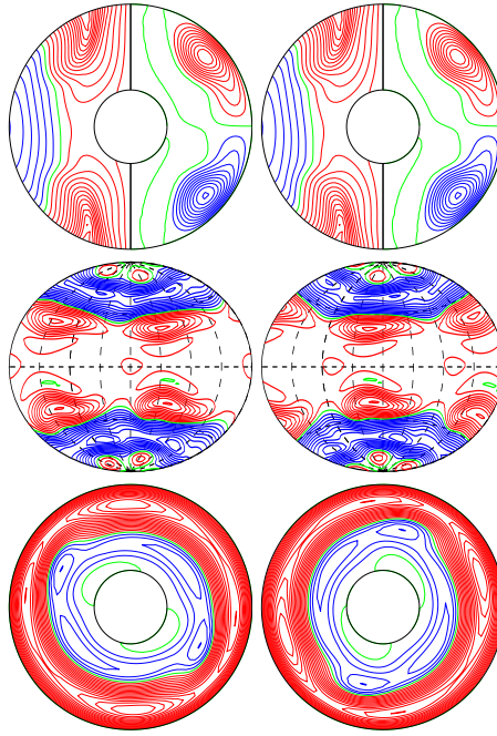
a.e03p1t03r-50000m1n2N2z1.35e5aca E_{\text{kin}}
