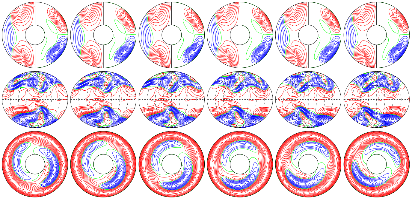
a.e03p1t03r-50000m1n2N2z1.25e5a E_{\text{kin}}
