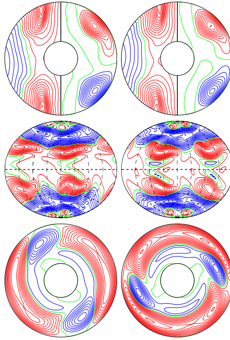
a.e03p1t03r-50000m1n2N2z1.6e5aca E_{\text{kin}}
