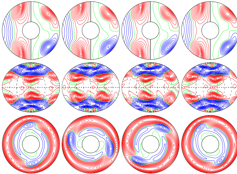
a.e03p1t03r-50000m1n2N2z1.5e5aca E_{\text{kin}}
