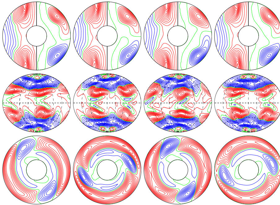
a.e03p1t03r-50000m1n2N2z1.6e5aca E_{\text{kin}}
