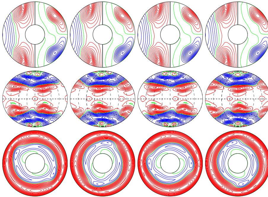
a.e03p1t03r-50000m1n2N2z1.35e5aca E_{\text{kin}}
