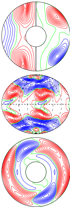
a.e03p1t03r-50000m1n2N2z1.68e5aca E_{\text{kin}}
