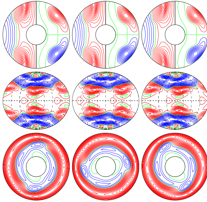
a.e03p1t03r-50000m1n2N2z1.4e5aca E_{\text{kin}}
