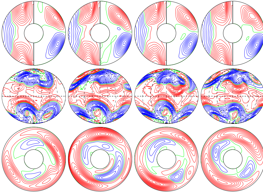
a.e03p1t03r-50000m1n2N2z1.7e5aca E_{\text{kin}}
