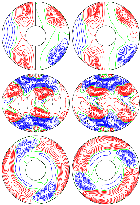
a.e03p1t03r-50000m1n2N2z1.68e5aca E_{\text{kin}}
