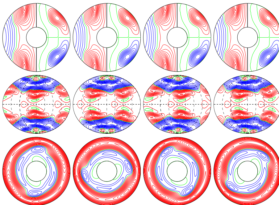
a.e03p1t03r-50000m1n2N2z1.4e5aca E_{\text{kin}}
