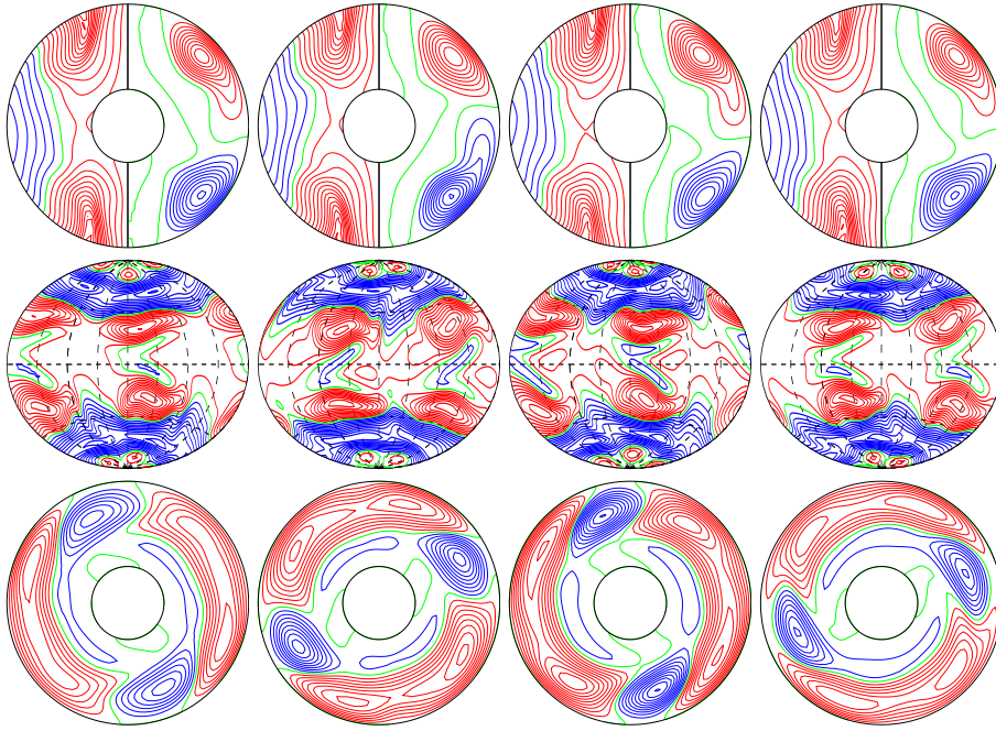
a.e03p1t03r-50000m1n2N2z1.65e5aca E_{\text{kin}}
