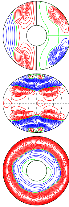
a.e03p1t03r-50000m1n2N2z1.32e5b E_{\text{kin}}
