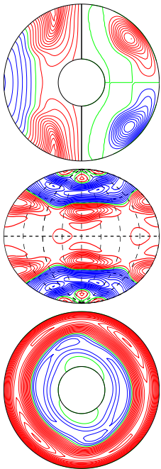
a.e03p1t03r-50000m1n2N2z1.31e5aca E_{\text{kin}}
