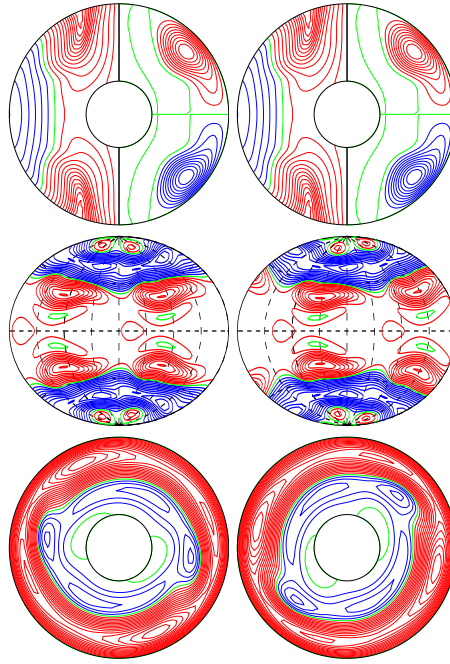
a.e03p1t03r-50000m1n2N2z1.38e5b E_{\text{kin}}
