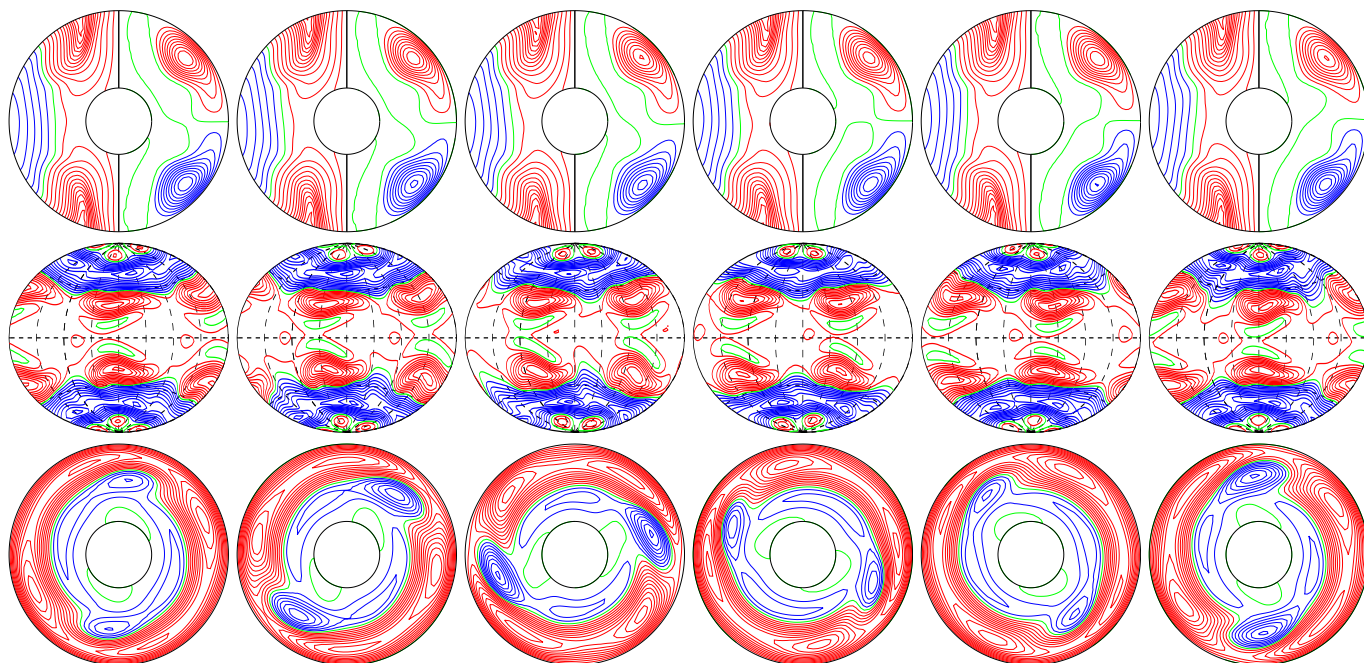
a.e03p1t03r-50000m1n2N2z1.5e5aca E_{\text{kin}}
