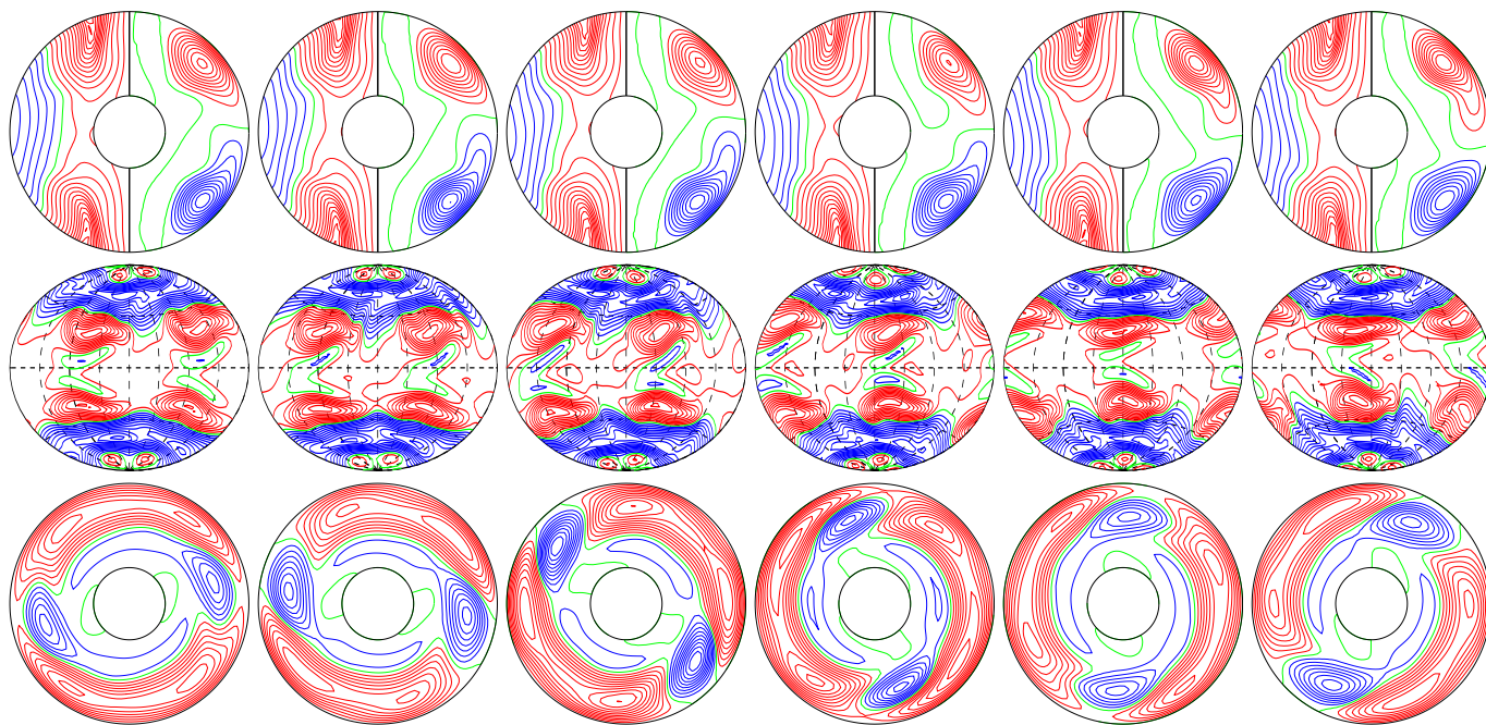
a.e03p1t03r-50000m1n2N2z1.6e5aca E_{\text{kin}}
