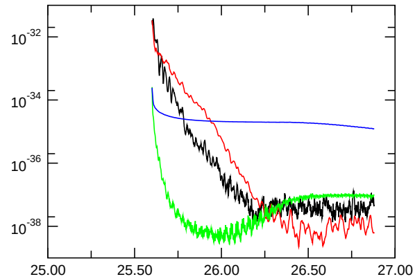
E_{kin,asymm.}
