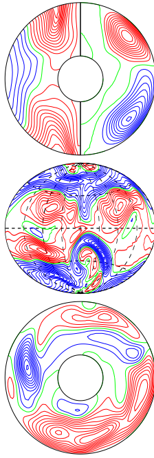
a.e03p1t03r-50000m1n2N2z1.64e5aca E_{\text{kin}}
