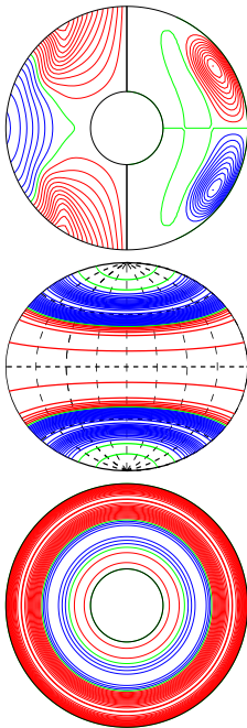
a.e03p1t03r-50000m1n2N2z1.1e5ac E_{\text{kin}}
