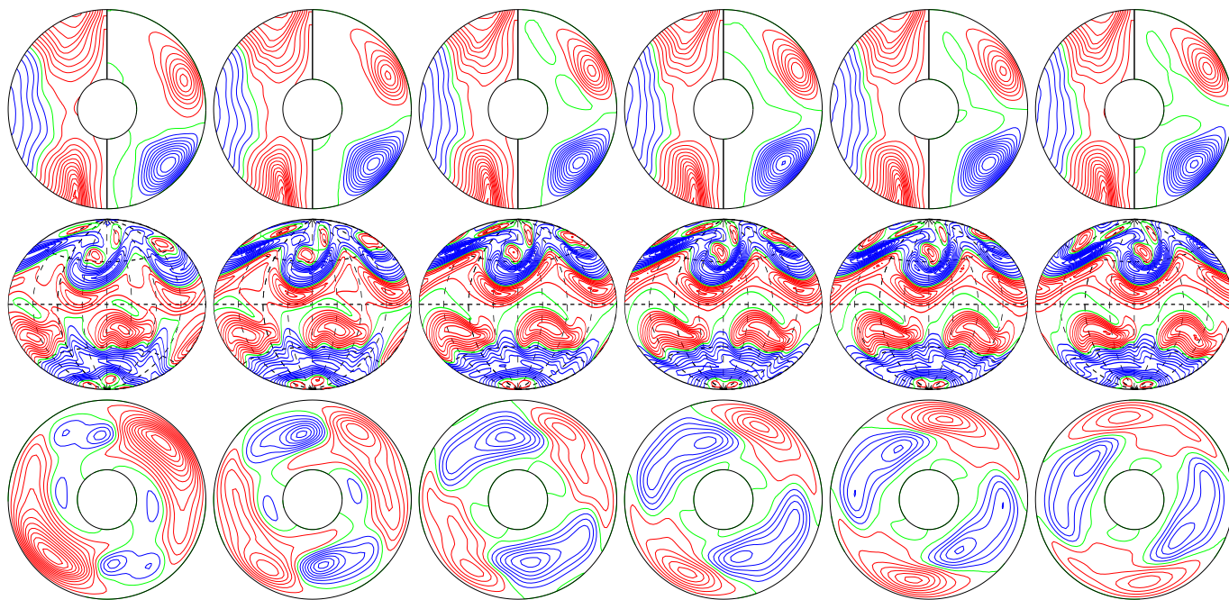
a.e03p1t03r-50000m1n2N2z1.65e5aca E_{\text{kin}}
