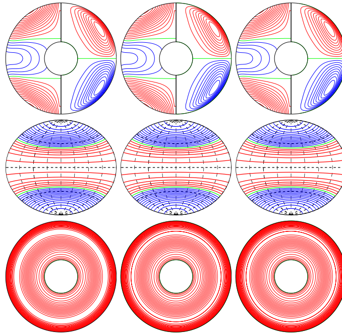
a.e03p1t03r-50000m1n2N2z1e0ac E_{\text{kin}}
