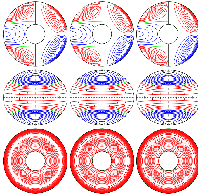
a.e03p1t03r-50000m1n2N2z1e2ac E_{\text{kin}}
