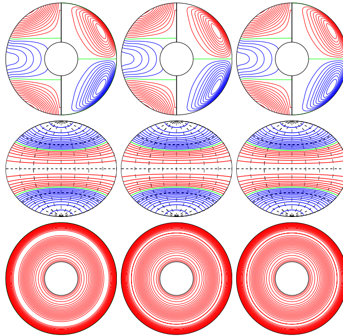
a.e03p1t03r-50000m1n2N2z1e4ac E_{\text{kin}}
