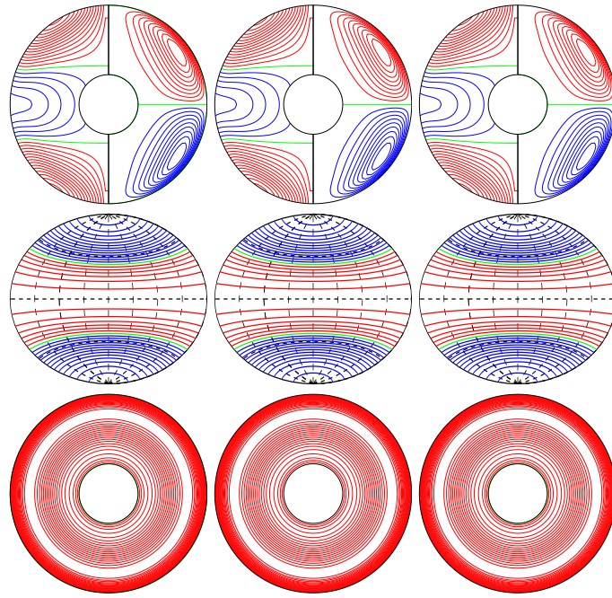
a.e03p1t03r-50000m1n2N2z1e3ac E_{\text{kin}}
