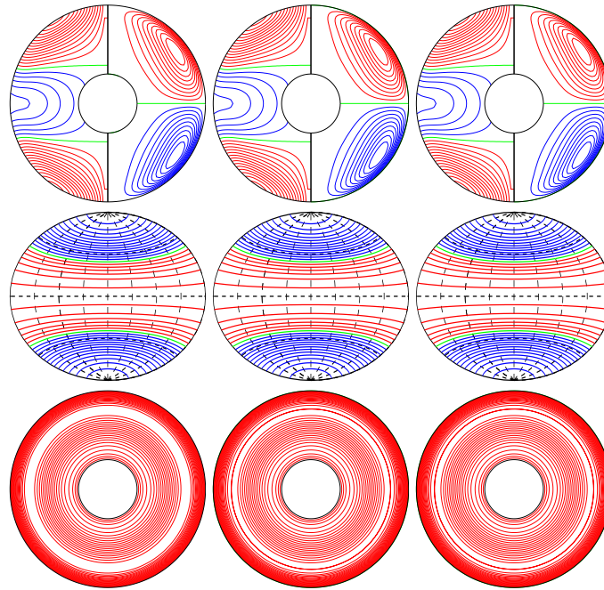
a.e03p1t03r-50000m1n2N2z1e1ac E_{\text{kin}}
