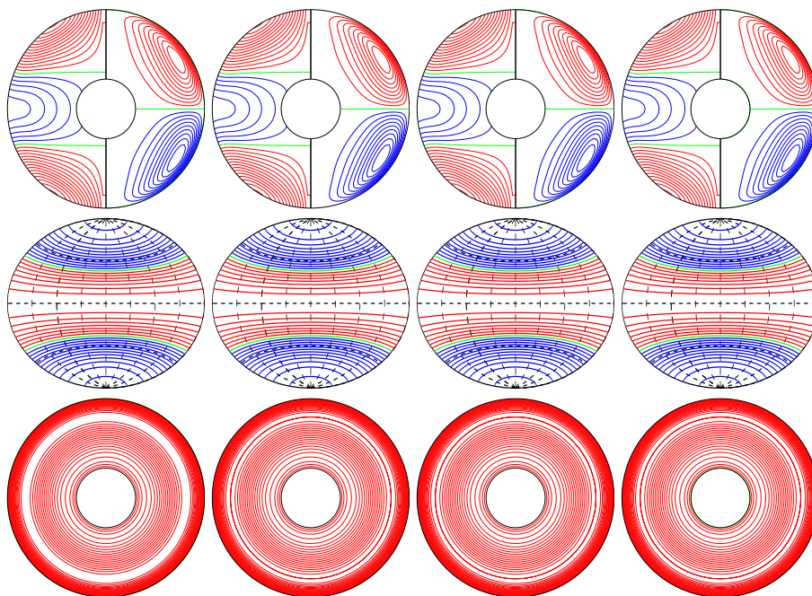
a.e03p1t03r-50000m1n2N2z1e4ac E_{\text{kin}}
