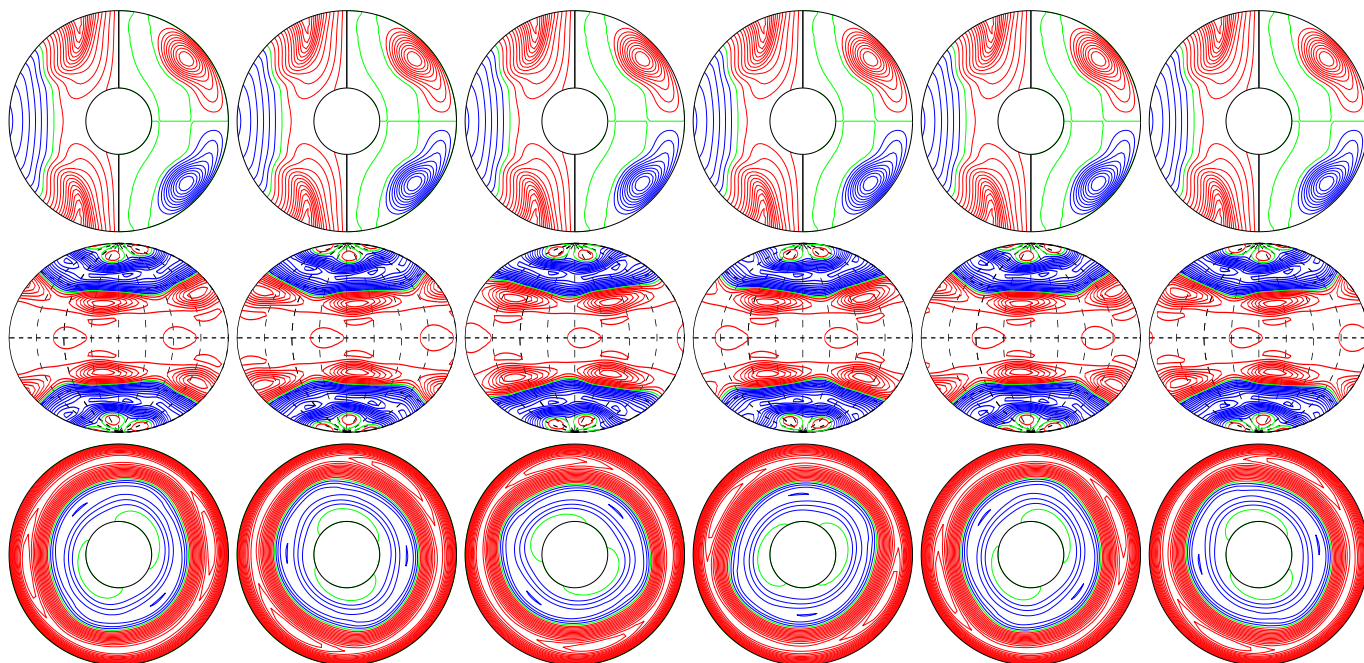
a.e03p1t03r-50000m1n2N2z1.25e5ac E_{\text{kin}}
