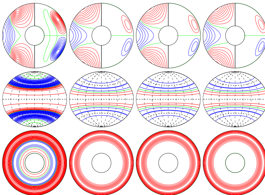
a.e03p1t03r-50000m1n2N2z1.1e5ac E_{\text{kin}}
