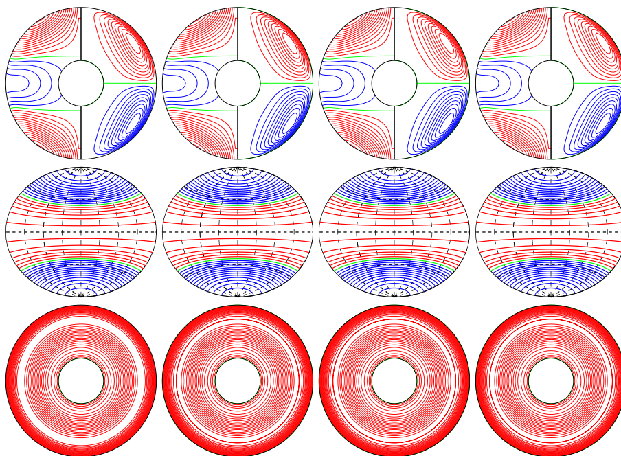
a.e03p1t03r-50000m1n2N2z1e0ac E_{\text{kin}}
