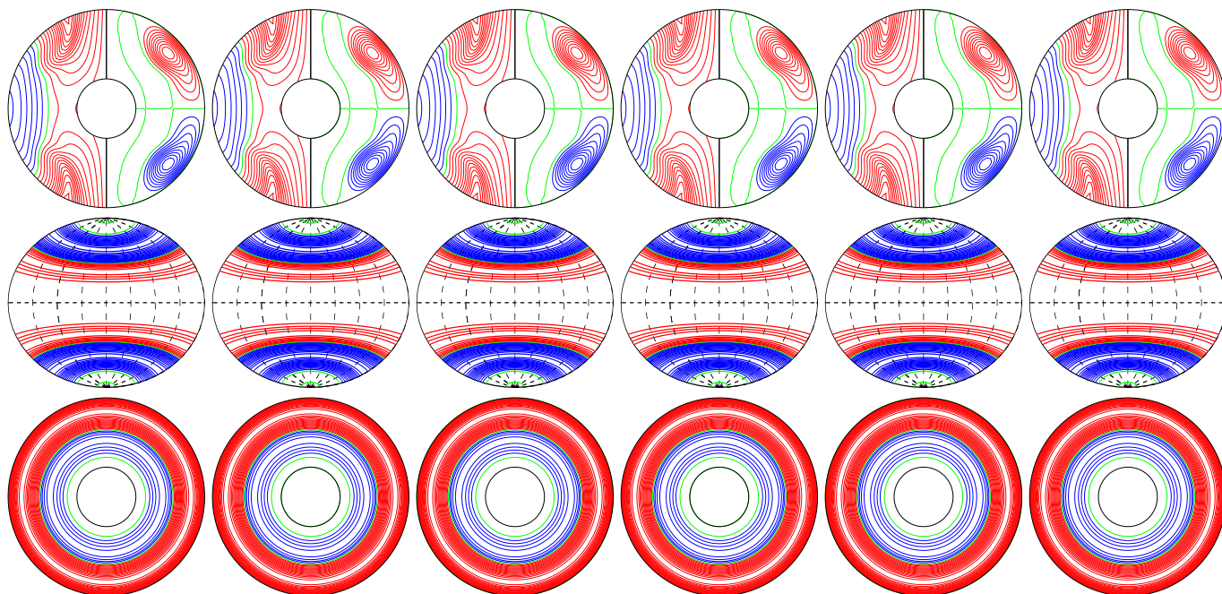
a.e03p1t03r-50000m1n2N2z1.15e5ac E_{\text{kin}}
