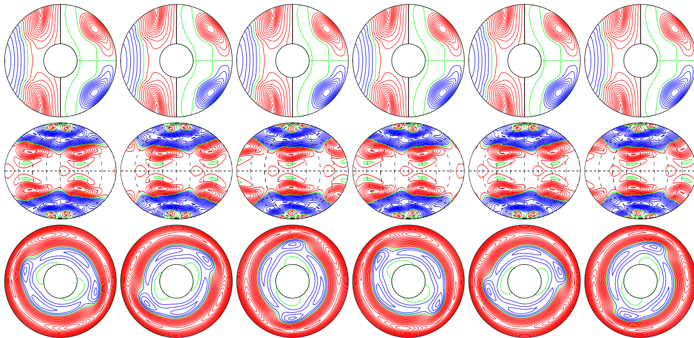
a.e03p1t03r-50000m1n2N2z1.38e5b E_{\text{kin}}
