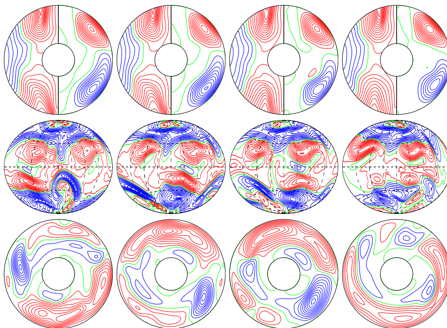
a.e03p1t03r-50000m1n2N2z1.64e5aca E_{\text{kin}}
