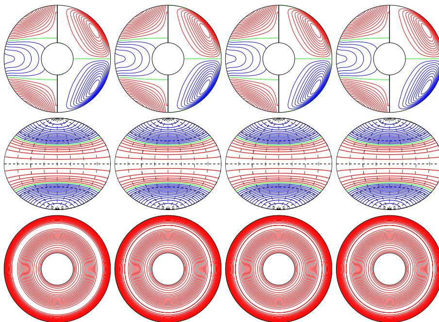
a.e03p1t03r-50000m1n2N2z1e1ac E_{\text{kin}}
