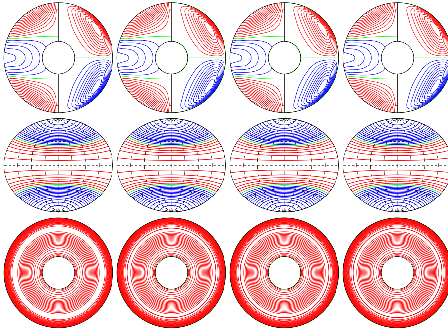
a.e03p1t03r-50000m1n2N2z1e2ac E_{\text{kin}}
