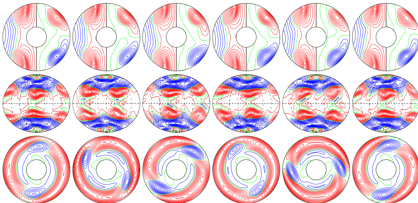
a.e03p1t03r-50000m1n2N2z1.55e5aca E_{\text{kin}}
