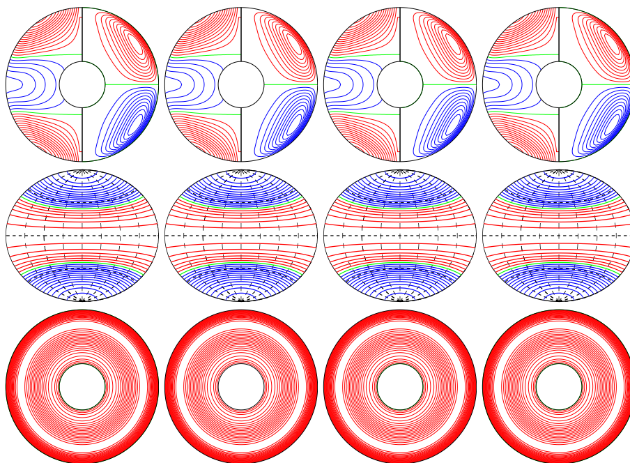
a.e03p1t03r-50000m1n2N2z1e3ac E_{\text{kin}}
