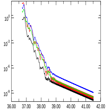
E_{\text{magn,dip}}
