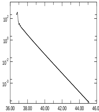
E_{\text{magn, quadr.}}
