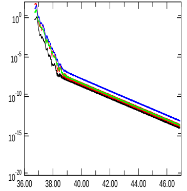
E_{\text{magn, dip}}
