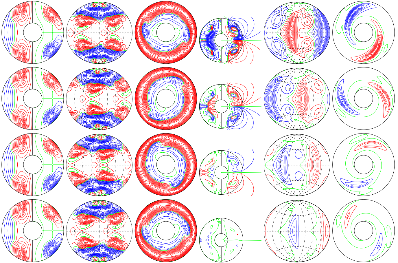
a.e03p1t03r-50000m1p4n2N2z1.45e5a E_{\text{kin}}
