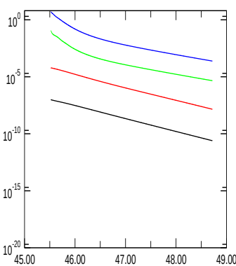
E_{\text{magn, quadr.}}
