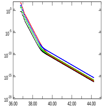
E_{magn,dip.}
