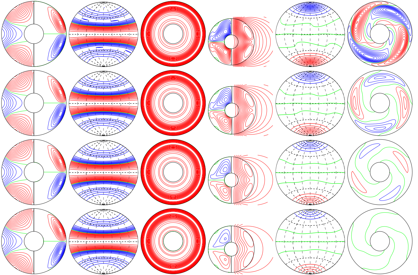
a.e03p1t03r-50000m1p10n2N2z1.05e5a E_{\text{kin}}
