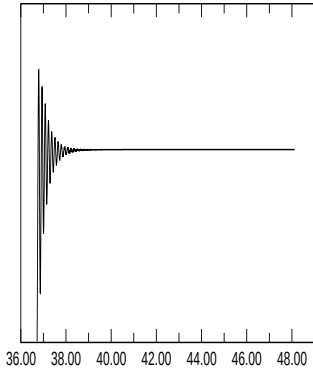
E_{kin,asymm.}
