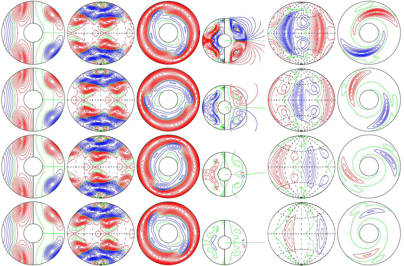
a.e03p1t03r-50000m1p4n2N2z1.45e5a E_{kin}
