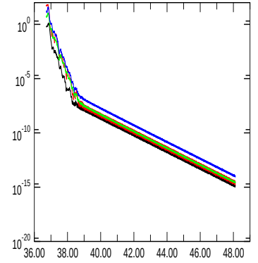
E_{magn,dip.}
