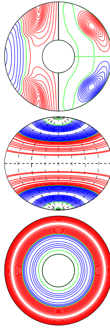
a.e03p1t03r-50000m1n2N2z1.17e5Bincr E_{\text{kin}}
