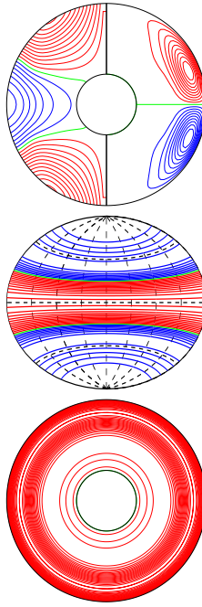
a.e03p1t03r-50000m1n2N2z1.02incr E_{\text{kin}}
