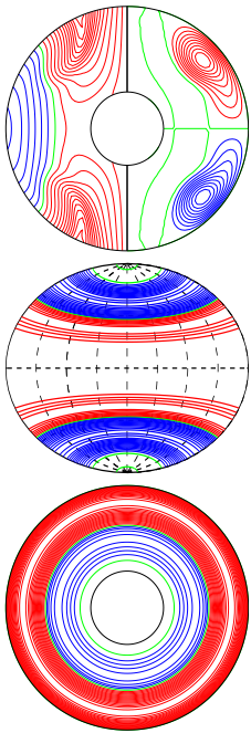
a.e03p1t03r-50000m1n2N2z1.16e5Bincr E_{kin}
