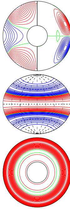
a.e03p1t03r-50000m1n2N2z1.14incr E_{\text{kin}}
