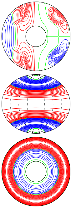
a.e03p1t03r-50000m1n2N2z1.18e5Bincr E_{kin}
