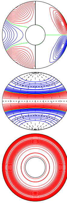
a.e03p1t03r-50000m1n2N2z1.06incr E_{\text{kin}}
