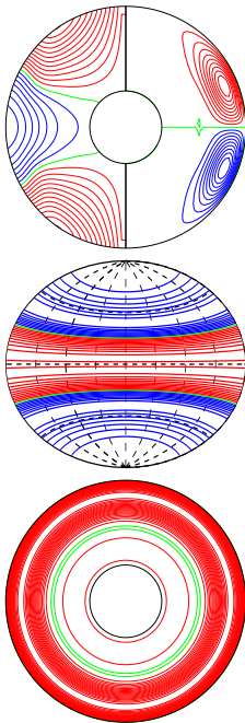
a.e03p1t03r-50000m1n2N2z1.12incr E_{kin}
