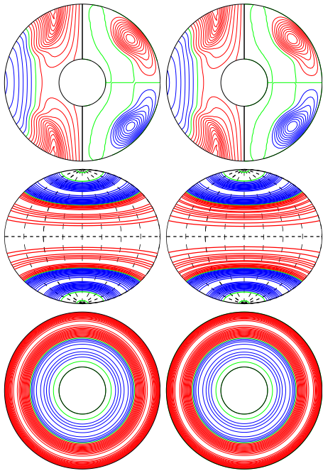
a.e03p1t03r-50000m1n2N2z1.17e5Bincr E_{\text{kin}}
