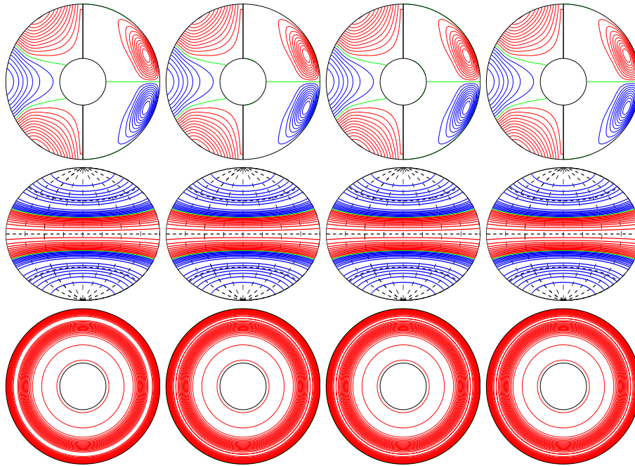
a.e03p1t03r-50000m1n2N2z1.10incr E_{\text{kin}}
