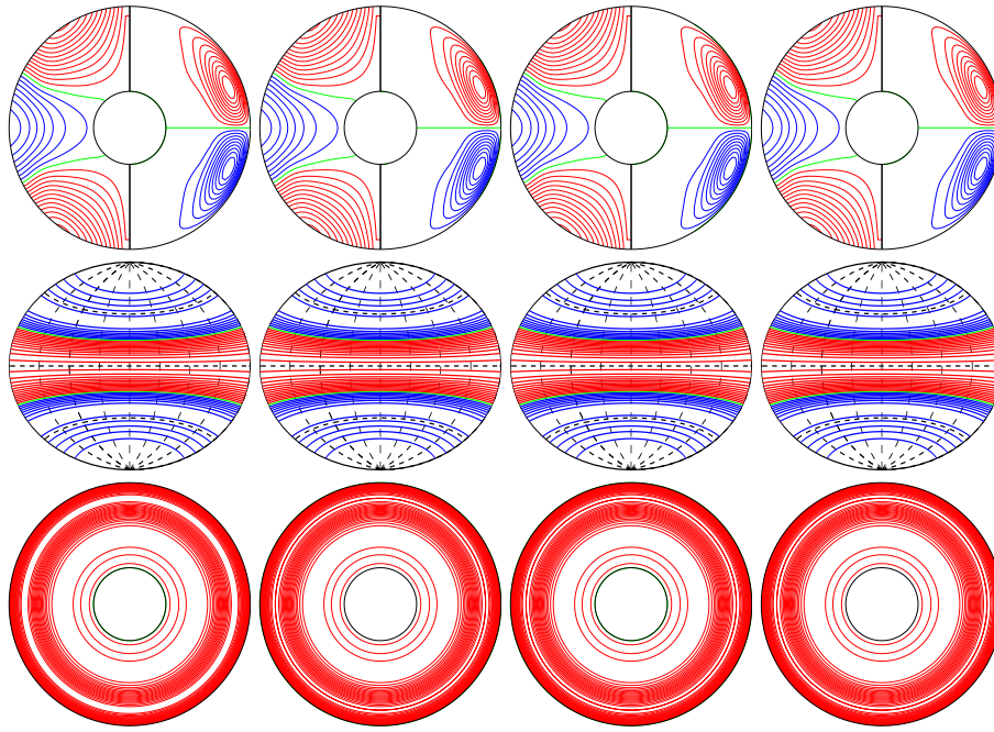
a.e03p1t03r-50000m1n2N2z1.02incr E_{\text{kin}}
