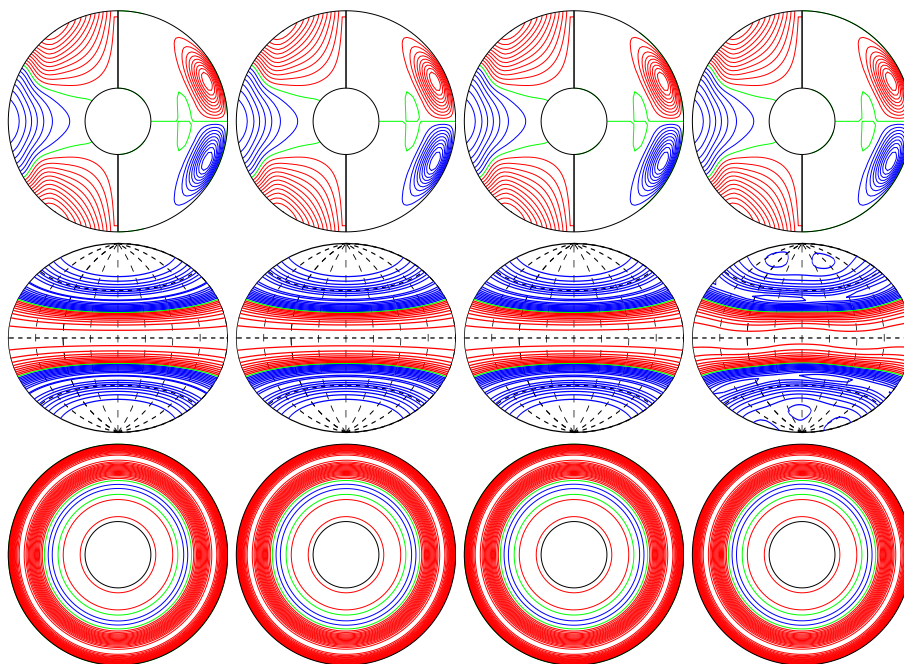
a.e03p1t03r-50000m1n2N2z1.16incr E_{\text{kin}}
