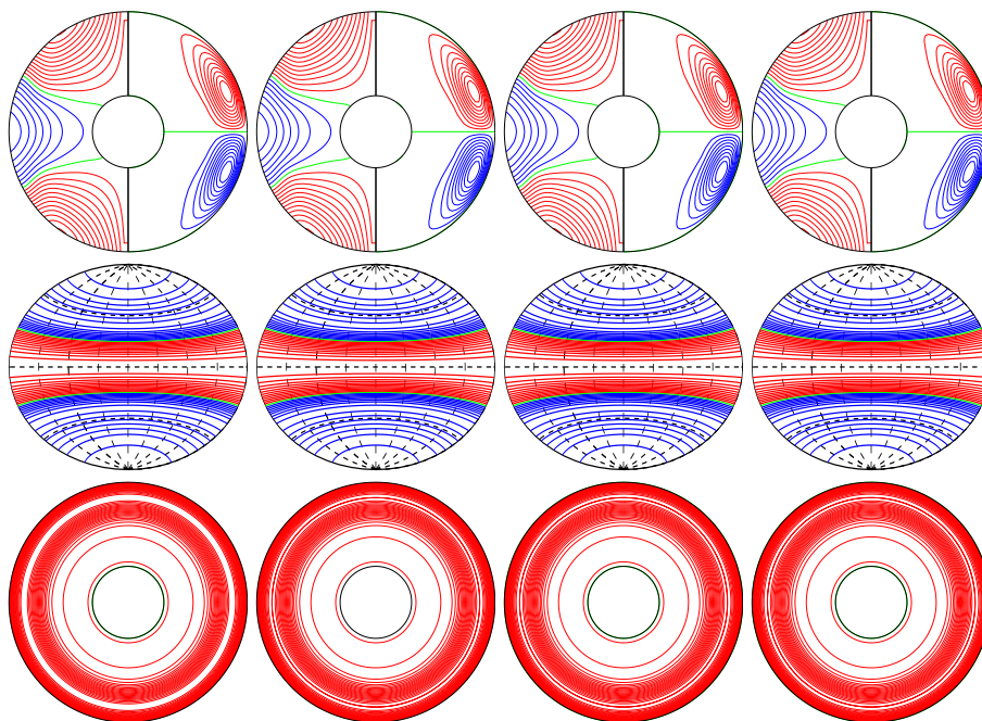
a.e03p1t03r-50000m1n2N2z1.08incr E_{\text{kin}}
