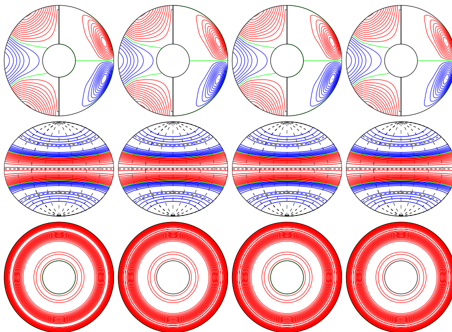
a.e03p1t03r-50000m1n2N2z1.04incr E_{\text{kin}}
