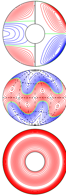
a.e03p1t03r-50000m1n2N2z1e2decr E_{kin}
