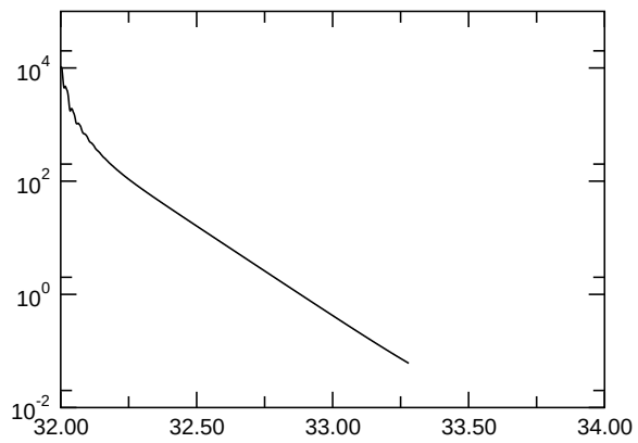
E_{kin,asymm.}
