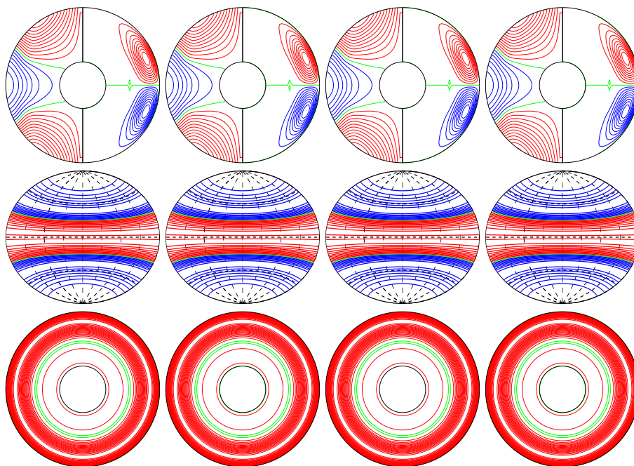
a.e03p1t03r-50000m1n2N2z1.12incr E_{\text{kin}}
