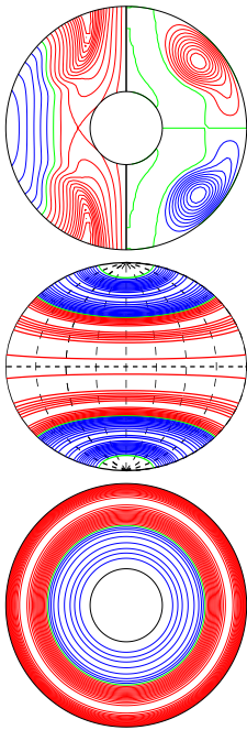
a.e03p1t03r-50000m1n2N2z1.22incr E_{kin}
