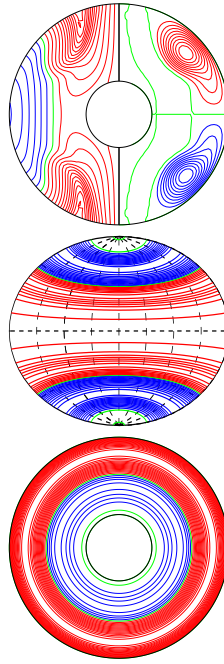
a.e03p1t03r-50000m1n2N2z1.20incr E_{\text{kin}}
