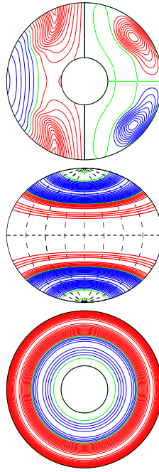
a.e03p1t03r-50000m1n2N2z1.18incr E_{\text{kin}}
