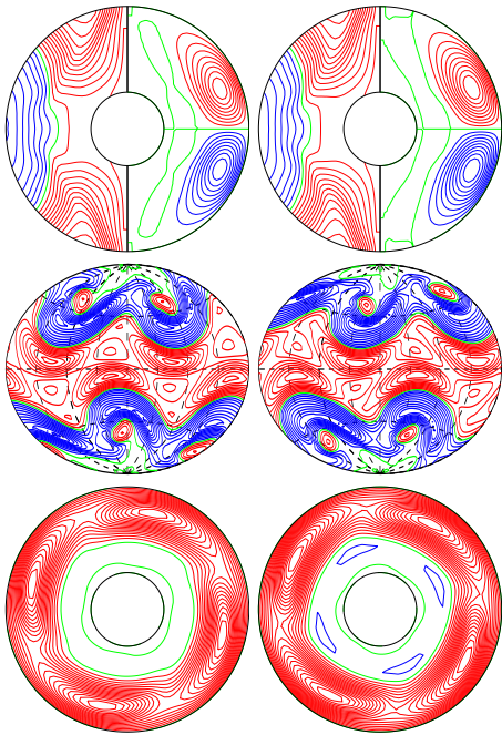
a.e03p1t03r-50000m1n2N2z1.55incr E_{kin}
