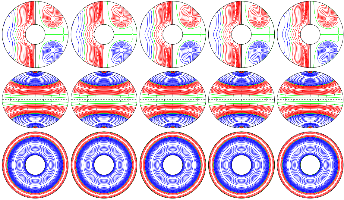
a.e03p1t03r-50000m16n2N2z1.8incr E_{\text{kin}}
