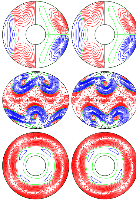
a.e03p1t03r-50000m1n2N2z1.35incr E_{kin}
