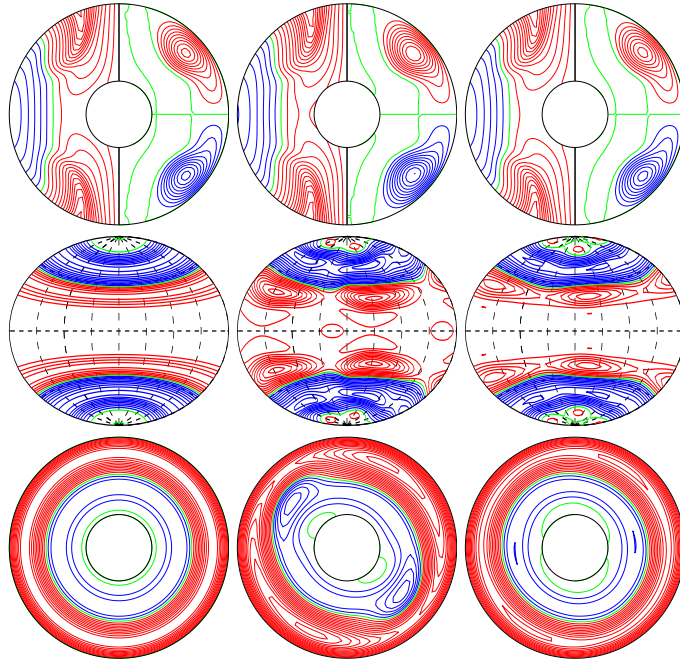
a.e03p1t03r-50000m1n2N2z1.20incr E_{\text{kin}}
