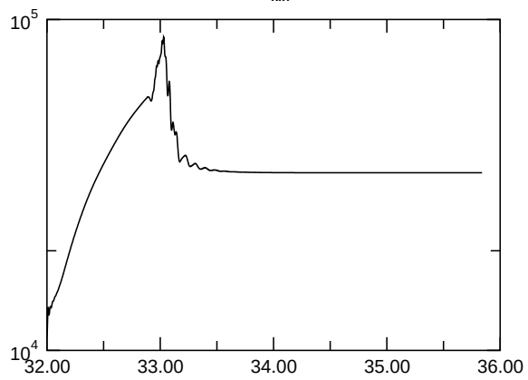
E_{kin,asymm.}
