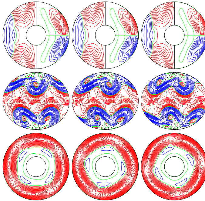
a.e03p1t03r-50000m1n2N2z1.30incr E_{\text{kin}}
