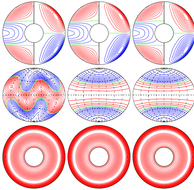
a.e03p1t03r-50000m1n2N2z1e2decr E_{\text{kin}}
