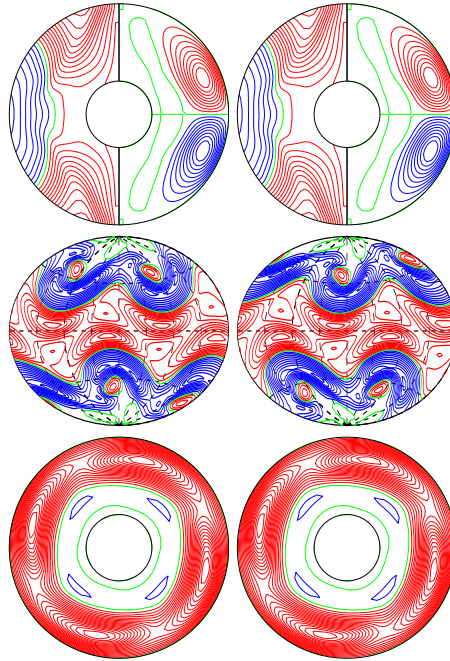
a.e03p1t03r-50000m1n2N2z1.40incr E_{kin}
