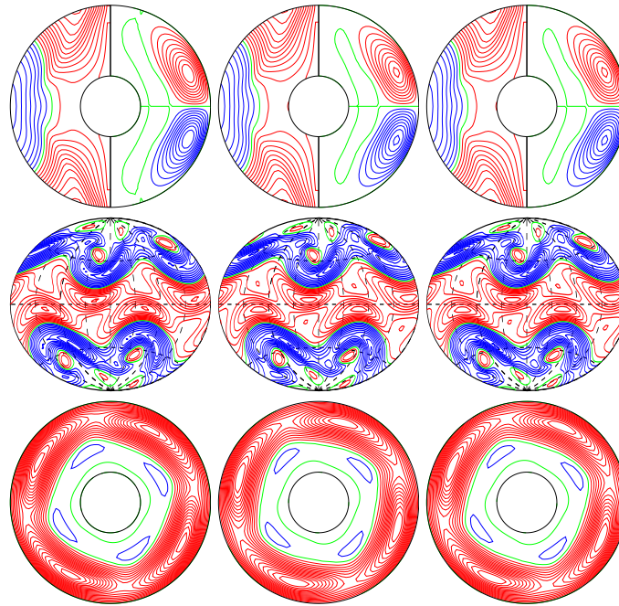
a.e03p1t03r-50000m1n2N2z1.28incr E_{kin}
