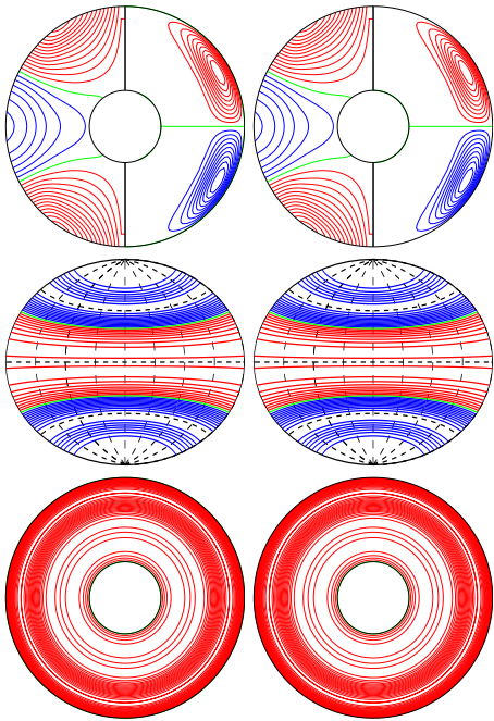
a.e03p1t03r-50000m1n2N2z1.0e5Z E_{\text{kin}}
