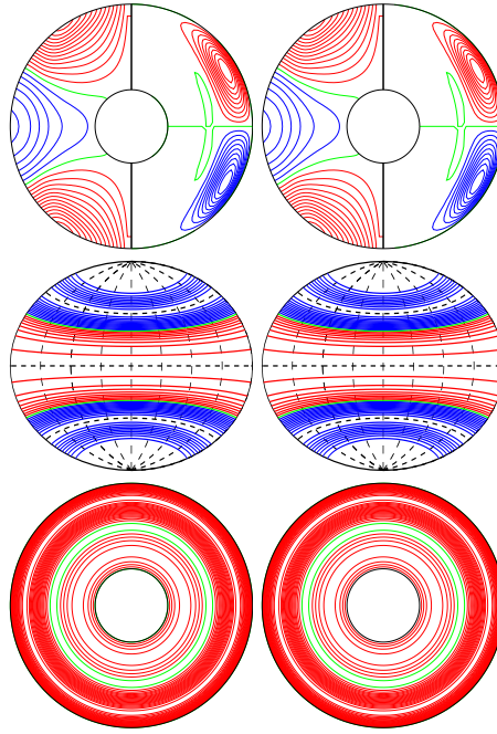
a.e03p1t03r-50000m1n2N2z1.12e5Z E_{\text{kin}}
