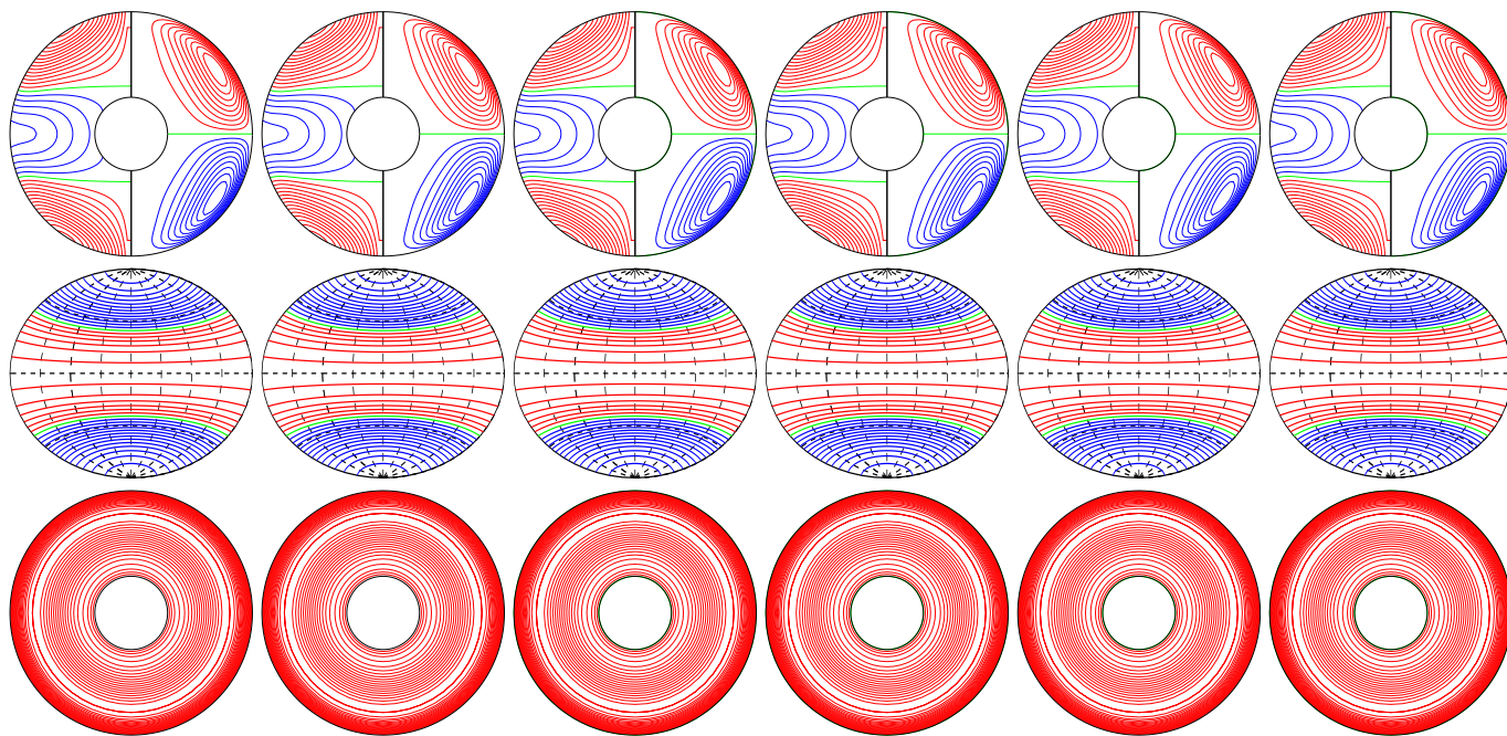
a.e03p1t03r-50000m16n2N2z1.0e2Z E_{\text{kin}}
