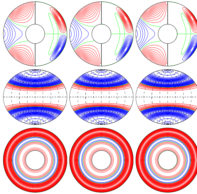
a.e03p1t03r-50000m1n2N2z1.22e5Z E_{\text{kin}}
