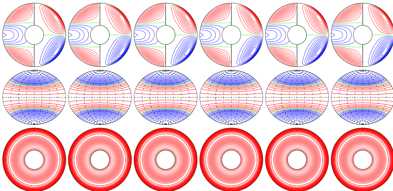
a.e03p1t03r-50000m16n2N2z1.0e0Z E_{\text{kin}}
