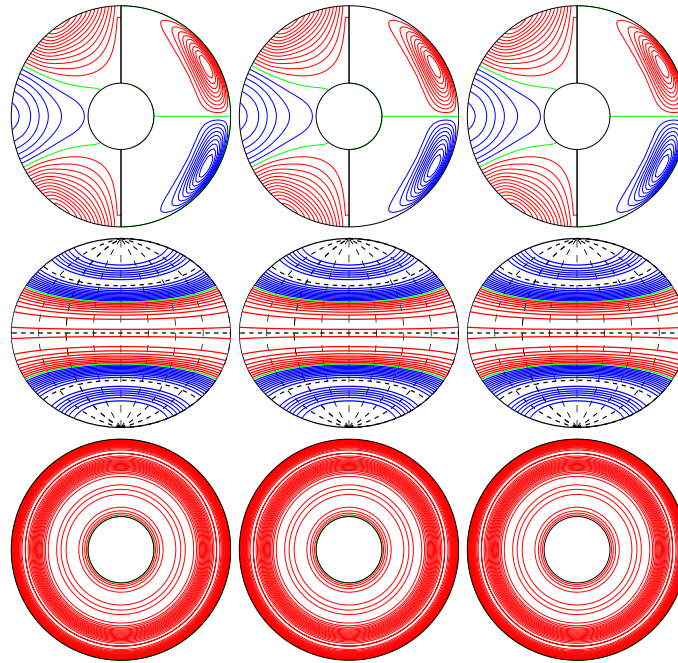
a.e03p1t03r-50000m1n2N2z1.0e5Z E_{\text{kin}}
