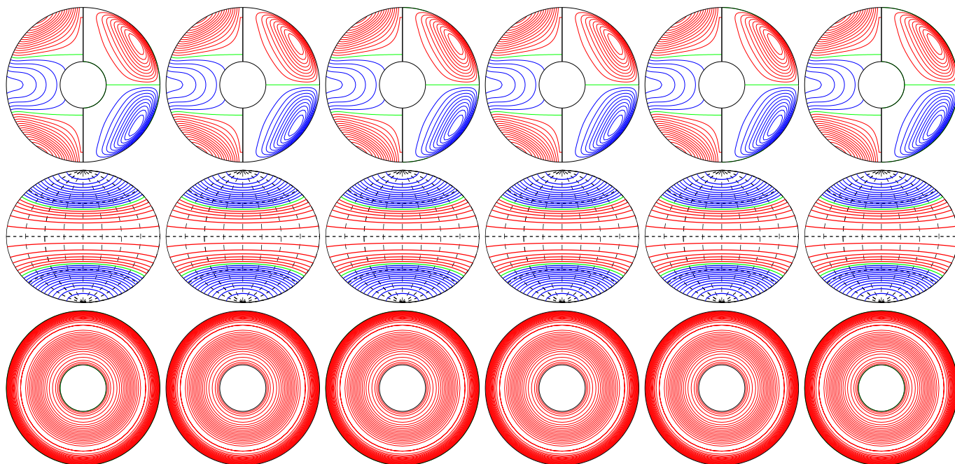
a.e03p1t03r-50000m16n2N2z1.0e1Z E_{\text{kin}}
