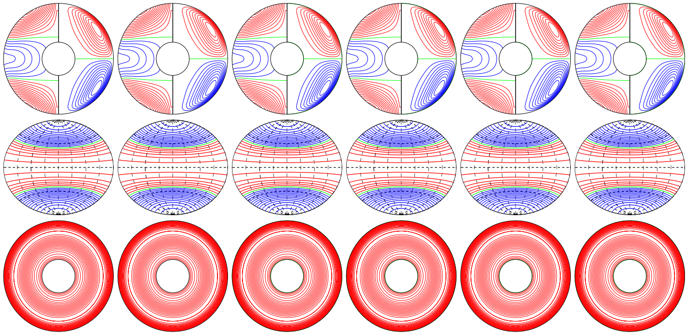
a.e03p1t03r-50000m16n2N2z1.0e2Z E_{\text{kin}}
