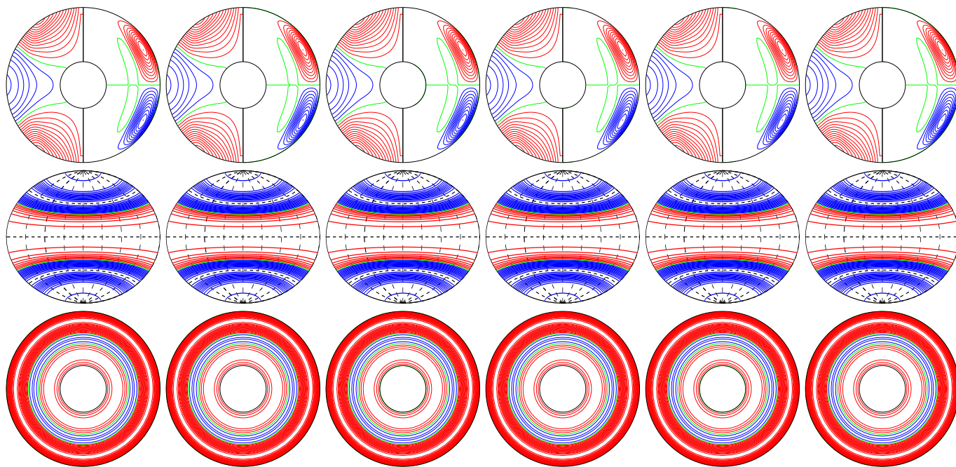
a.e03p1t03r-50000m16n2N2z1.2e5Z E_{\text{kin}}
