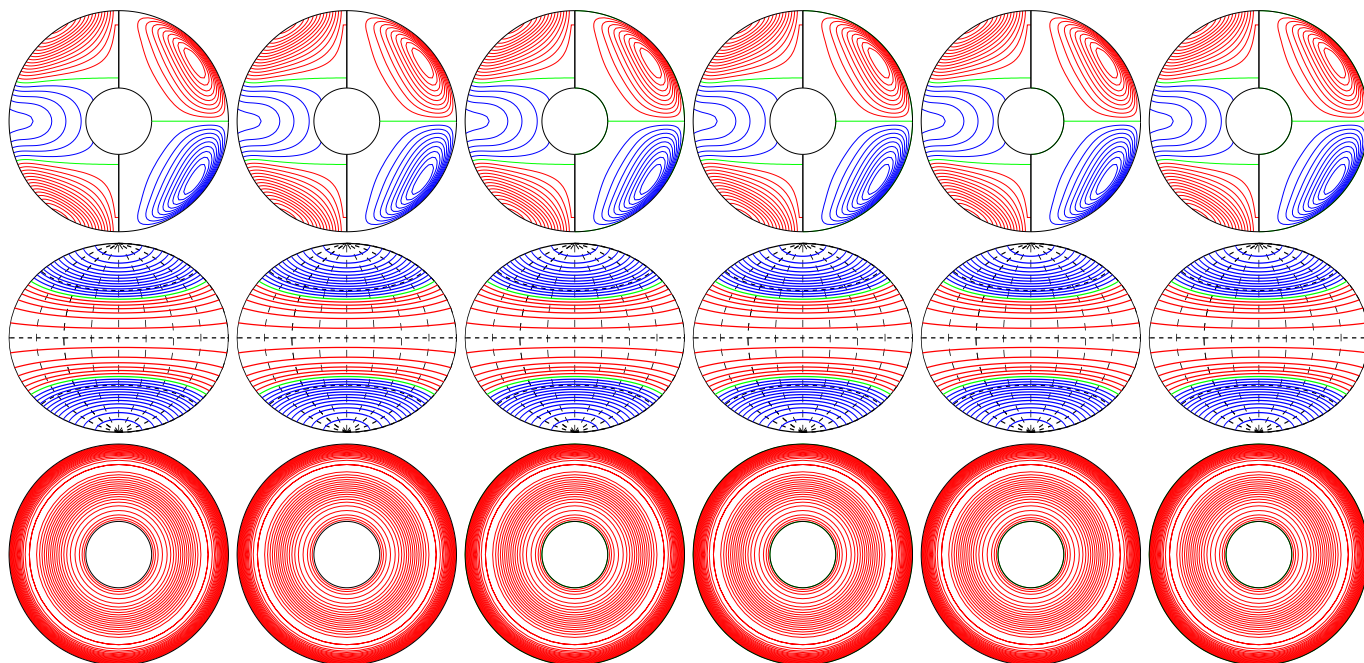
a.e03p1t03r-50000m16n2N2z1.0e2Z E_{\text{kin}}
