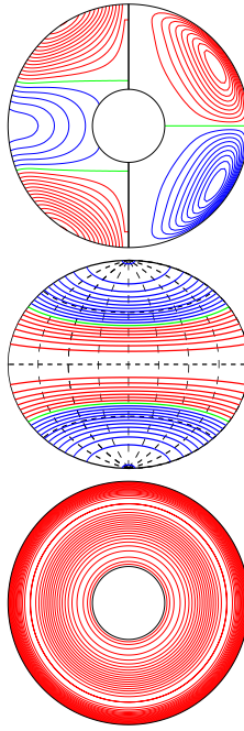
a.e03p1t03r-50000m1n2N2z1.0e4Y E_{\text{kin}}
