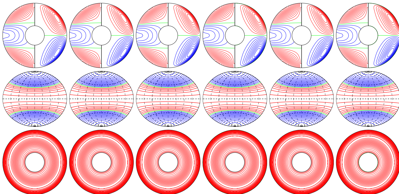
a.e03p1t03r-50000m16n2N2z1.0e0Y E_{\text{kin}}
