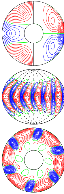
a.e03p1t03r-50000m1n2N2z6.0e4Ya E_{\text{kin}}
