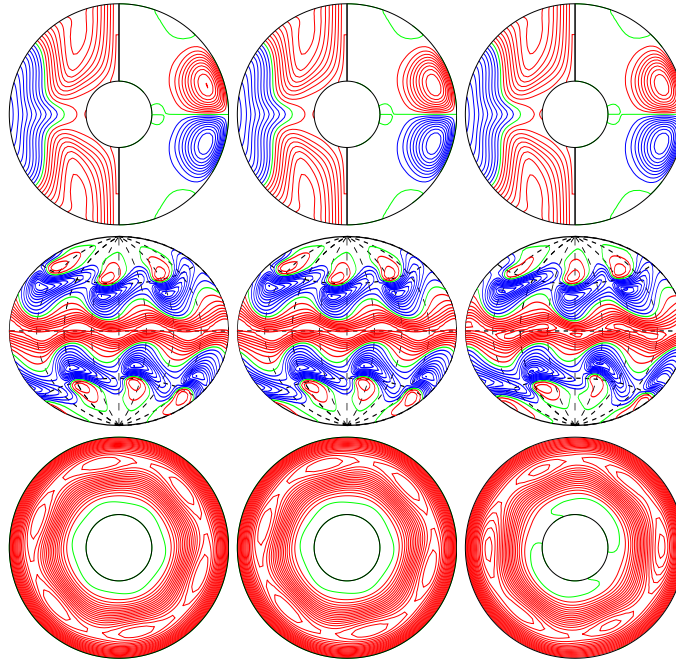
a.e03p1t03r-50000m1n2N2z1.4e5Y E_{\text{kin}}
