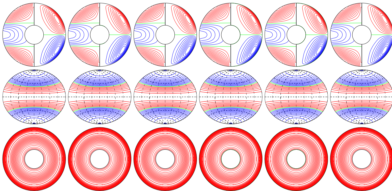
a.e03p1t03r-50000m16n2N2z1.0e4Y E_{\text{kin}}
