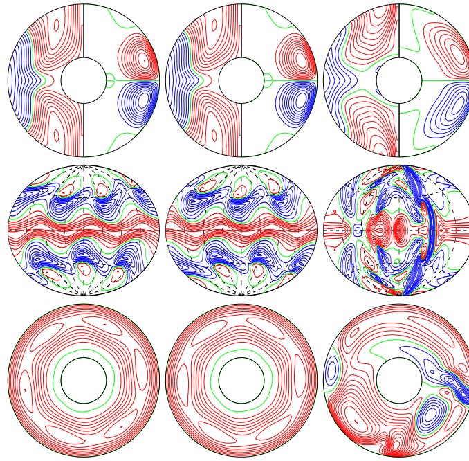
a.e03p1t03r-50000m1n2N2z1.5e5Y E_{\text{kin}}
