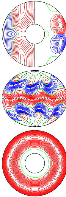
a.e03p1t03r-50000m1n2N2z1.3e5Y E_{\text{kin}}
