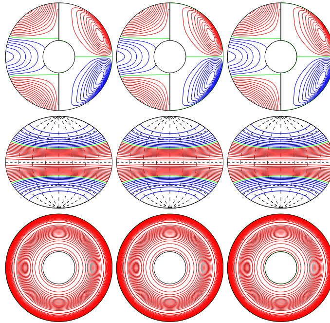
a.e03p1t03r-50000m1n2N2z3.0e4Y E_{\text{kin}}
