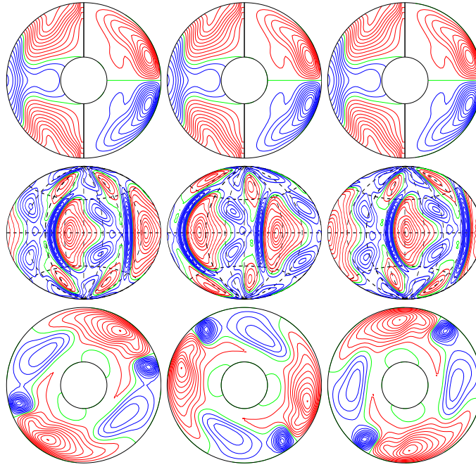
a.e03p1t03r-50000m1n2N2z1.0e5Ya E_{\text{kin}}
