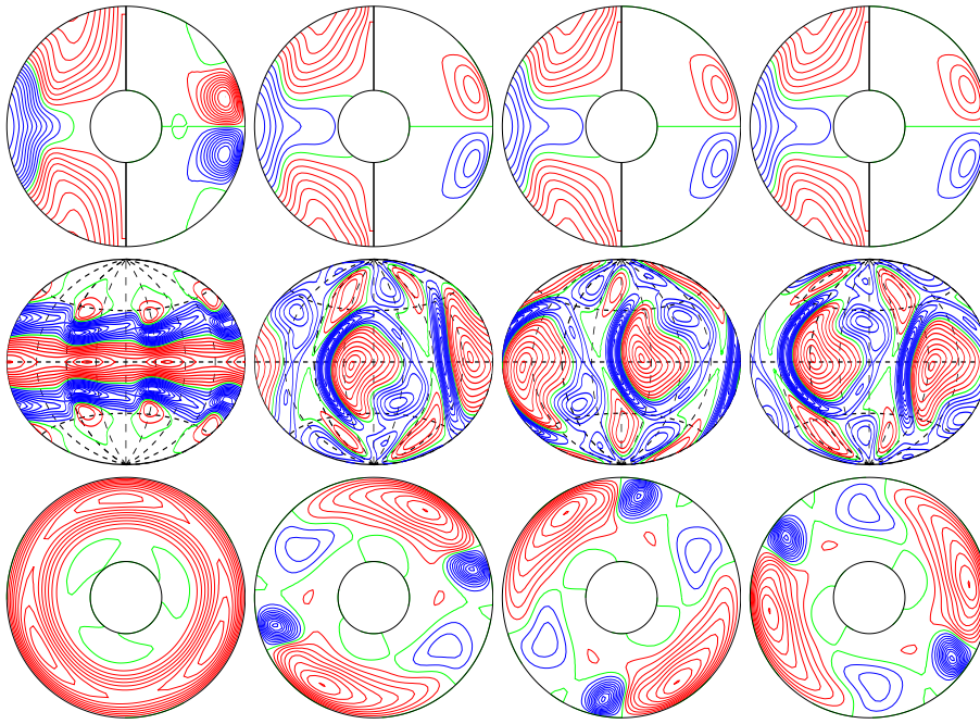
a.e03p1t03r-50000m1n2N2z9.0e4Y E_{\text{kin}}
