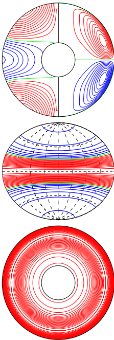
a.e03p1t03r-50000m1n2N2z4.4e4Y E_{\text{kin}}
