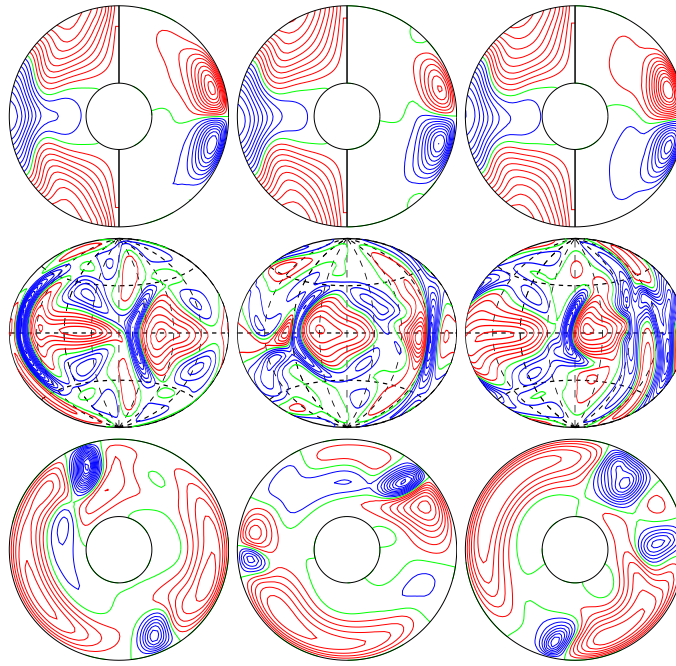
a.e03p1t03r-50000m1n2N2z8.0e4Ya E_{\text{kin}}
