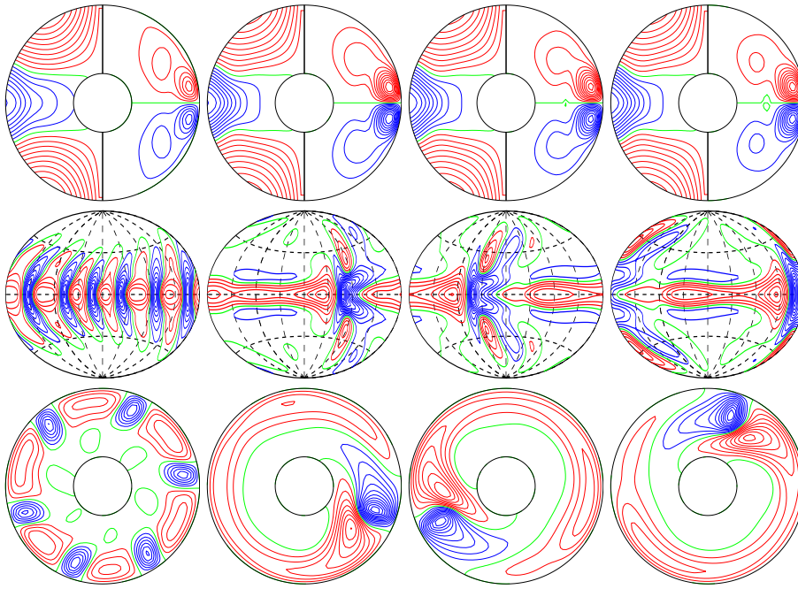
a.e03p1t03r-50000m1n2N2z6.0e4Y E_{\text{kin}}
