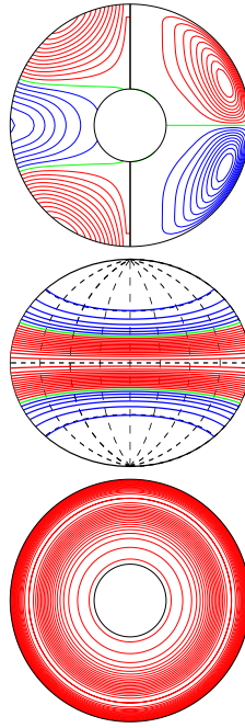
a.e03p1t03r-50000m1n2N2z4.2e4Y E_{\text{kin}}
