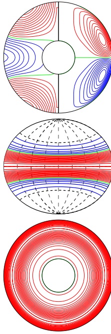
a.e03p1t03r-50000m1n2N2z4.6e4Y E_{\text{kin}}
