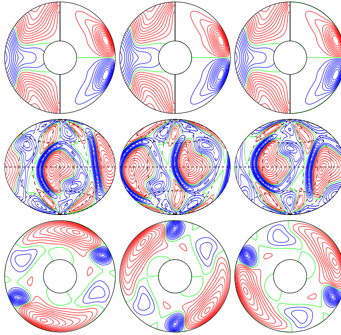
a.e03p1t03r-50000m1n2N2z9.0e4Ya E_{\text{kin}}
