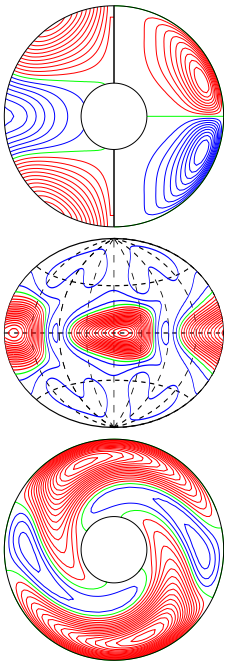
a.e03p1t03r-50000m1n2N2z4.6e4Ya E_{\text{kin}}
