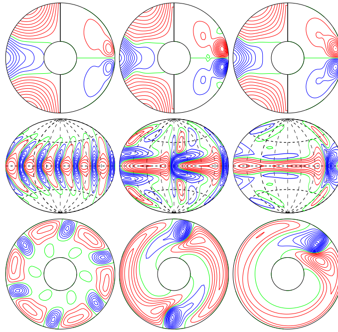
a.e03p1t03r-50000m1n2N2z6.0e4Ya E_{\text{kin}}
