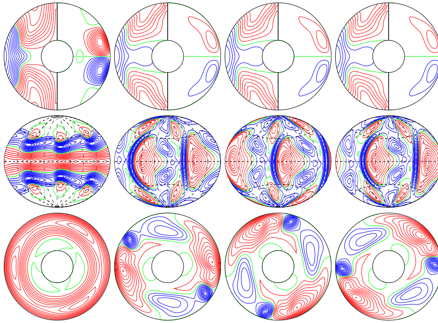
a.e03p1t03r-50000m1n2N2z1.0e5Y E_{\text{kin}}
