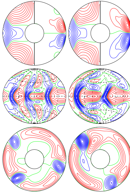
a.e03p1t03r-50000m1n2N2z7.0e4Ya E_{\text{kin}}
