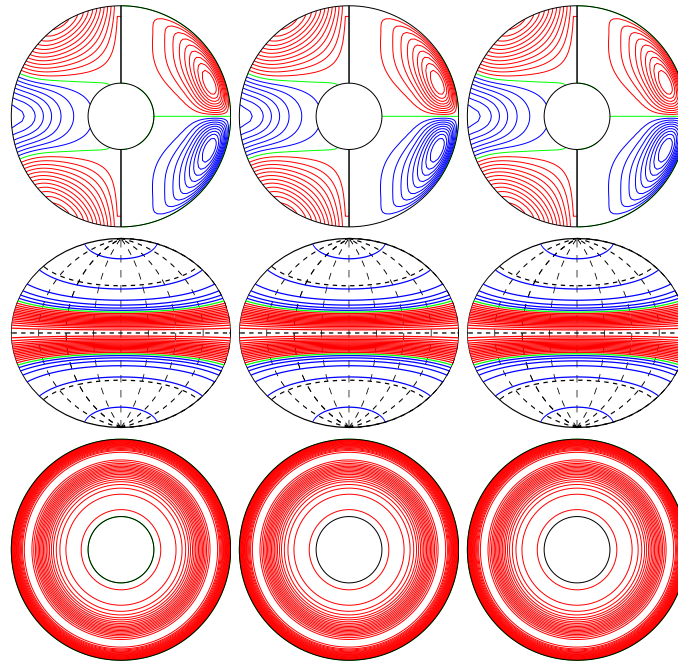
a.e03p1t03r-50000m1n2N2z5.0e4Y E_{\text{kin}}
