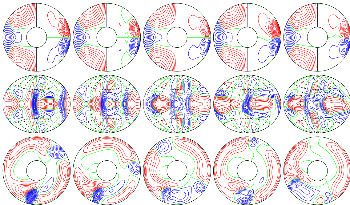
a.e03p1t03r-50000m1n2N2z7.0e4Y E_{\text{kin}}
