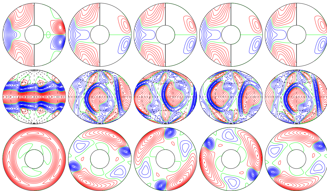
a.e03p1t03r-50000m1n2N2z9.0e4Y E_{\text{kin}}
