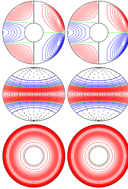
a.e03p1t03r-50000m1n2N2z4.2e4Y E_{\text{kin}}
