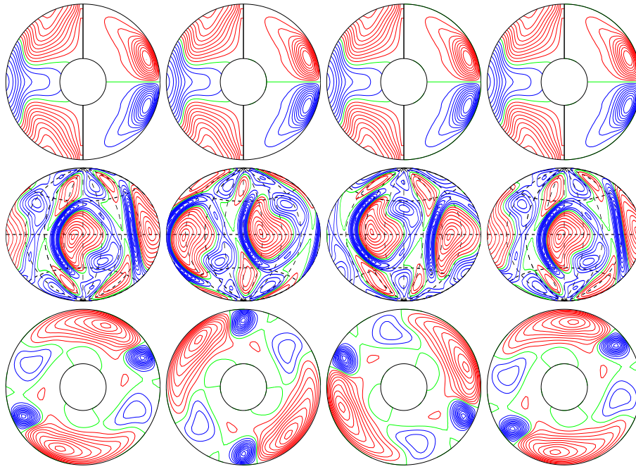
a.e03p1t03r-50000m1n2N2z9.0e4Ya E_{\text{kin}}
