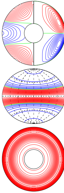
a.e03p1t03r-50000m1n2N2z4.4e4Y E_{\text{kin}}
