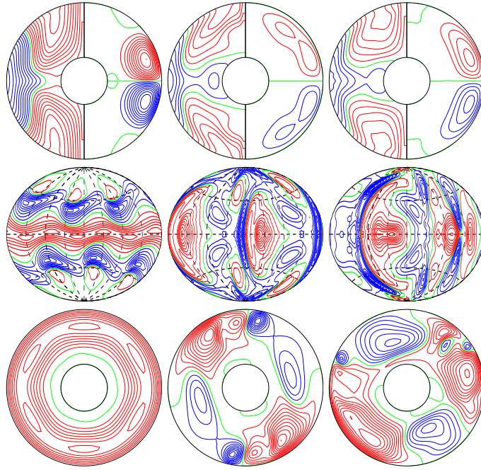
a.e03p1t03r-50000m1n2N2z1.3e5Y E_{\text{kin}}
