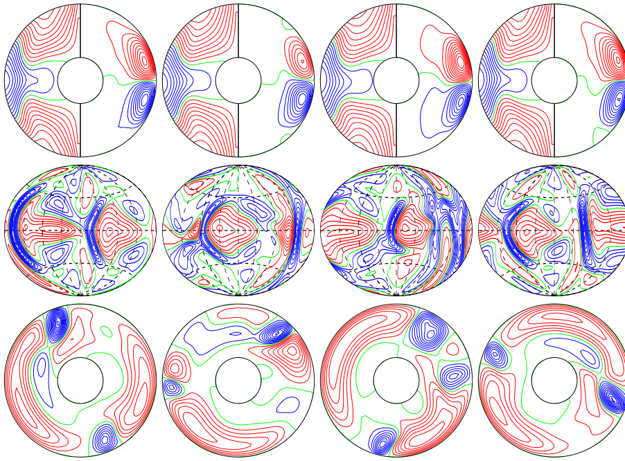
a.e03p1t03r-50000m1n2N2z8.0e4Ya E_{\text{kin}}
