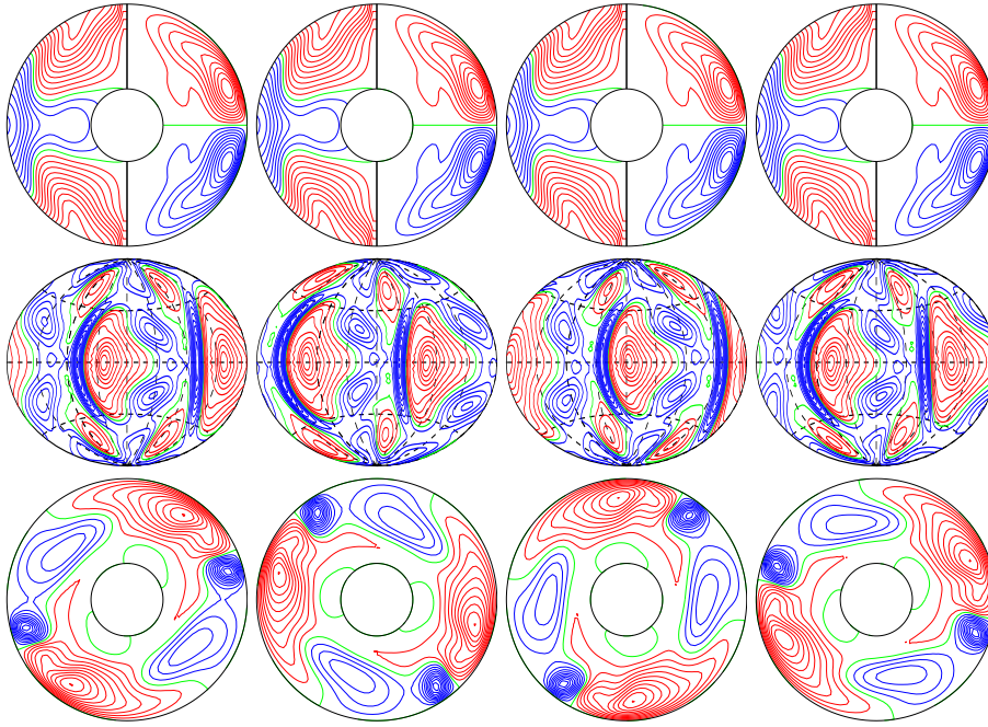
a.e03p1t03r-50000m1n2N2z1.0e5Ya E_{\text{kin}}
