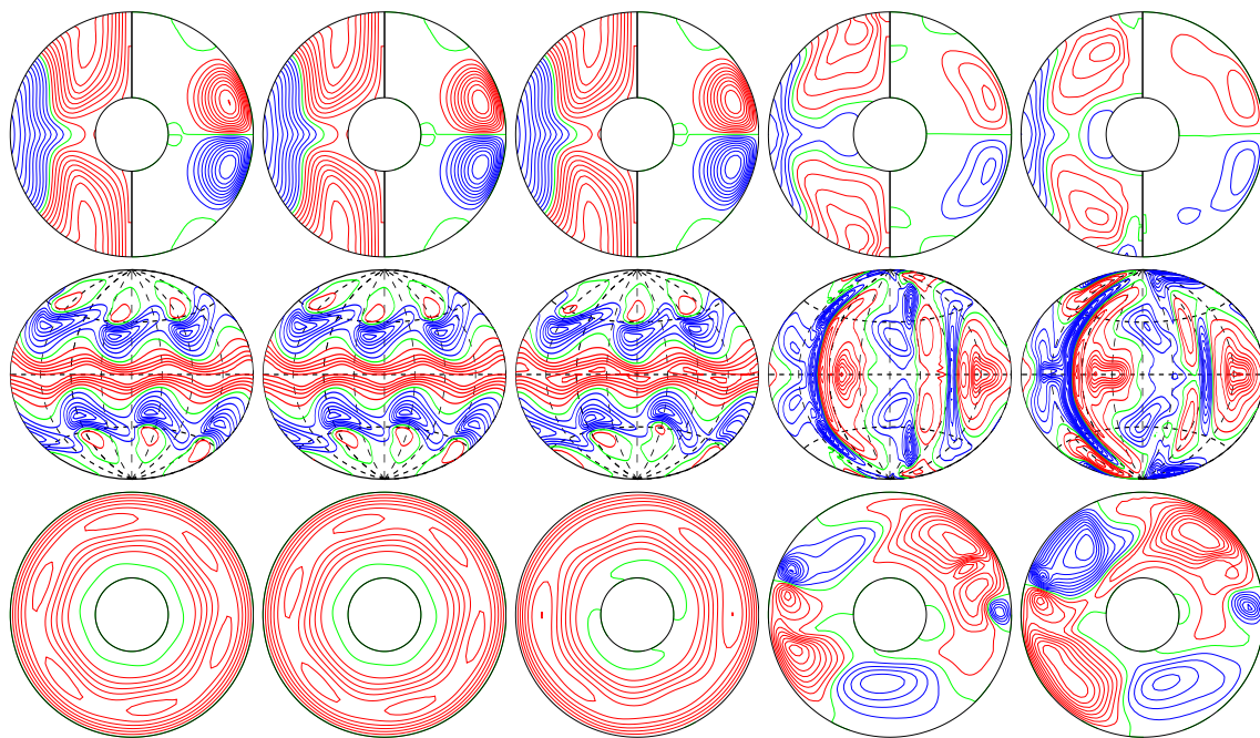
a.e03p1t03r-50000m1n2N2z1.4e5Y E_{\text{kin}}
