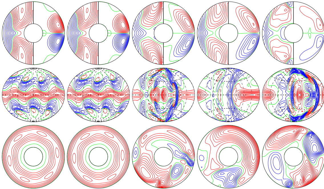
a.e03p1t03r-50000m1n2N2z1.5e5Y E_{\text{kin}}
