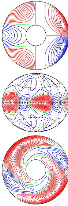
a.e03p1t03r-50000m1n2N2z4.68e4Yb E_{\text{kin}}
