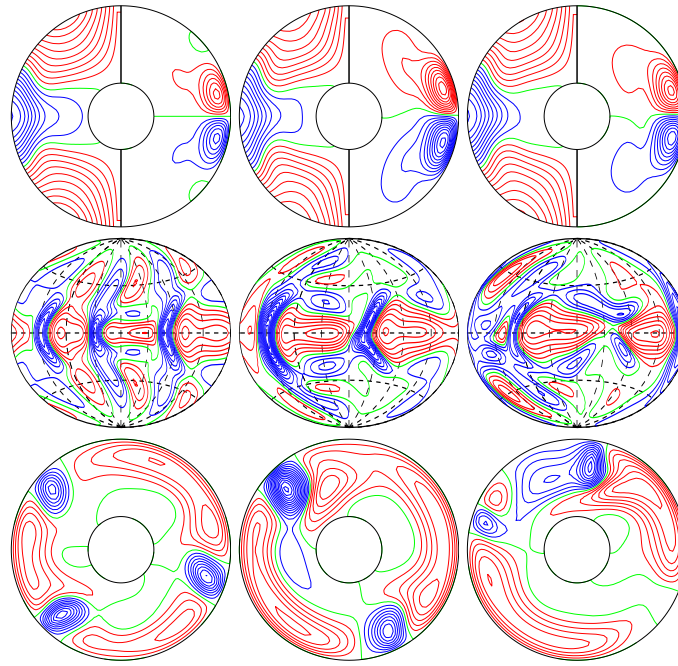
a.e03p1t03r-50000m1n2N2z7.0e4Ya E_{\text{kin}}
