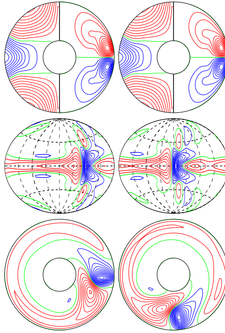
a.e03p1t03r-50000m1n2N2z5.8e4Ya E_{\text{kin}}
