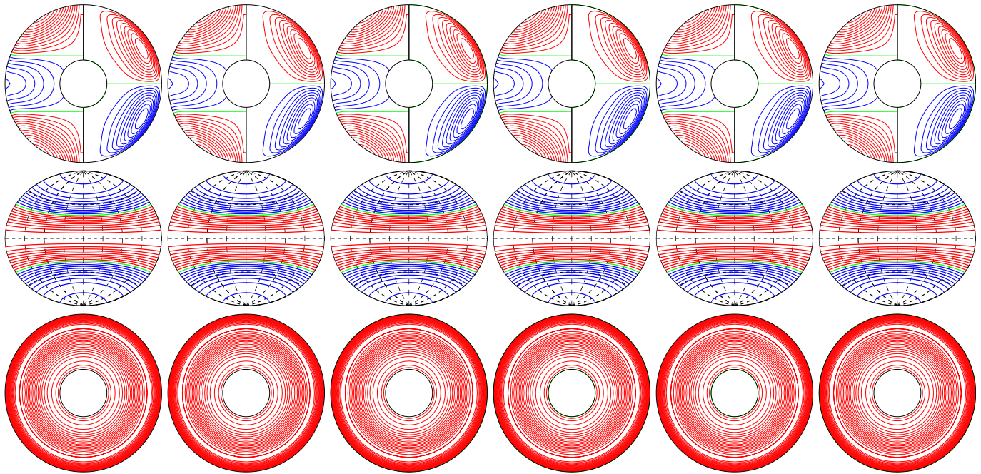
a.e03p1t03r-50000m16n2N2z2.0e4Y E_{\text{kin}}
