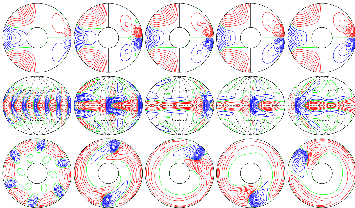
a.e03p1t03r-50000m1n2N2z6.0e4Ya E_{\text{kin}}
