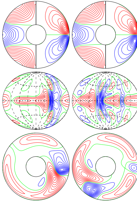
a.e03p1t03r-50000m1n2N2z5.6e4Ya E_{\text{kin}}
