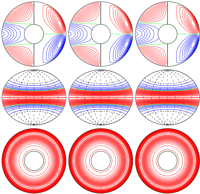
a.e03p1t03r-50000m1n2N2z4.6e4Y E_{\text{kin}}
