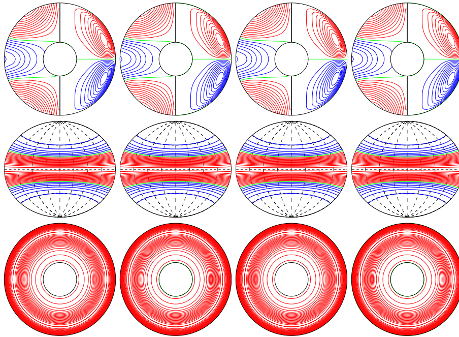
a.e03p1t03r-50000m1n2N2z4.2e4Y E_{\text{kin}}
