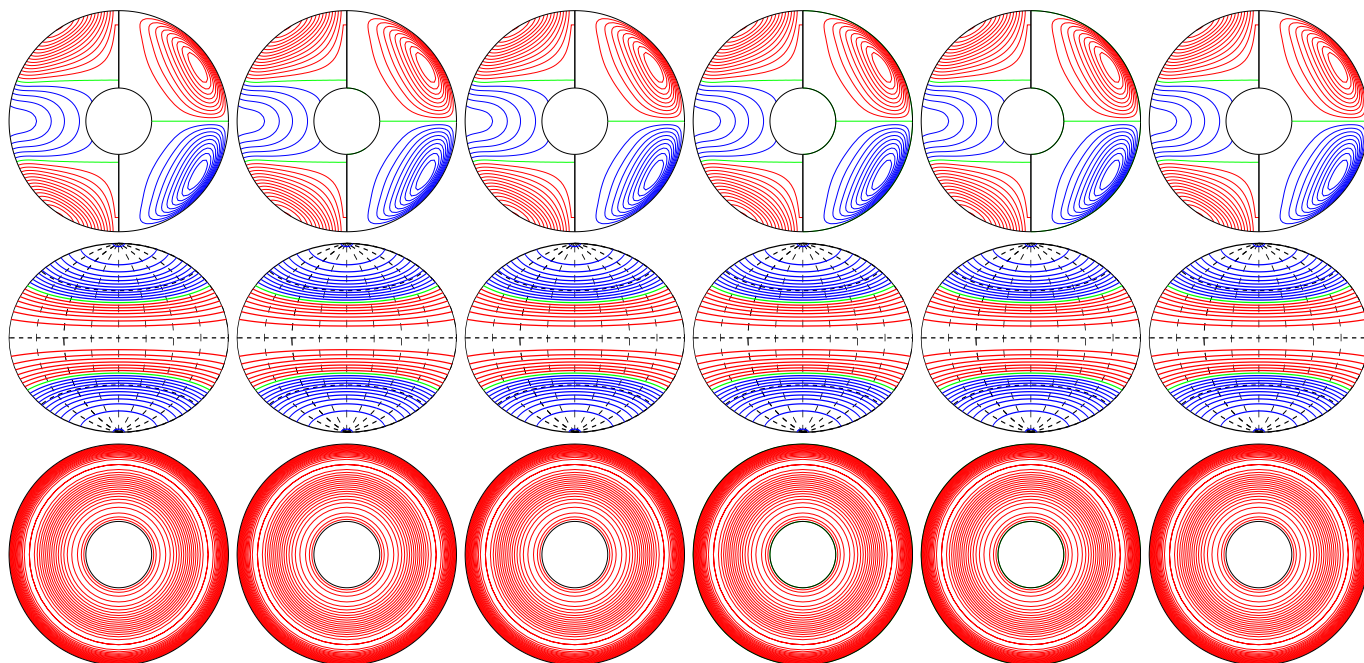
a.e03p1t03r-50000m16n2N2z1.0e4Y E_{\text{kin}}
