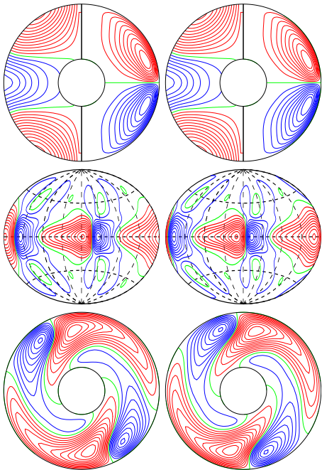
a.e03p1t03r-50000m1n2N2z4.7e4Ya E_{\text{kin}}
