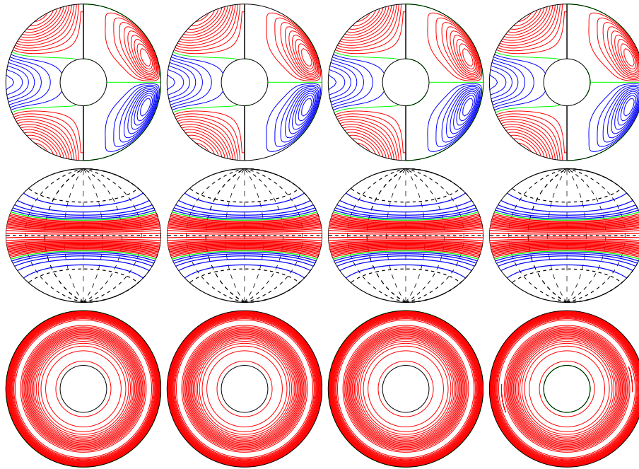
a.e03p1t03r-50000m1n2N2z4.8e4Y E_{\text{kin}}
