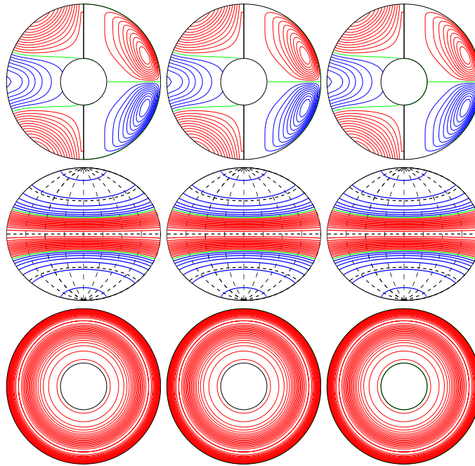
a.e03p1t03r-50000m1n2N2z4.4e4Y E_{\text{kin}}
