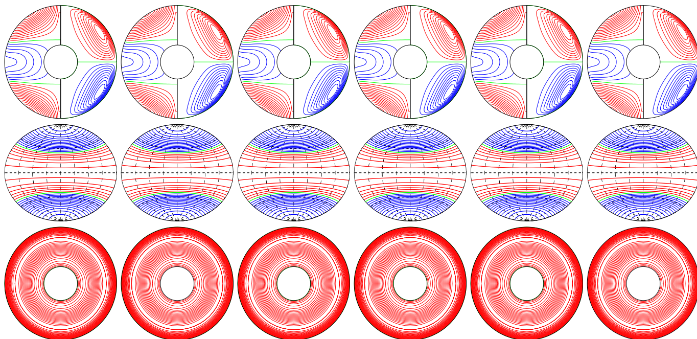
a.e03p1t03r-50000m16n2N2z1.0e1Y E_{\text{kin}}
