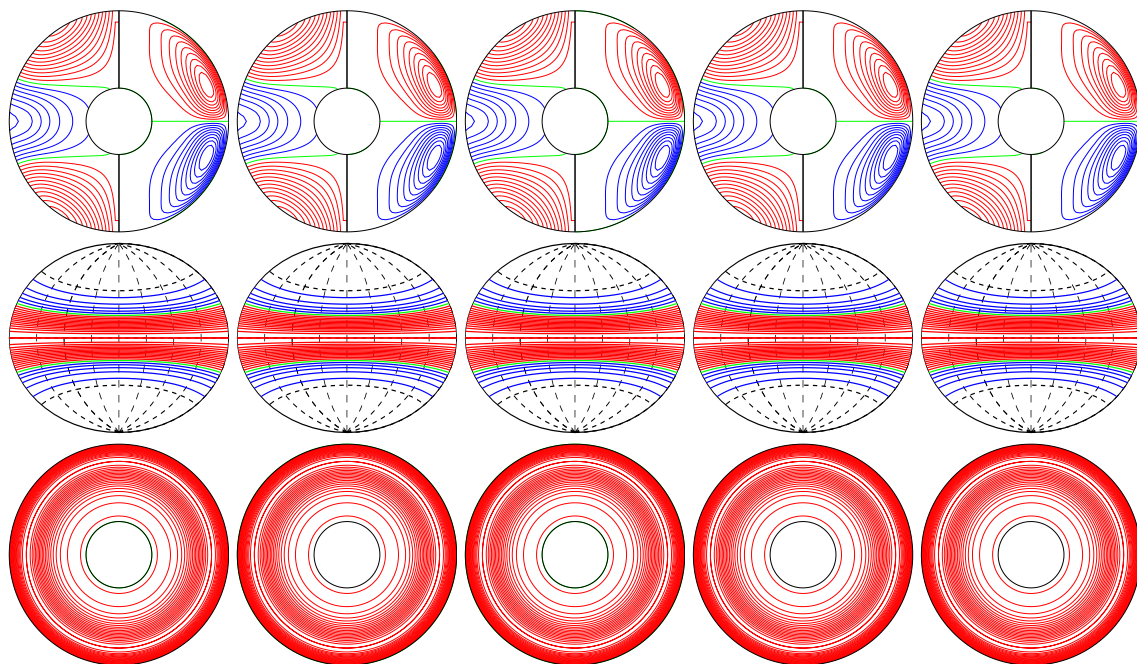
a.e03p1t03r-50000m1n2N2z4.6e4Y E_{\text{kin}}
