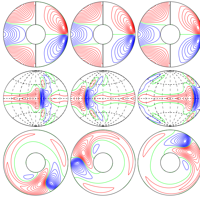
a.e03p1t03r-50000m1n2N2z5.4e4Ya E_{\text{kin}}
