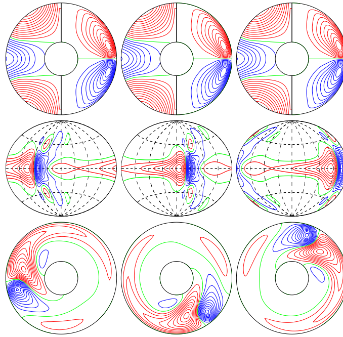
a.e03p1t03r-50000m1n2N2z5.2e4Ya E_{\text{kin}}
