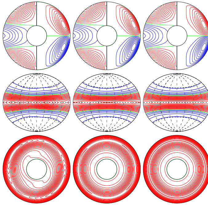
a.e03p1t03r-50000m1n2N2z4.5e4Ya E_{\text{kin}}
