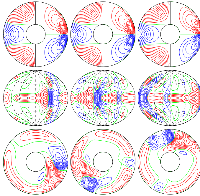
a.e03p1t03r-50000m1n2N2z5.6e4Ya E_{\text{kin}}
