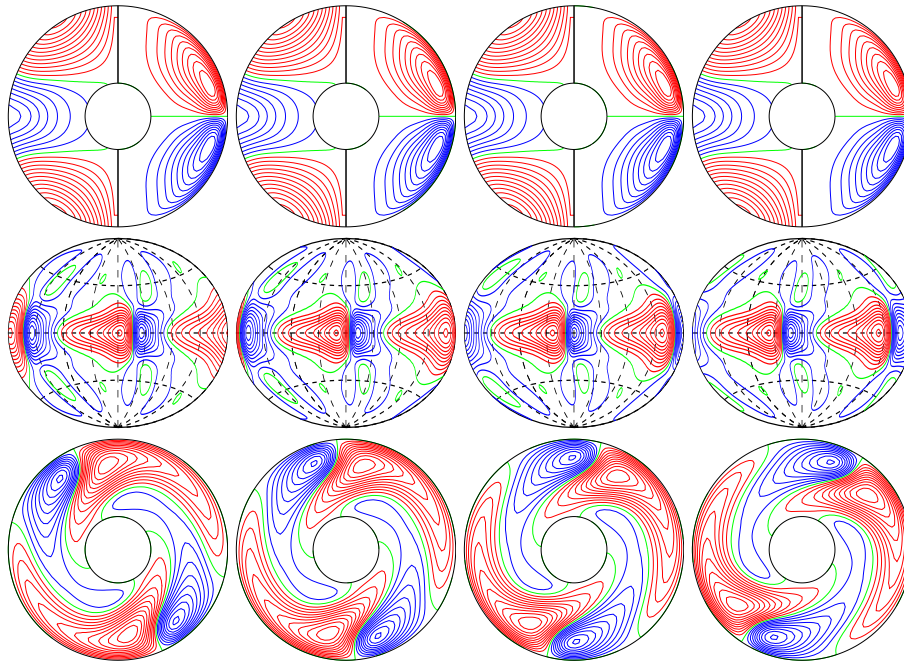
a.e03p1t03r-50000m1n2N2z4.7e4Ya E_{\text{kin}}
