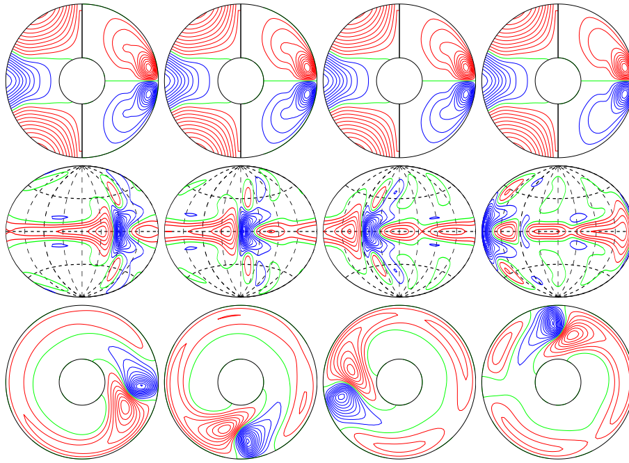
a.e03p1t03r-50000m1n2N2z5.8e4Ya E_{\text{kin}}
