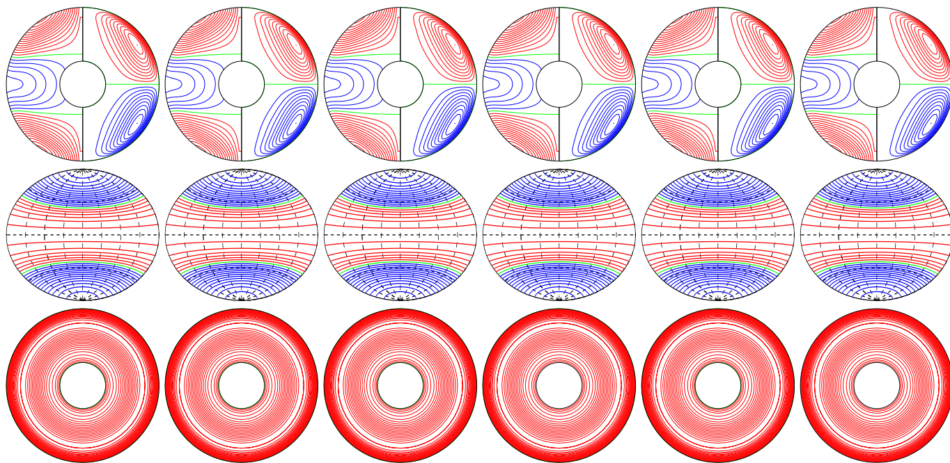
a.e03p1t03r-50000m16n2N2z1.0e2Y E_{\text{kin}}
