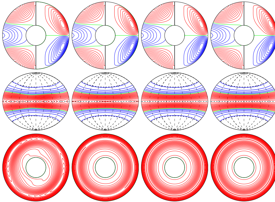
a.e03p1t03r-50000m1n2N2z4.5e4Ya E_{\text{kin}}
