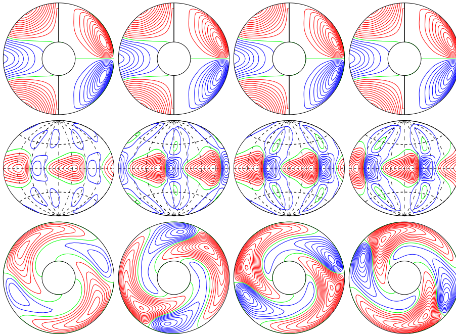
a.e03p1t03r-50000m1n2N2z4.68e4Yb E_{\text{kin}}
