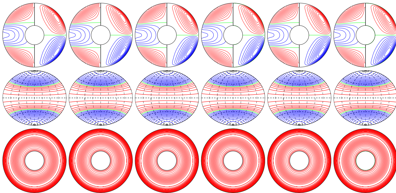
a.e03p1t03r-50000m16n2N2z1.0e0Y E_{\text{kin}}
