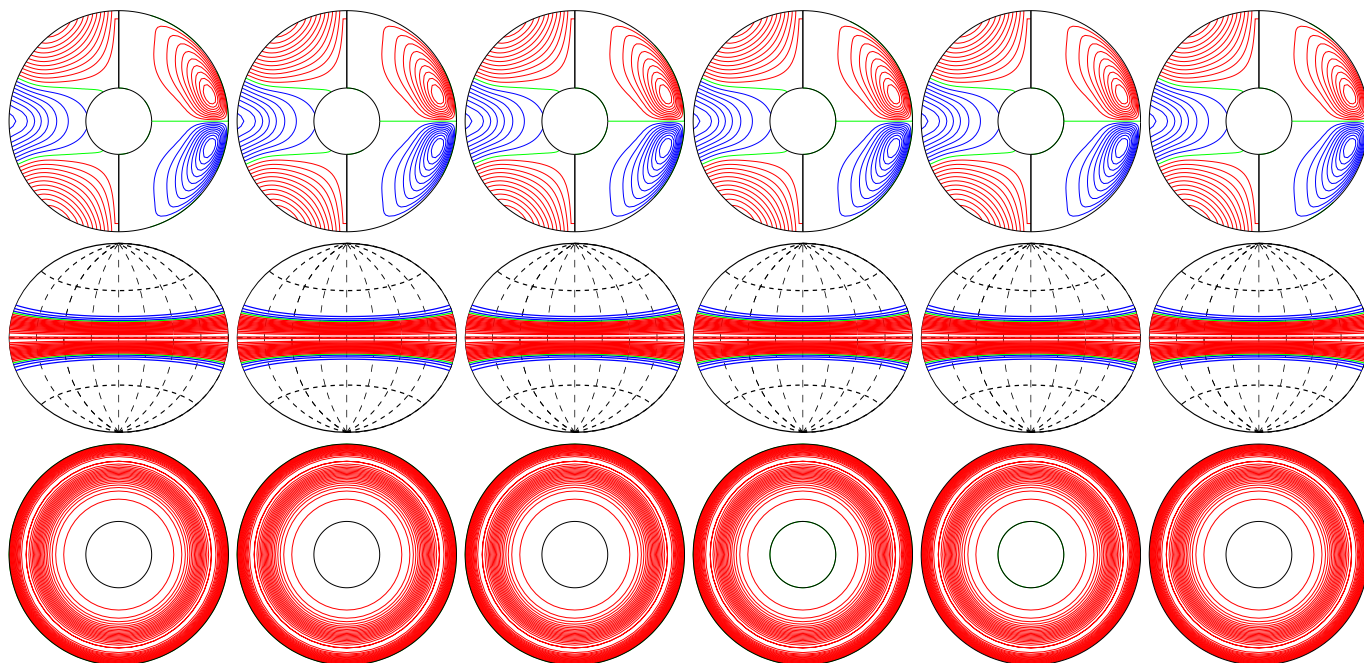
a.e03p1t03r-50000m16n2N2z6.0e4Y E_{\text{kin}}
