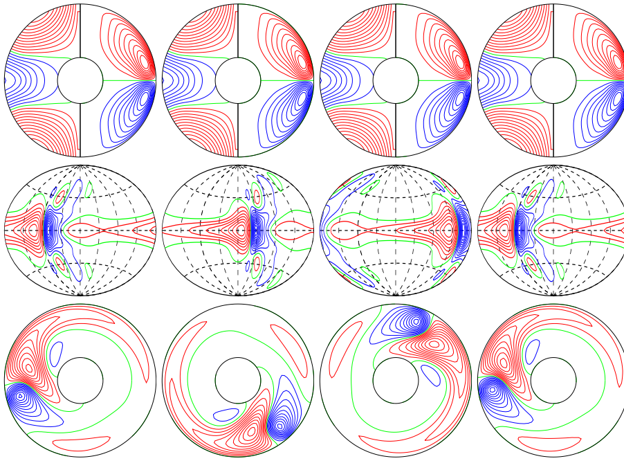
a.e03p1t03r-50000m1n2N2z5.2e4Ya E_{\text{kin}}
