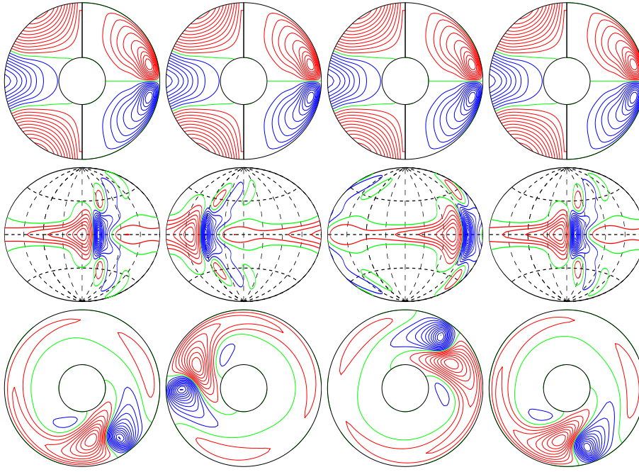
a.e03p1t03r-50000m1n2N2z5.4e4Ya E_{\text{kin}}
