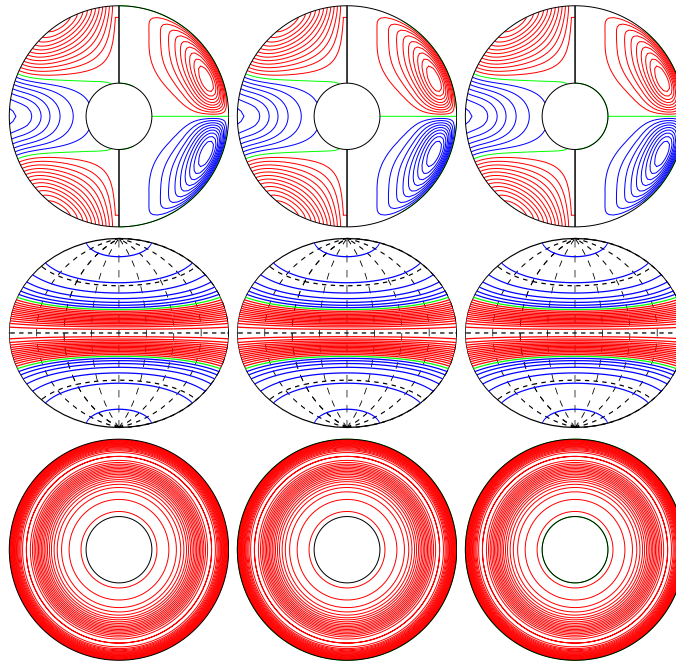
a.e03p1t03r-50000m1n2N2z4.4e4Y E_{\text{kin}}
