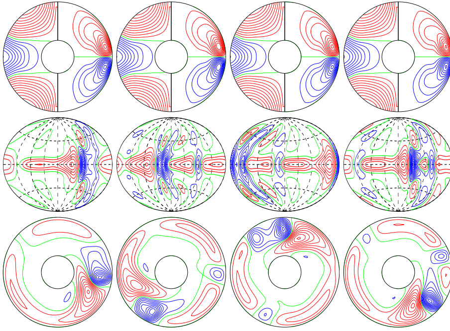
a.e03p1t03r-50000m1n2N2z5.6e4Ya E_{\text{kin}}
