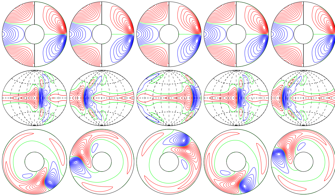
a.e03p1t03r-50000m1n2N2z5.4e4Ya E_{\text{kin}}
