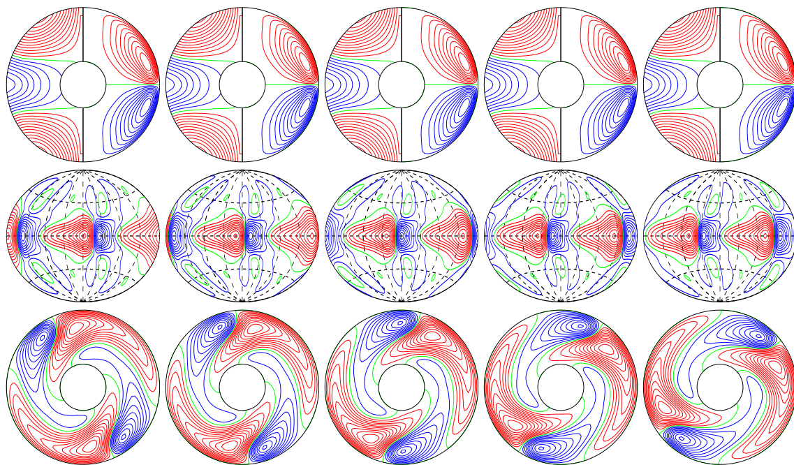
a.e03p1t03r-50000m1n2N2z4.7e4Ya E_{\text{kin}}
