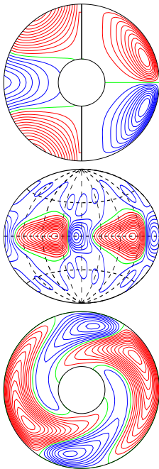
a.e03p1t03r-50000m1n2N2z4.64e4Yb E_{\text{kin}}
