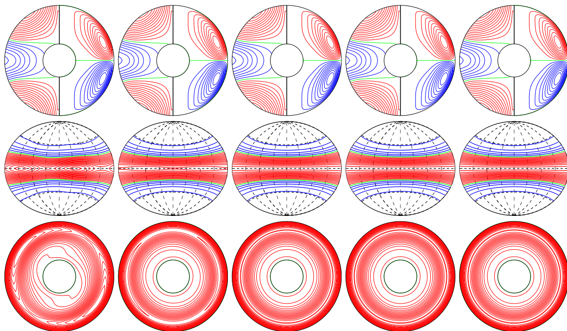
a.e03p1t03r-50000m1n2N2z4.5e4Ya E_{\text{kin}}
