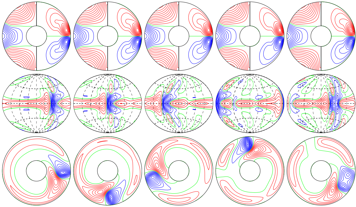
a.e03p1t03r-50000m1n2N2z5.8e4Ya E_{\text{kin}}
