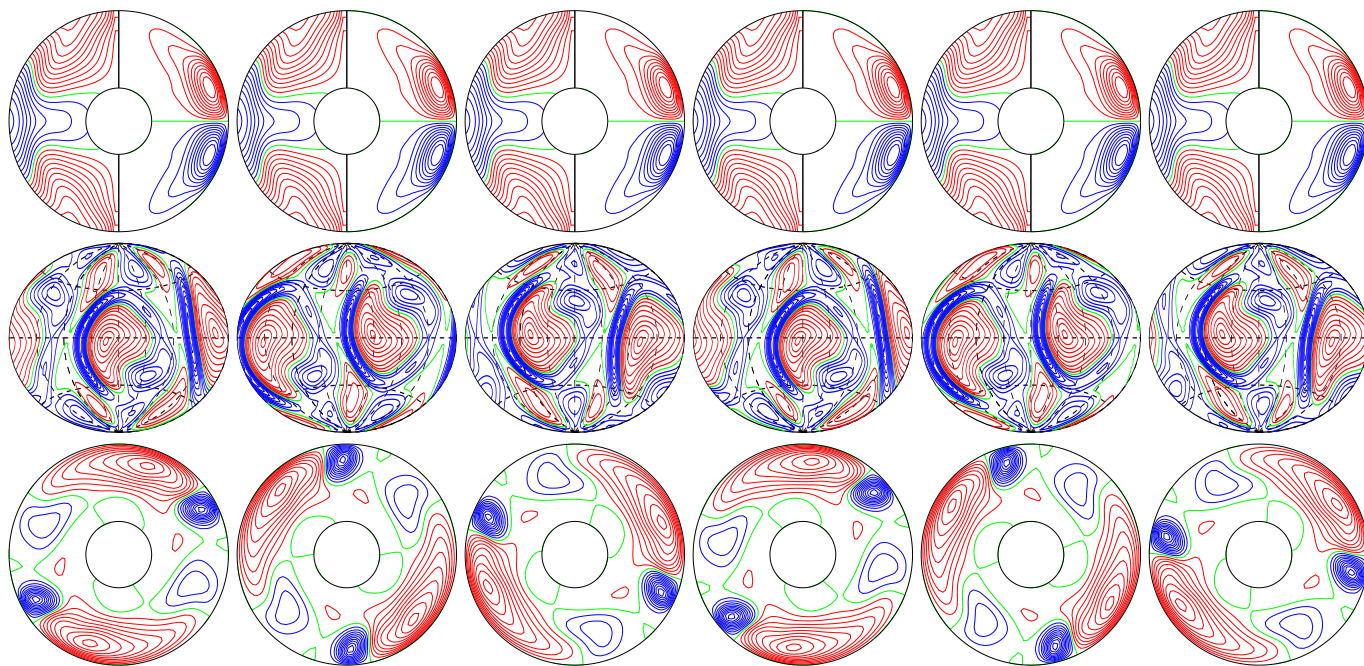
a.e03p1t03r-50000m1n2N2z9.0e4Y E_{\text{kin}}
