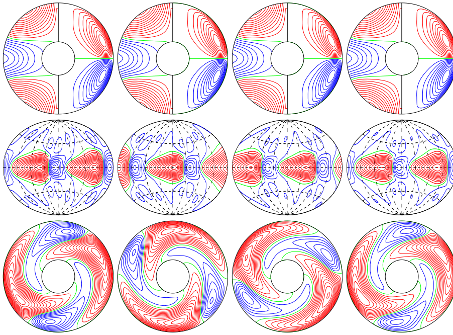
a.e03p1t03r-50000m1n2N2z4.64e4Yb E_{\text{kin}}
