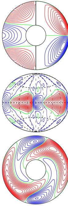
a.e03p1t03r-50000m1n2N2z4.66e4Yb E_{\text{kin}}
