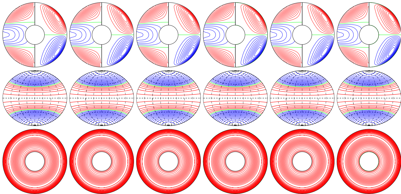
a.e03p1t03r-50000m16n2N2z1.0e0Y E_{\text{kin}}
