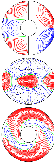
a.e03p1t03r-50000m1n2N2z4.615e4Yb E_{\text{kin}}
