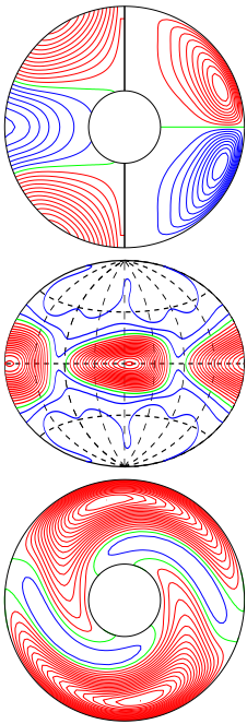
a.e03p1t03r-50000m1n2N2z4.61e4Yb E_{\text{kin}}
