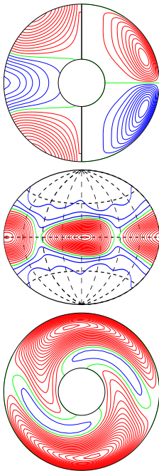
a.e03p1t03r-50000m1n2N2z4.605e4Yb E_{\text{kin}}
