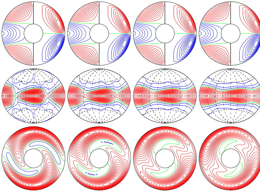
a.e03p1t03r-50000m1n2N2z4.61e4Yb E_{\text{kin}}
