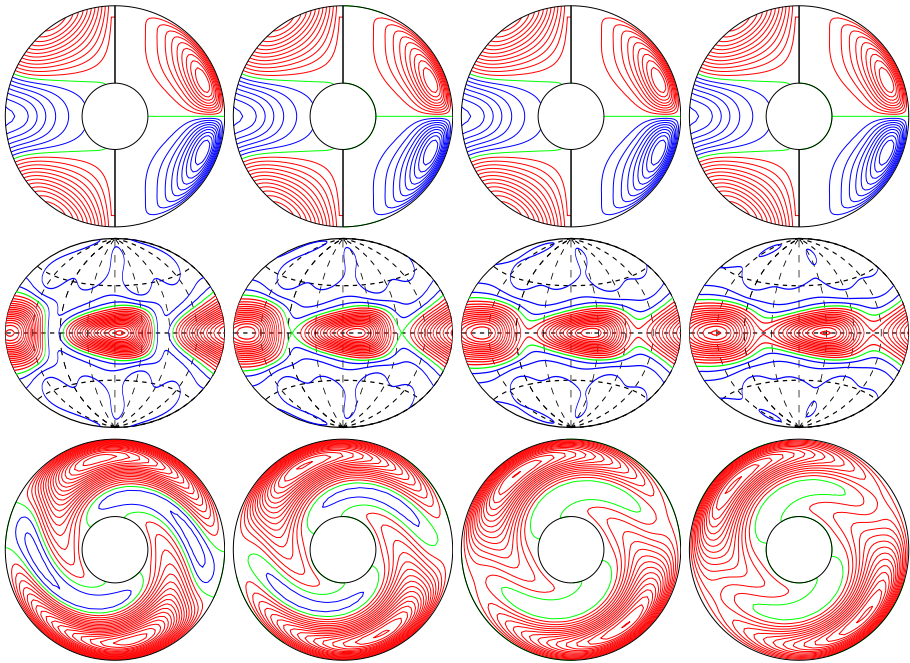
a.e03p1t03r-50000m1n2N2z4.615e4Yb E_{\text{kin}}
