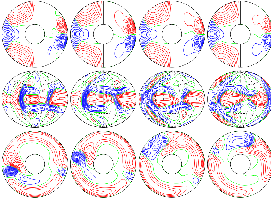
a.e03p1t03r-50000m1n2N2z6.8e4Ya E_{\text{kin}}
