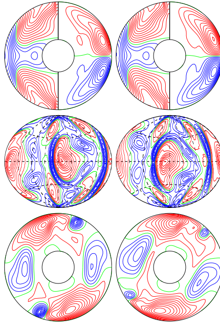
a.e03p1t03r-50000m1n2N2z1.1e5Ya E_{\text{kin}}
