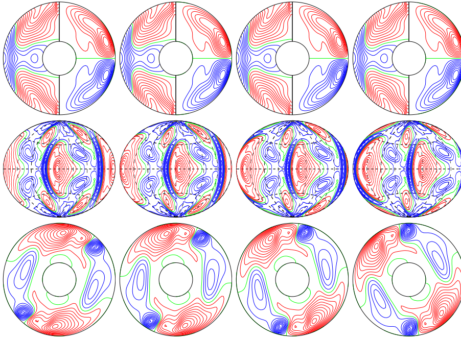
a.e03p1t03r-50000m1n2N2z1.1e5Yb E_{\text{kin}}
