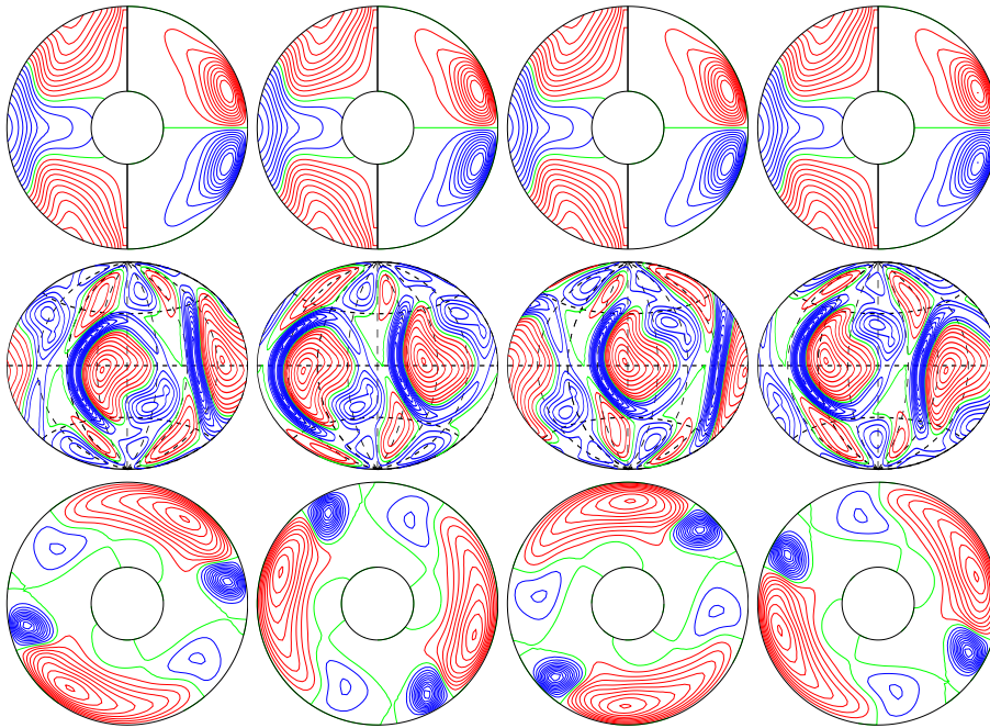
a.e03p1t03r-50000m1n2N2z8.8e4Ya E_{\text{kin}}
