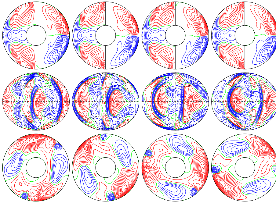
a.e03p1t03r-50000m1n2N2z1.15e5Ya E_{\text{kin}}
