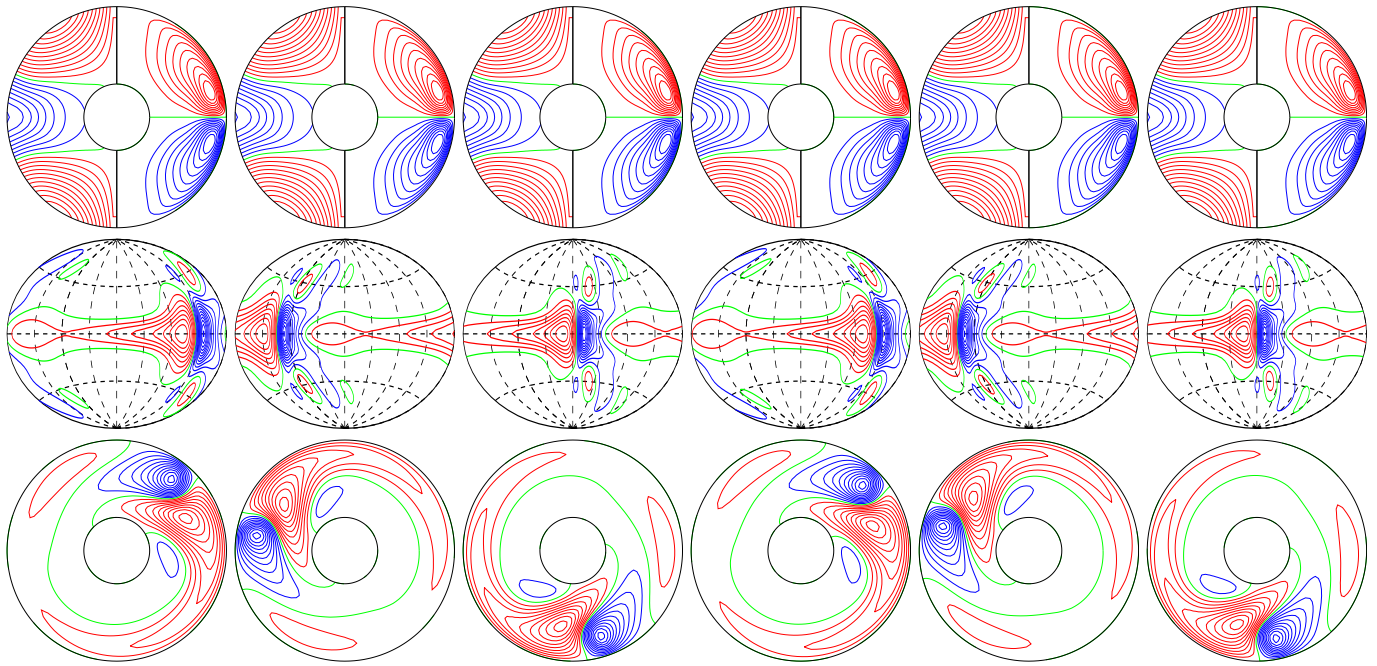
a.e03p1t03r-50000m1n2N2z5.2e4Ya E_{\text{kin}}
