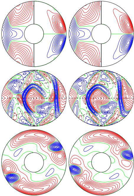
a.e03p1t03r-50000m1n2N2z8.4e4Ya E_{\text{kin}}
