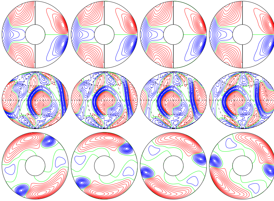
a.e03p1t03r-50000m1n2N2z8.6e4Ya E_{\text{kin}}
