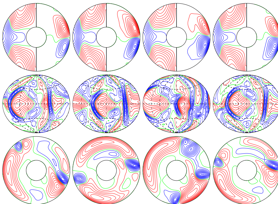
a.e03p1t03r-50000m1n2N2z8.4e4Yb E_{\text{kin}}
