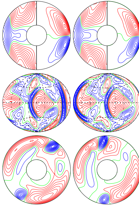
a.e03p1t03r-50000m1n2N2z8.8e4Yb E_{\text{kin}}
