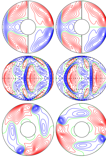
a.e03p1t03r-50000m1n2N2z1.2e5Yb E_{\text{kin}}
