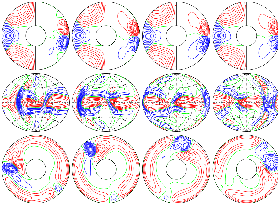
a.e03p1t03r-50000m1n2N2z6.6e4Ya E_{\text{kin}}
