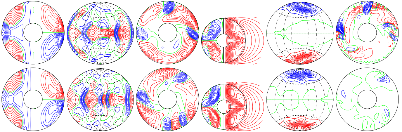
a.e03p1t03r-50000m1p6n2N2z8.0e4Ya E_{\text{kin}}
