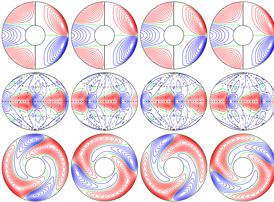
a.e03p1t03r-50000m1n2N2z4.66e4Yb E_{\text{kin}}
