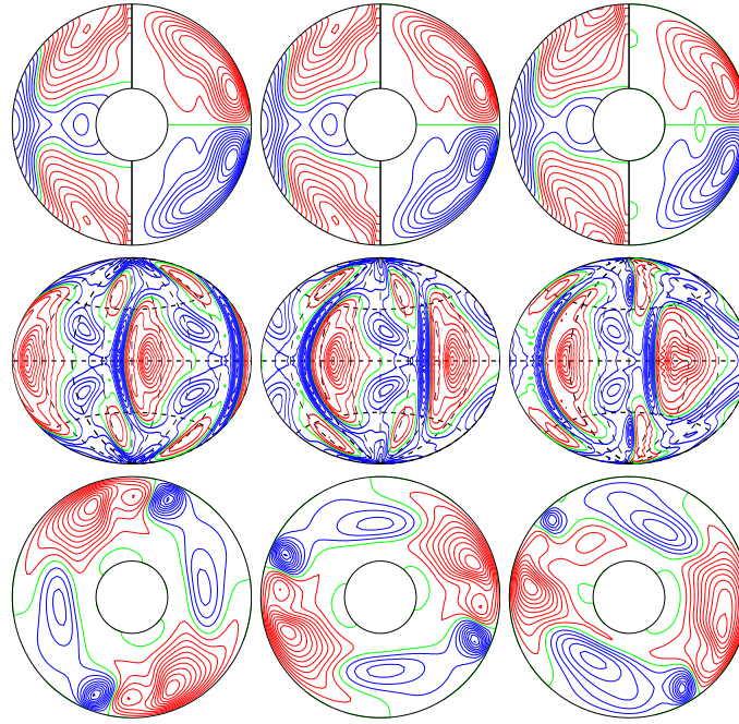
a.e03p1t03r-50000m1n2N2z1.2e5Yb E_{\text{kin}}
