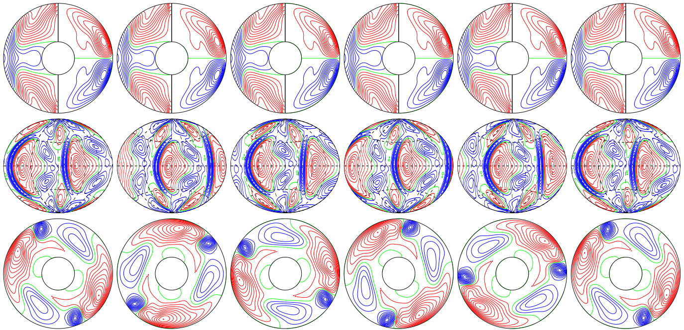
a.e03p1t03r-50000m1n2N2z1.0e5Y E_{\text{kin}}
