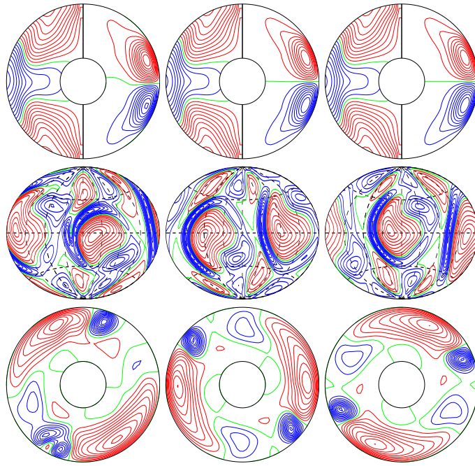
a.e03p1t03r-50000m1n2N2z9.0e4Ybb E_{\text{kin}}
