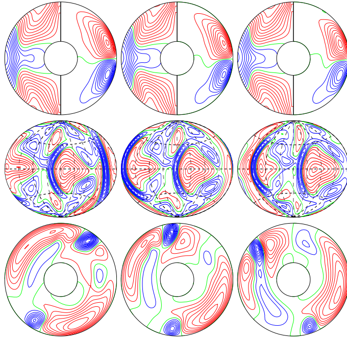
a.e03p1t03r-50000m1n2N2z8.8e4Yb E_{\text{kin}}
