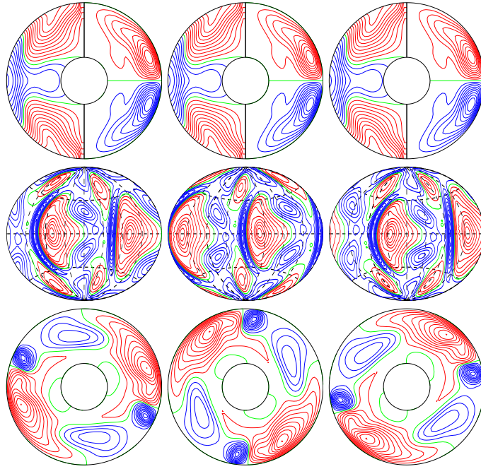
a.e03p1t03r-50000m1n2N2z1.0e5Yaa E_{\text{kin}}
