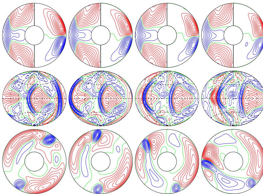
a.e03p1t03r-50000m1n2N2z8.8e4Yb E_{\text{kin}}
