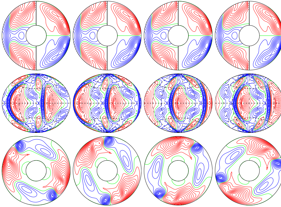
a.e03p1t03r-50000m1n2N2z1.15e5Yb E_{\text{kin}}
