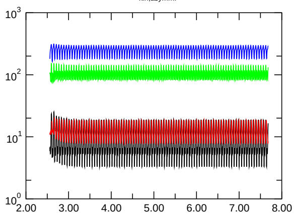
E_{kin,asymm.}
