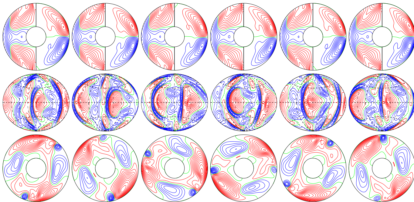
a.e03p1t03r-50000m1n2N2z1.15e5Ya E_{\text{kin}}
