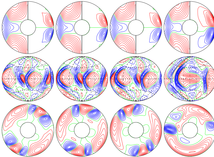
a.e03p1t03r-50000m1n2N2z8.2e4Ya E_{\text{kin}}
