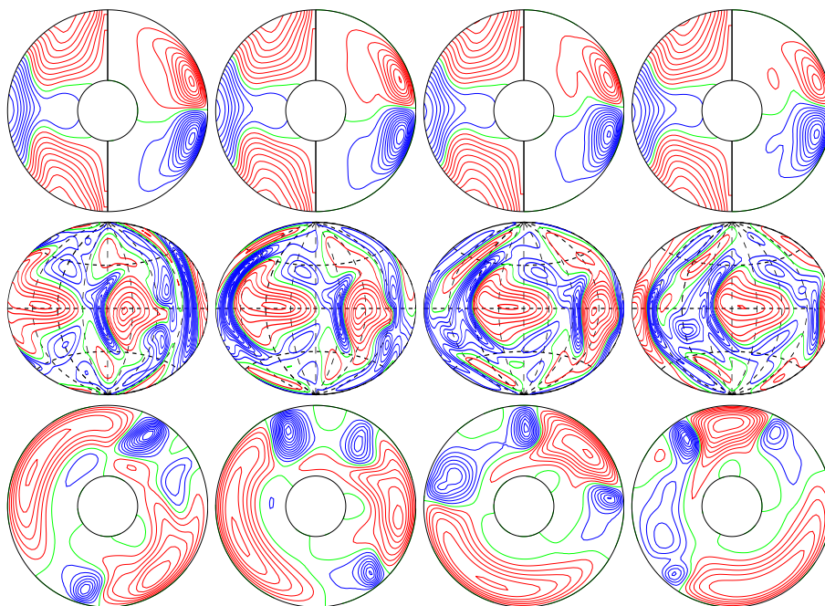
a.e03p1t03r-50000m1n2N2z8.6e4Yb E_{kin}
