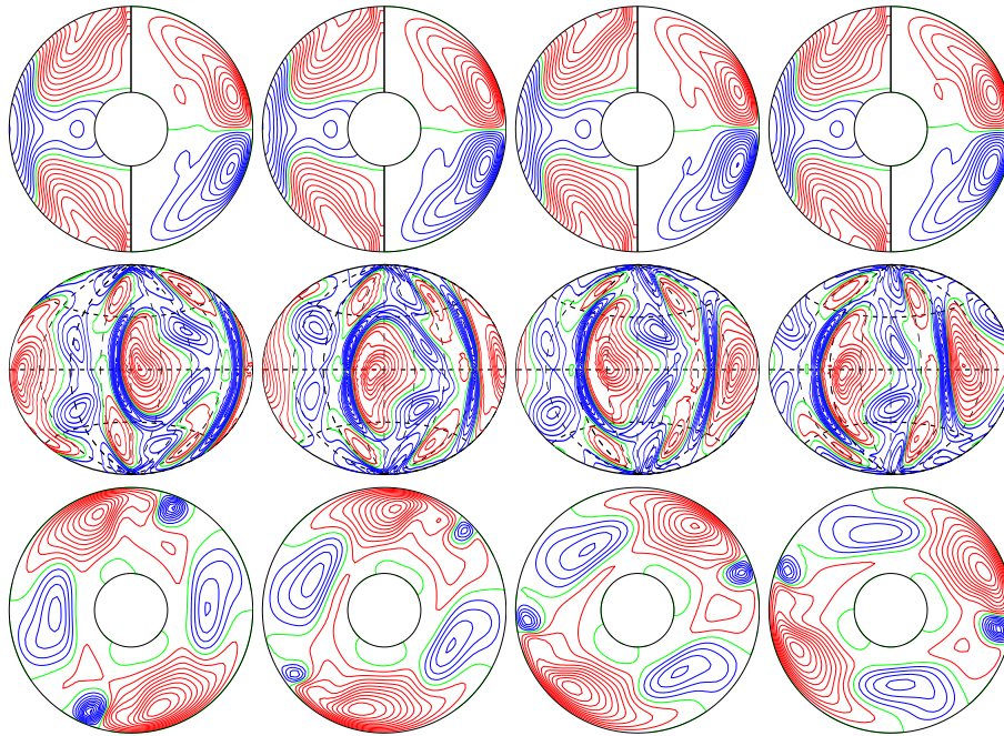
a.e03p1t03r-50000m1n2N2z1.1e5Ya E_{\text{kin}}
