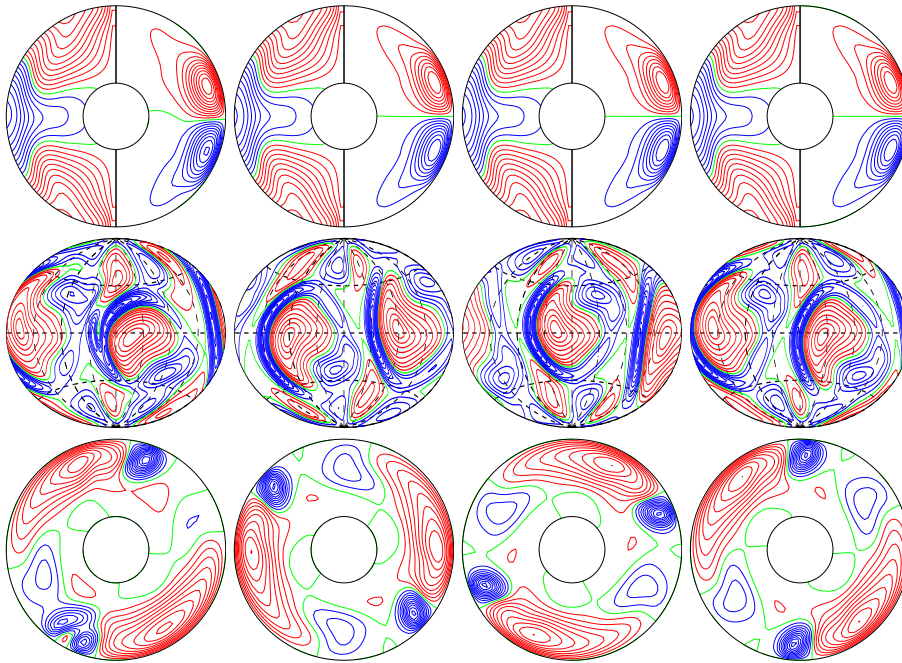
a.e03p1t03r-50000m1n2N2z9.0e4Ybb E_{\text{kin}}
