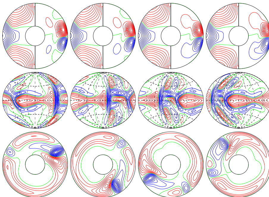
a.e03p1t03r-50000m1n2N2z6.4e4Ya E_{\text{kin}}
