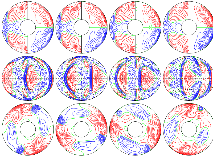
a.e03p1t03r-50000m1n2N2z1.2e5Yb E_{\text{kin}}
