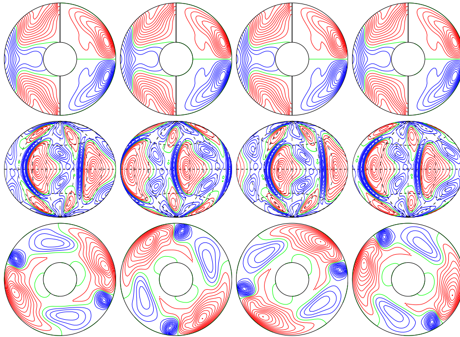
a.e03p1t03r-50000m1n2N2z1.0e5Yaa E_{\text{kin}}
