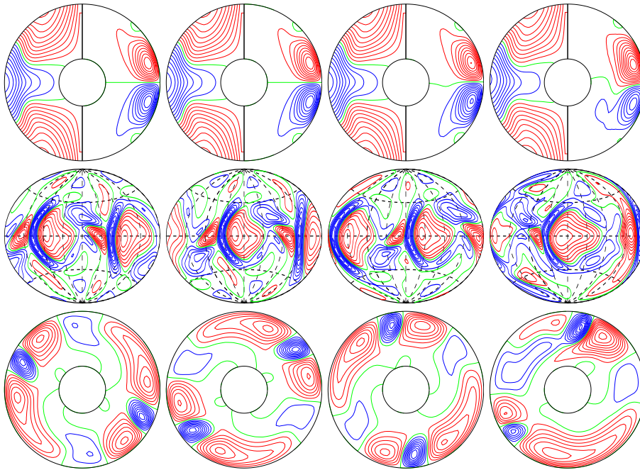
a.e03p1t03r-50000m1n2N2z8.0e4Yaa E_{\text{kin}}
