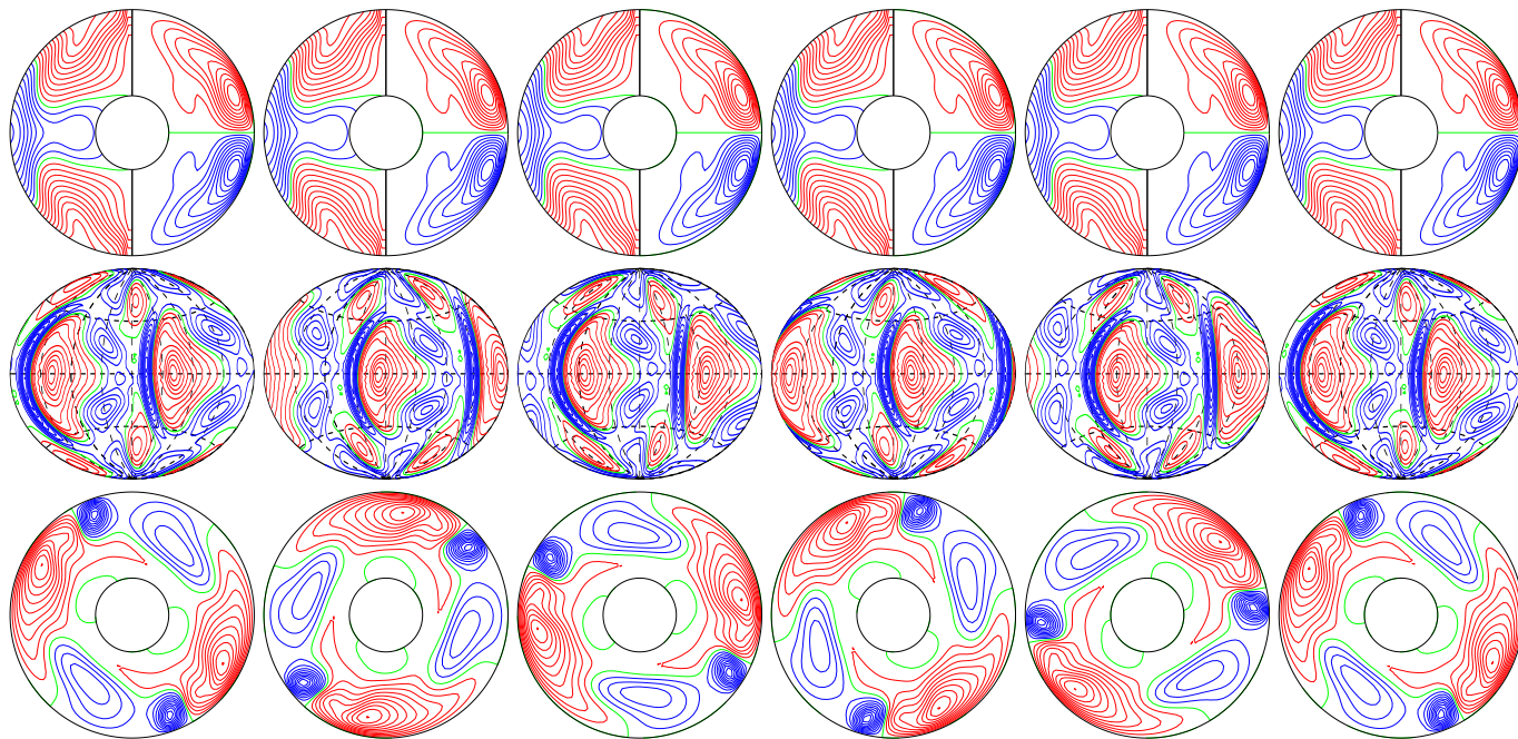
a.e03p1t03r-50000m1n2N2z1.0e5Y E_{\text{kin}}
