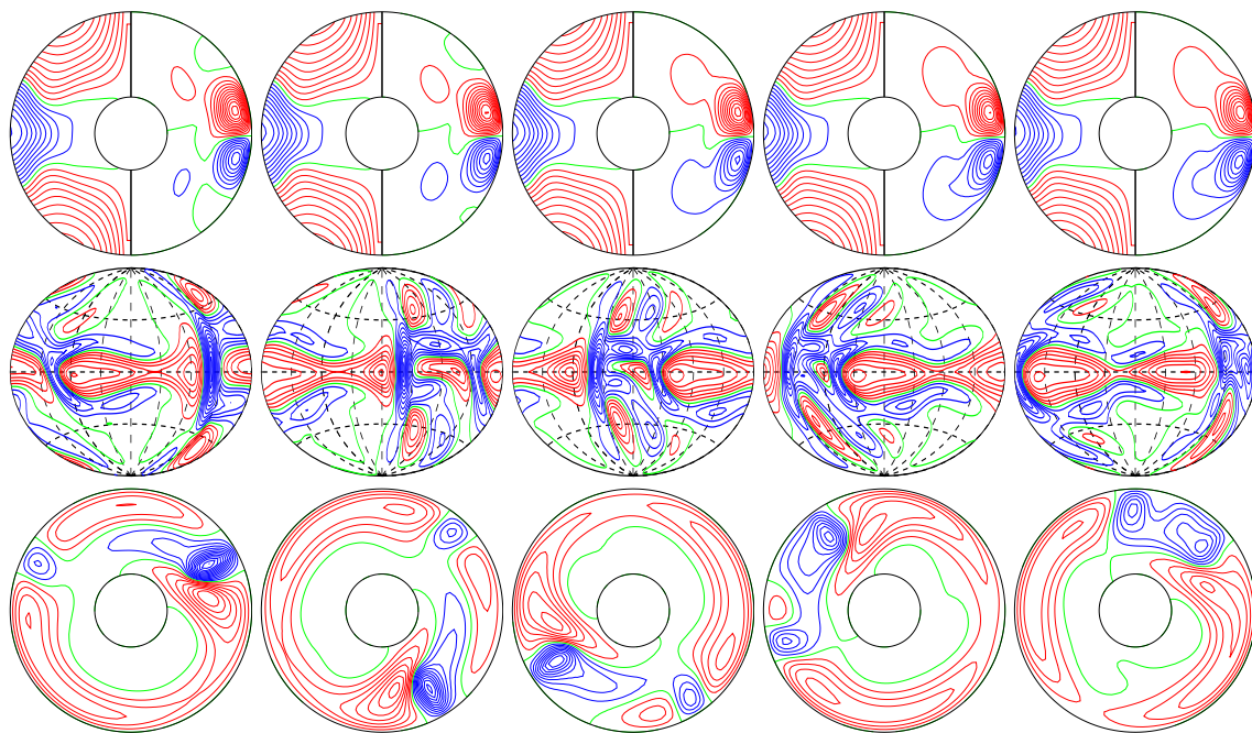
a.e03p1t03r-50000m1n2N2z6.4e4Ya E_{\text{kin}}
