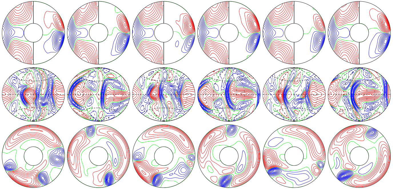
a.e03p1t03r-50000m1n2N2z8.2e4Yb E_{\text{kin}}
