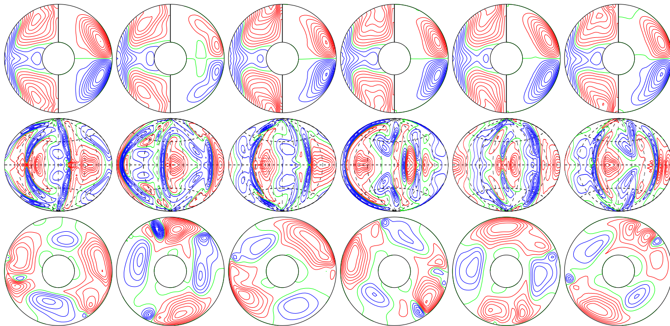
a.e03p1t03r-50000m1n2N2z1.3e5Y E_{\text{kin}}
