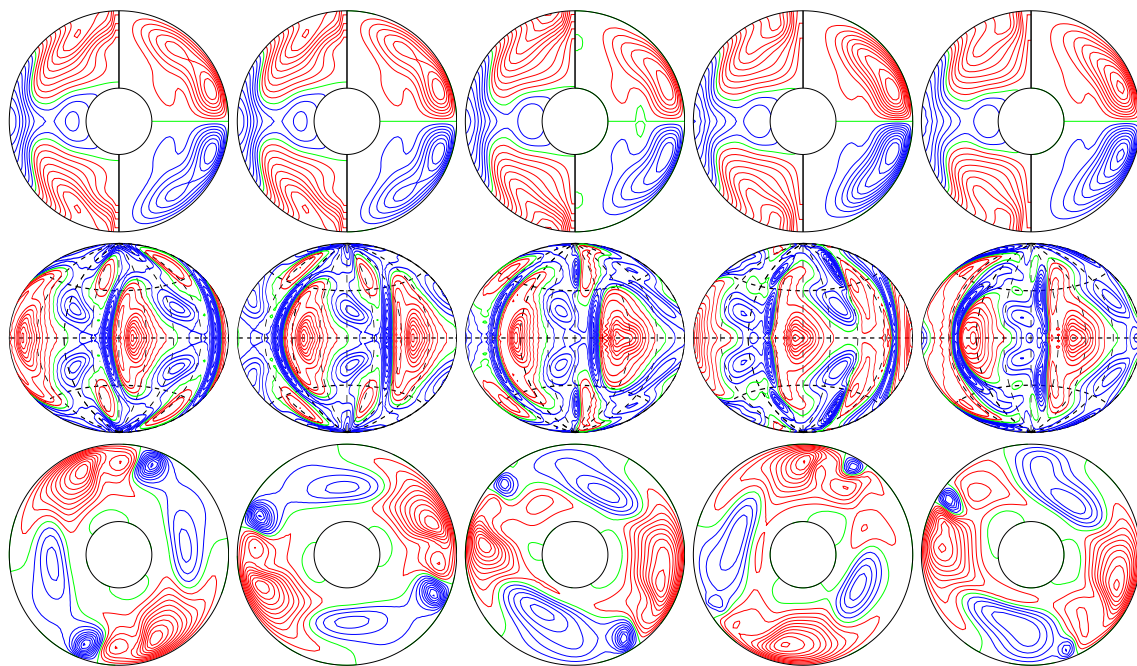
a.e03p1t03r-50000m1n2N2z1.2e5Yb E_{\text{kin}}
