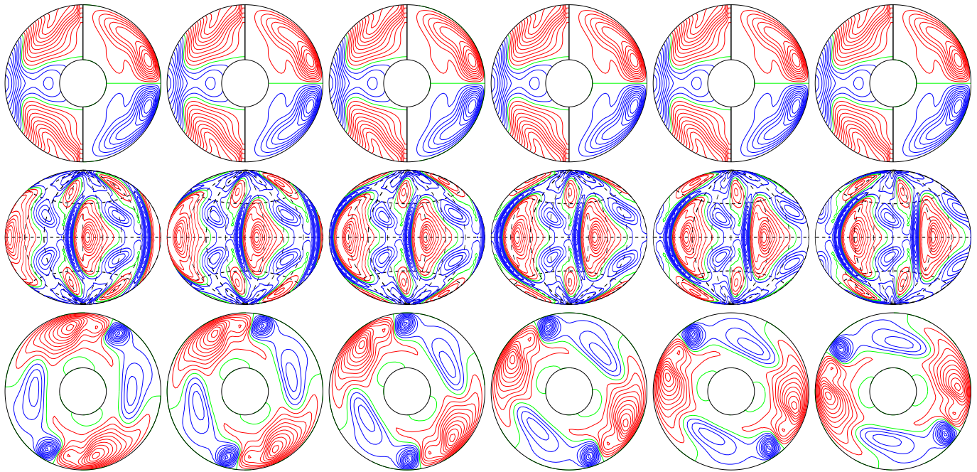
a.e03p1t03r-50000m1n2N2z1.1e5Yb E_{\text{kin}}
