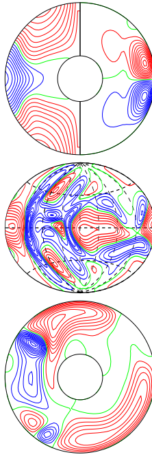
a.e03p1t03r-50000m1n2N2z7.25e4Yb E_{\text{kin}}
