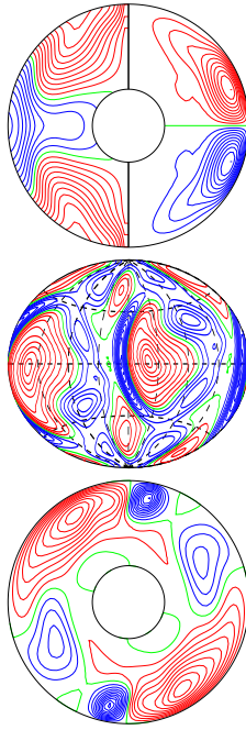
a.e03p1t03r-50000m1n2N2z9.5e4Yb E_{\text{kin}}
