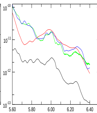
E_{\text{magn, quadr.}}
