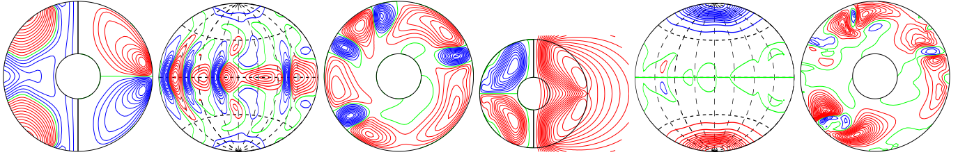
a.e03p1t03r-50000m1p7n2N2z6.5e4Ya E_{kin}
