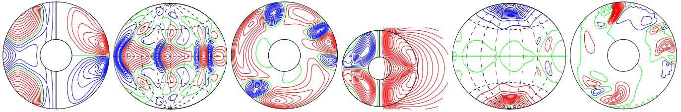
a.e03p1t03r-50000m1p6n2N2z7.0e4Ya E_{\text{kin}}
