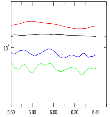
E_{\text{magn, dip.}}
