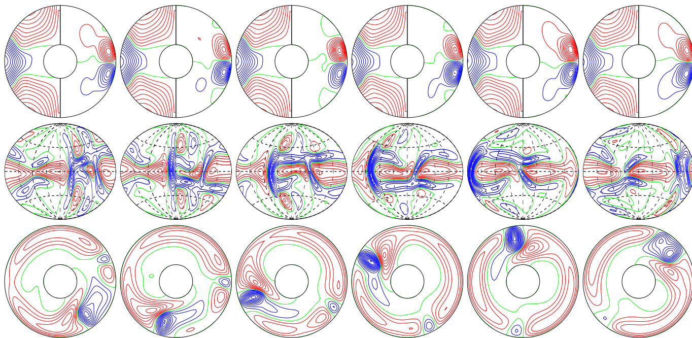
a.e03p1t03r-50000m1n2N2z6.6e4Ya E_{\text{kin}}
