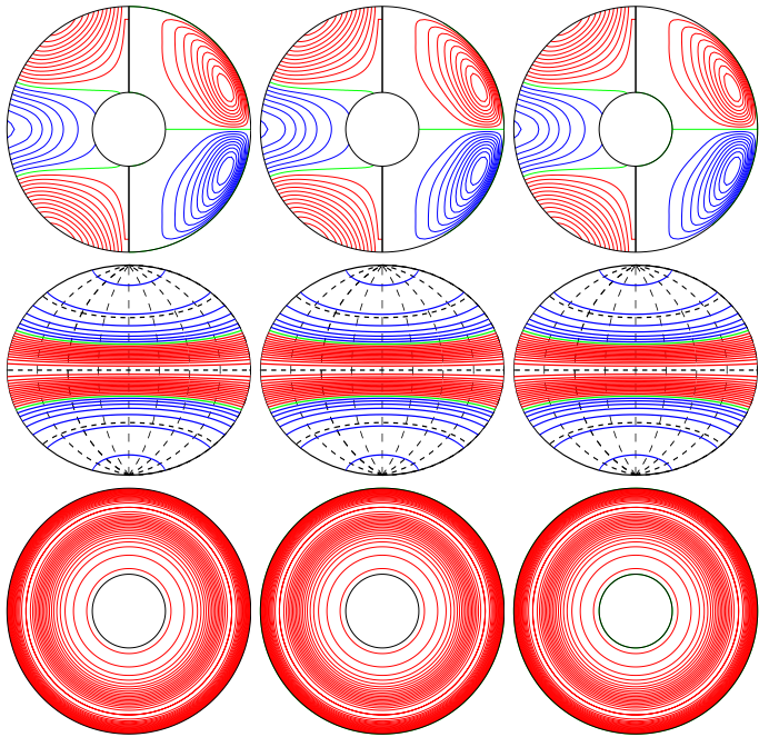
a.e03p1t03r-50000m1n2N2z4.4e4Y E_{\text{kin}}
