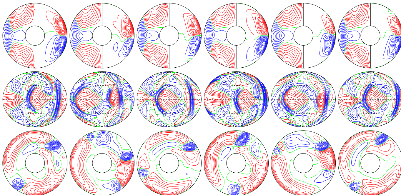
a.e03p1t03r-50000m1n2N2z8.4e4Yb E_{\text{kin}}
