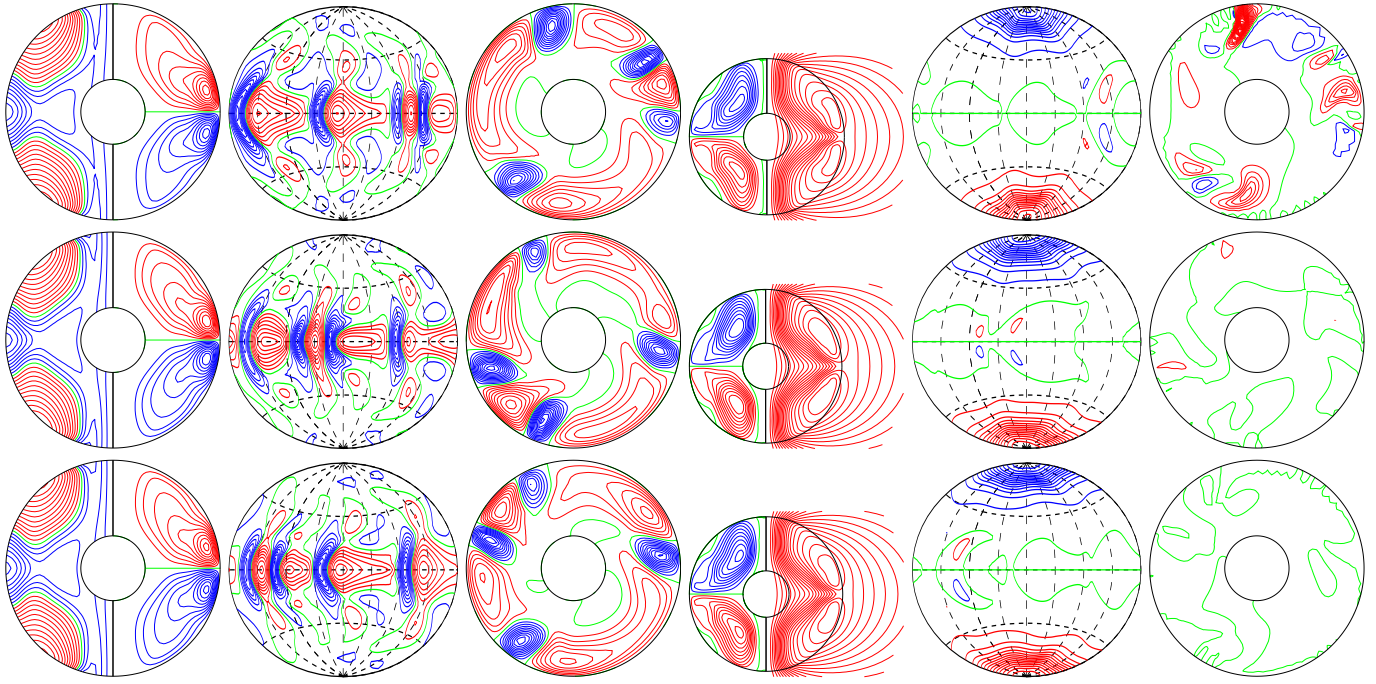
a.e03p1t03r-50000m1p6n2N2z7.0e4Ya E_{kin}
