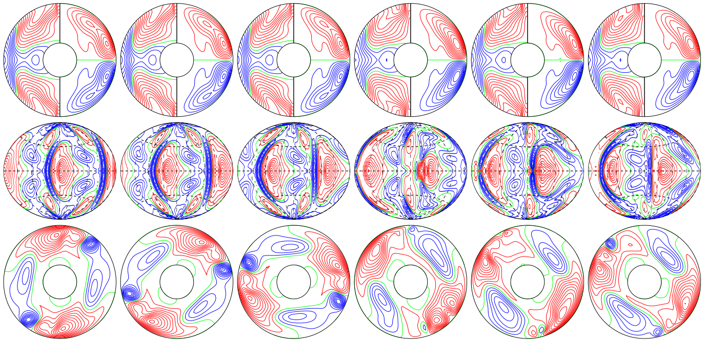
a.e03p1t03r-50000m1n2N2z1.15e5Yb E_{\text{kin}}
