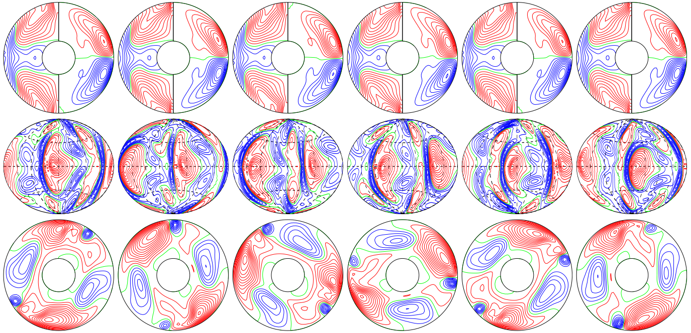
a.e03p1t03r-50000m1n2N2z1.15e5Ya E_{\text{kin}}
