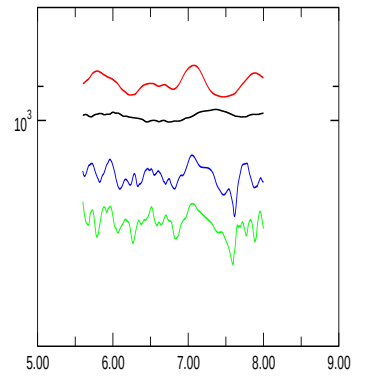
E_{magn,dip.}
