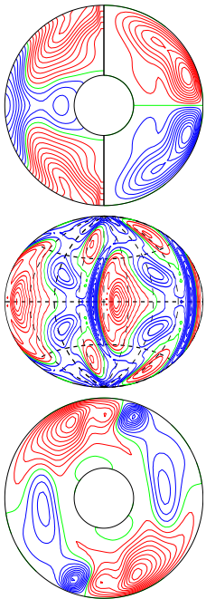
a.e03p1t03r-50000m1n2N2z1.14e5YbB E_{\text{kin}}
