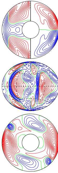
a.e03p1t03r-50000m1n2N2z1.08e5YaA E_{\text{kin}}
