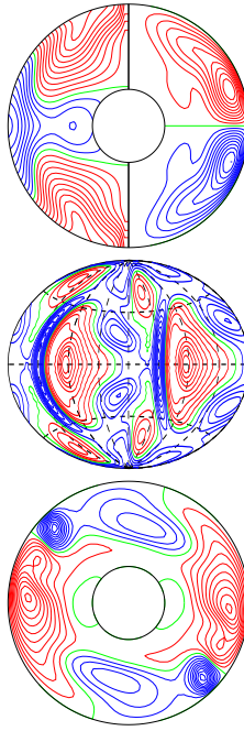
a.e03p1t03r-50000m1n2N2z1.04e5YaA E_{\text{kin}}
