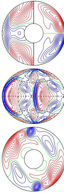
a.e03p1t03r-50000m1n2N2z1.06e5YaA E_{\text{kin}}
