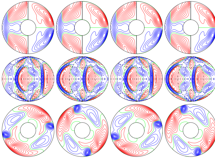
a.e03p1t03r-50000m1n2N2z1.02e5YbA E_{\text{kin}}
