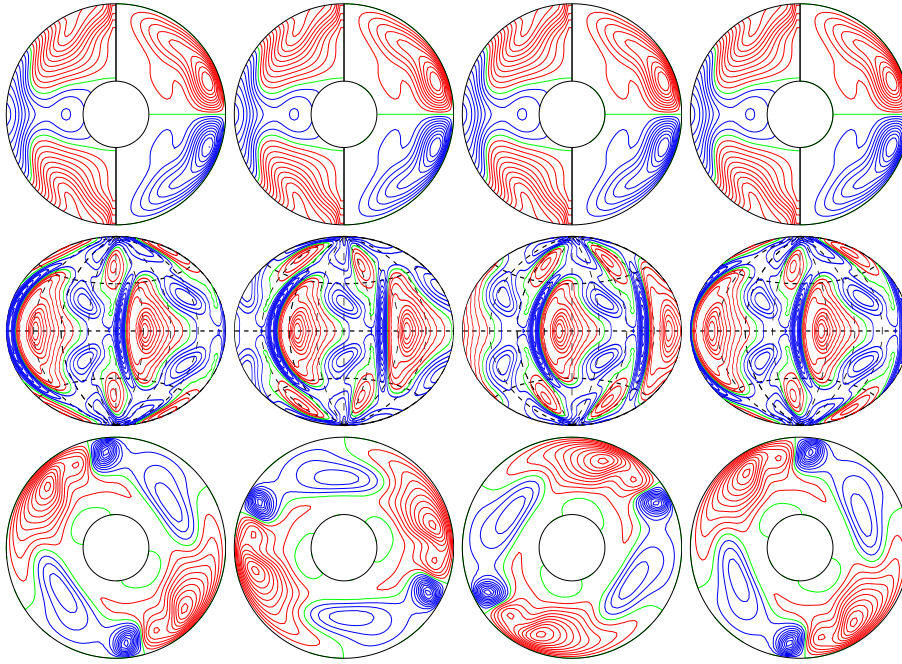
a.e03p1t03r-50000m1n2N2z1.06e5YaA E_{\text{kin}}
