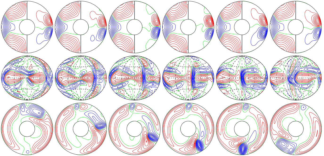
a.e03p1t03r-50000m1n2N2z6.8e4Ya E_{\text{kin}}
