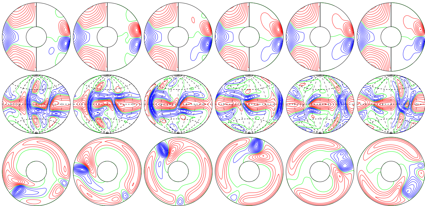
a.e03p1t03r-50000m1n2N2z6.6e4Ya E_{\text{kin}}
