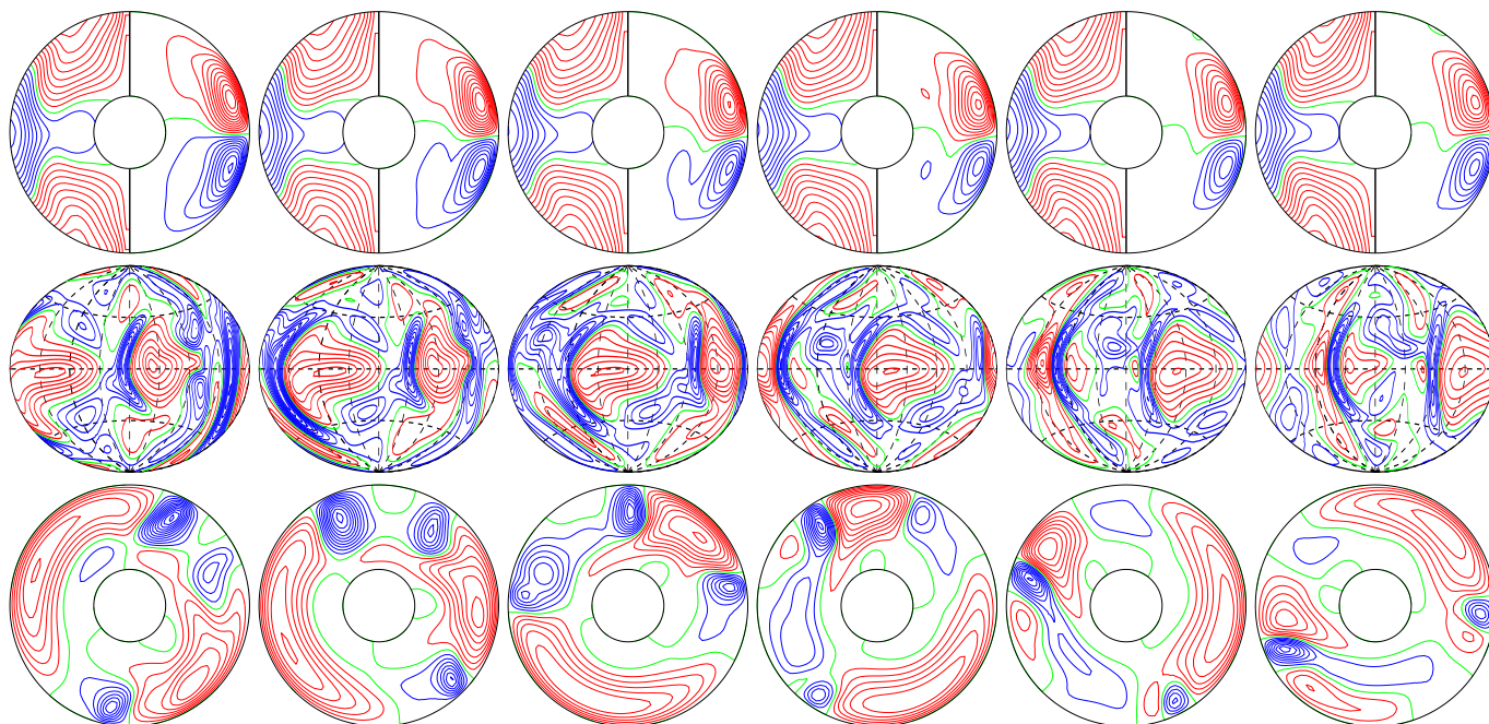
a.e03p1t03r-50000m1n2N2z8.6e4Yb E_{\text{kin}}
