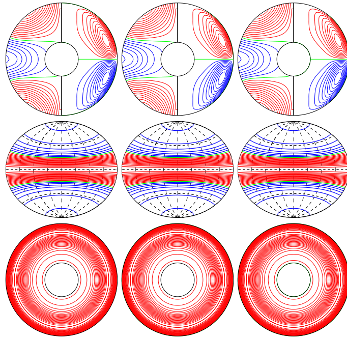
a.e03p1t03r-50000m1n2N2z4.4e4Y E_{\text{kin}}
