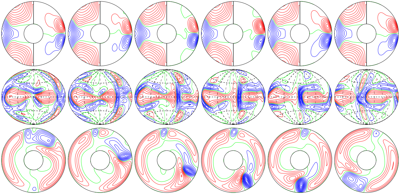
a.e03p1t03r-50000m1n2N2z6.8e4Ya E_{\text{kin}}
