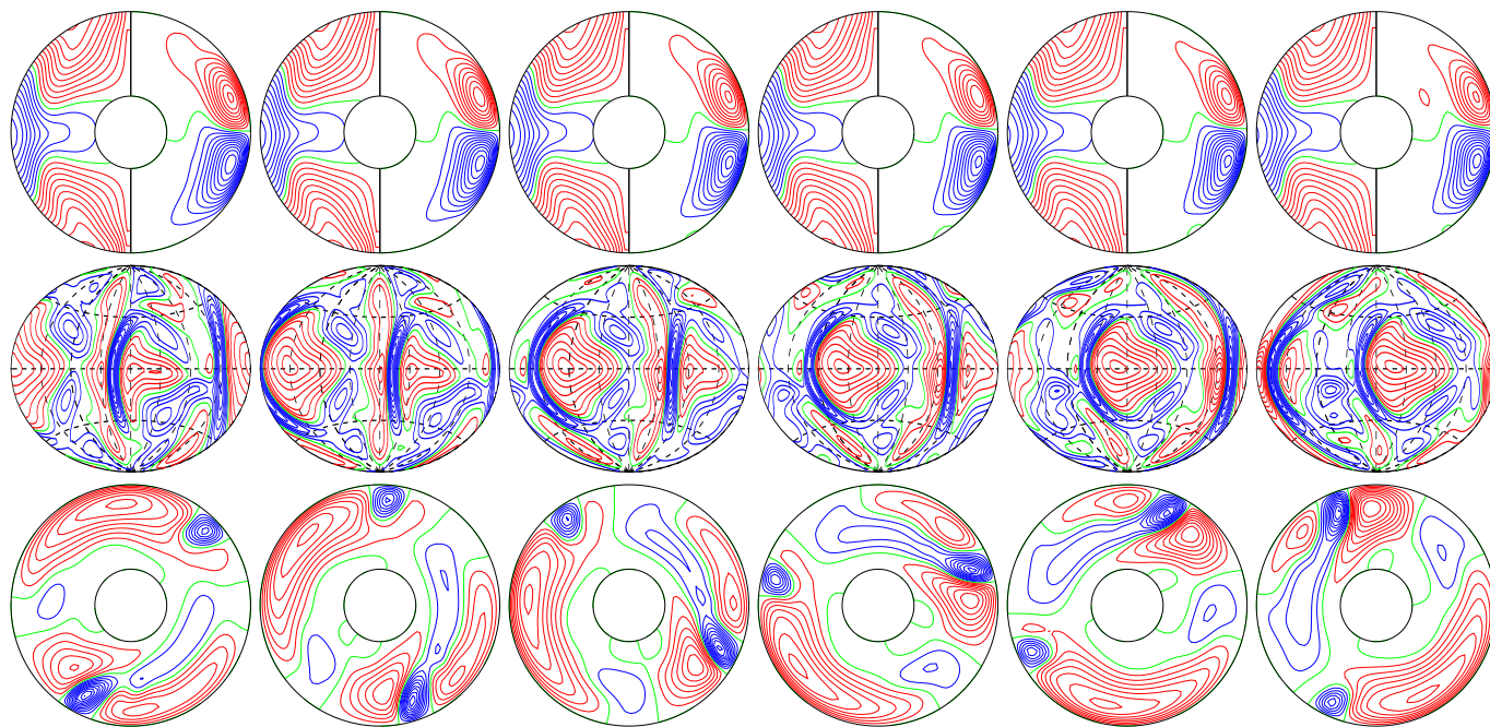
a.e03p1t03r-50000m1n2N2z8.7e4Yb E_{\text{kin}}
