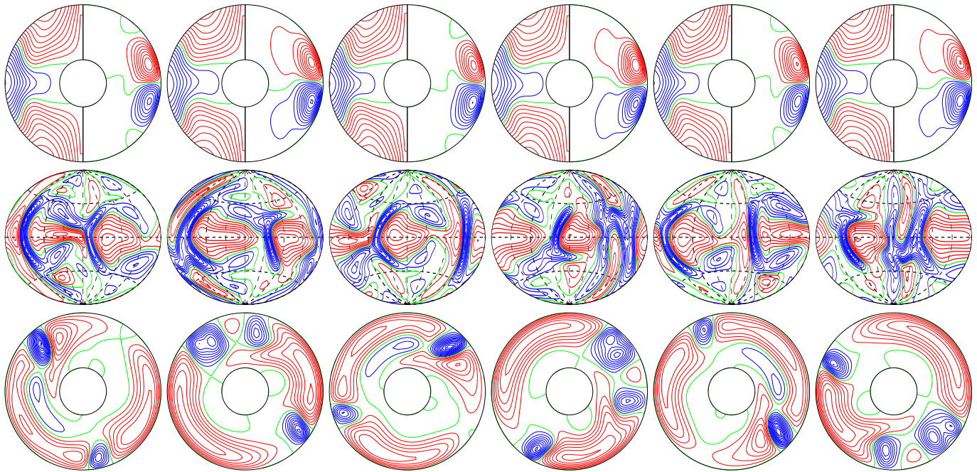
a.e03p1t03r-50000m1n2N2z7.75e4Ya E_{\text{kin}}
