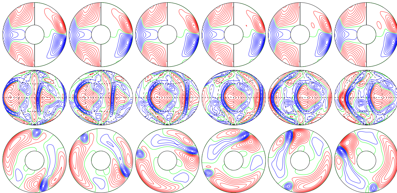
a.e03p1t03r-50000m1n2N2z8.7e4Yb E_{\text{kin}}
