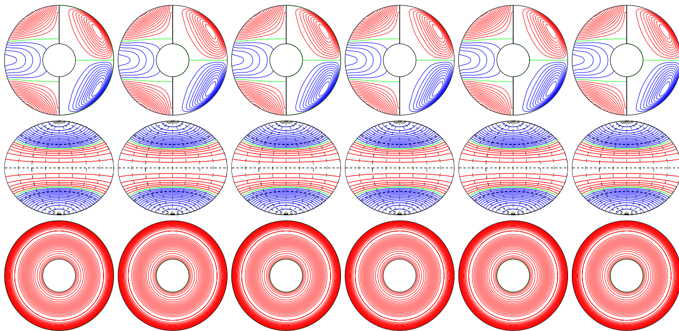
a.e03p1t03r-50000m16n2N2z1.0e3Y E_{\text{kin}}
