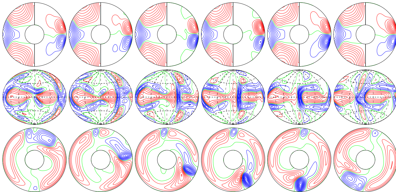
a.e03p1t03r-50000m1n2N2z6.8e4Ya E_{\text{kin}}
