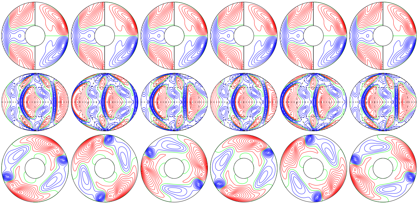
a.e03p1t03r-50000m1n2N2z1.05e5YaA E_{\text{kin}}
